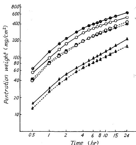
Fig. 4 AKAMATSU sapwood
