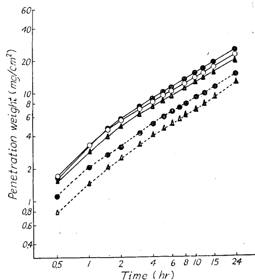
Fig. 2 SUGI heartwood
