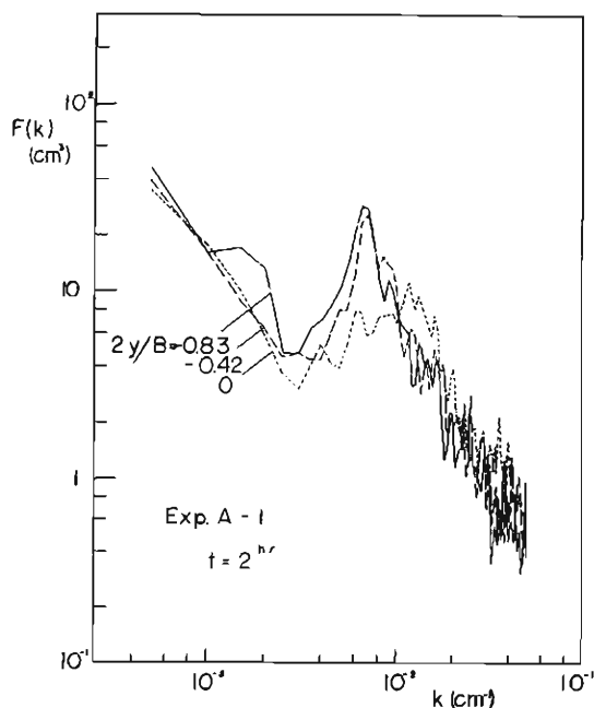
Fig. 2. Lateral variation of power spectral density of bed configuration along the longitudinal line, after 2 hr. in Exp. A-1.
