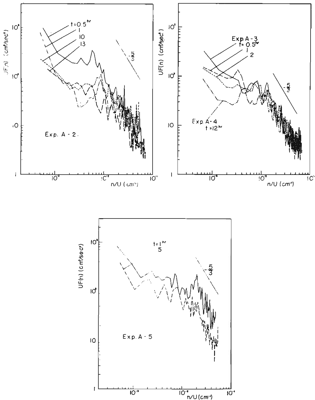
Fig. 7 Variations of energy spectra of the longitudinal velocity with time on the movable bed in flume A, at 2y/B = -0.57 , z = (h-2)\text{cm} .
