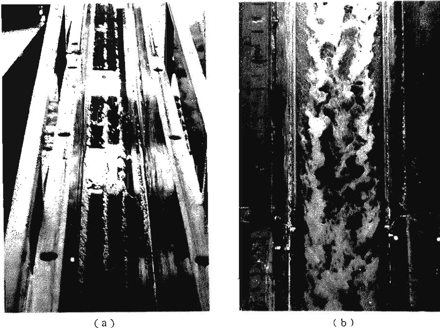
Photo. 3 Longitudinal streakings in Exp. B-4. (a) Bed configuration to up stream after 2 hr. (b) Surface flow pattern with aluminum powder to up stream.
