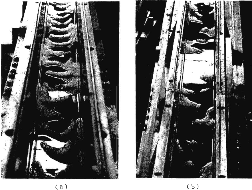
Photo. 2 Bed configuration to up stream in flume B.
