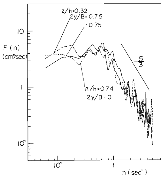
Fig. 6 Energy spectra of the longitudinal velocity on the steel bed in flume B, U = 70.6 \text{ cm/s} , h = 4.75 \text{ cm} , i = 1/200 .
