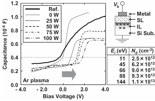
Fig. 2. Capacitance–voltage curves of metal/SL/IL/Si structure obtained by a mercury probe for various bias powers P_{RF} . The table lists the average ion energy E_i (= q(V_p - V_{dc})) and the calculated areal density of defect site ( N_d ).
