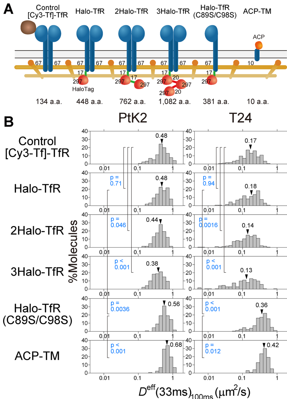
FIGURE 7: TFR's D^{\text{eff}}(33\text{ ms})_{100\text{ ms}} (and thus hop frequency) depends on both its cytoplasmic domain size and dimerization in both PtK2 and T24 cells. (A) Molecules used for this examination. Note that endogenous TFR exists as dimers, and that since the expression levels of modified TFR molecules are much smaller than that of endogenous TFR, most of the expressed molecules are expected to form dimers with endogenous TFR. The numbers indicate the number of amino acids in the cytoplasmic domain of the endogenous human TFR (67 aa), the Halo-tag protein (297 aa), linkers (17 and 20 aa), and the cytoplasmic domain of the ACP-TM (10 aa). The expected total numbers of amino acids in the cytoplasmic domain are shown below (the endogenous TFR in PtK2 cells was assumed to have the same number of amino acids in the cytoplasmic domain as that in human TFR). (B) Distributions of the effective macroscopic diffusion coefficient D^{\text{eff}}(33\text{ ms})_{100\text{ ms}} for the individual molecules in A in PtK2- and T24-cell PMs. D^{\text{eff}}(33\text{ ms})_{100\text{ ms}} should be proportional to the hop frequency. For a discussion of the effect of the cross section of a diffusant on its hop characteristics, see Supplemental Notes to Figure 7B.
