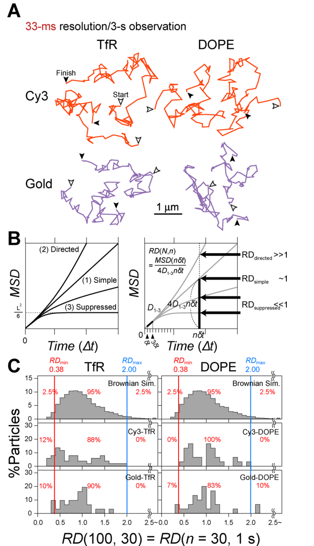
FIGURE 2: Method for classifying the trajectories into simple-Brownian-, suppressed-, and directed-diffusion modes and its application to TfR and DOPE trajectories (with fluorescent and gold probes) obtained in the PtK2-PM at video rate. (A) Representative trajectories of TfR (left) and DOPE (right) tagged with Cy3 (top) or gold (bottom) probes in the PtK2-PM. (B) Left, theoretical MSD- \Delta t curves for 1) simple-Brownian, 2) directed, and 3) suppressed diffusion (for the same short-term diffusion coefficients = initial slope at time 0). Right, motional mode classification based on RD(N, n) . (C) Distribution of RD(N, n) for N = 100 and n = 30 (1 s), used for the classification of the trajectories into different diffusion modes (left, TfR; right, DOPE). Top, simple-Brownian trajectories generated by Monte Carlo simulation (the same graphs are used for both TfR and DOPE). The 2.5th percentiles of the distribution from both ends, RD_{min}(100, 30) and RD_{MAX}(100, 30) , are shown by red and cyan vertical lines, respectively. Middle, SFMT at normal video rate, using Cy3 as a probe. Bottom, SPT at normal video rate, using gold particles as probes.
