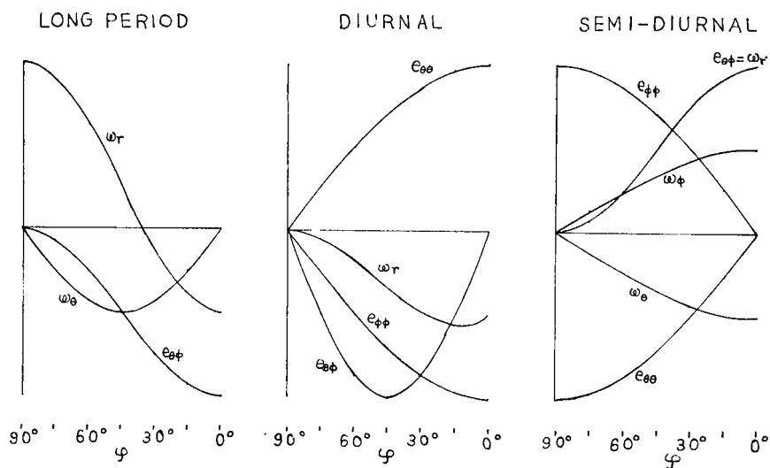
Fig. 5. The components of the strain of the torsional type deformation versus the latitude \varphi . The radial displacement and the cubical dilatation are nil.
