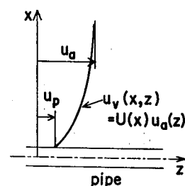
Fig. 6 Displacement Profile Function.
