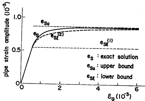
Fig. 5 Pipe Strain Amplitude. ( L/D=10^3 , h/D=15 , D/d=100 , G/E=2.5 \times 10^{-4} , \gamma_{cr}=1.4 \times 10^{-4} )
