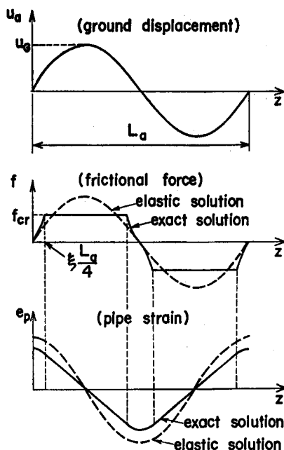
Fig. 3 Ground Displacement, Frictional Force, and Pipe Strain.
