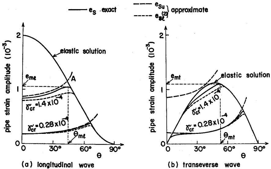
Fig. 7 Pipe Strain Amplitude. ( \epsilon_l = \gamma_l = 2 \times 10^{-3} , L_l/D = L_t/D = 10^3 , h/D = 15 , D/d = 100 , G/E = 2.5 \times 10^{-4} )
