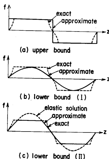
Fig. 4 Distribution of Frictional Forces for Approximate Pipe Strain.
