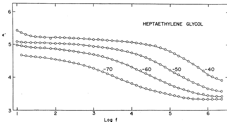
Fig. 10. Plots of \epsilon' versus frequency for solid heptaethylene glycol.
