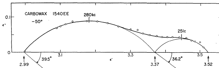
Fig. 8. Cole-Cole plots for solid Carbowax 1540 EE at -50^\circ\text{C} .
