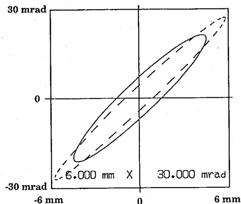
Fig. 8. Beam emittance at the downstream of the RFQ. The measured one (solid line) and the simulated one by the PARMTEQ code (dotted line). The beam energy is 2 MeV and the current is 400 \mu A.
