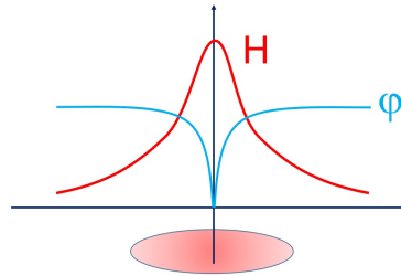
Fig. 3. The Abrikosov vortex in Type-II superconductors: a stable topological configuration composed of the magnetic field H and the Cooper-pair scalar field \varphi . The vortex has a topological charge on \Pi_1(U(1)) = \mathbf{Z} .
