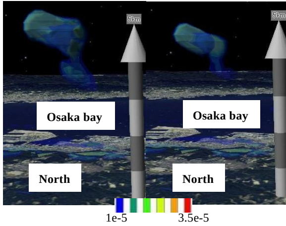
Fig. 13 3-D distribution of Q-value. (a) No control experiment and (b) Control experiment.
