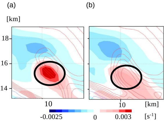
Fig. 15 Horizontal cross section of vertical vorticity at an altitude of 1.5 km. (a) No control experiment and (b) Control experiment.
