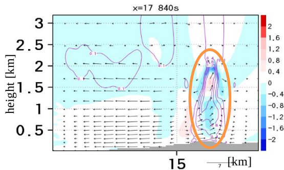
Fig. 8 Generation of updrafts due to the warm bubble. The shading indicates temperature deviation from the horizontal mean at the same altitude [K], and the contour indicates upwelling [ \text{ms}^{-1} ].
