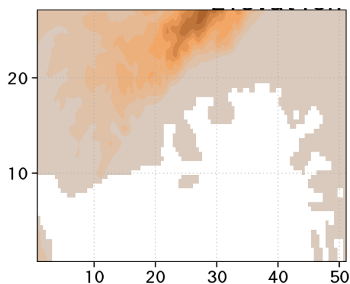
Fig. 4 Computational domain of the LES experiment. Both horizontal and vertical axes indicate the distance from the southwest edge of the computational domain [km].
