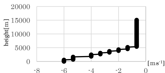
Fig. 6 Vertical profile of north-south wind. The horizontal axis indicates north-south wind (negative values indicate north wind).
