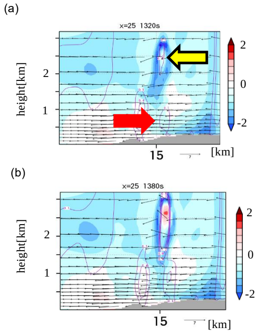
Fig. 11 (a) Upwelling at the center of the upwelling at 1320 s after the start of the computation and (b) merging with the upwelling caused by the warm bubble at 1380 s after the start of the computation. Shading indicates temperature deviation [\text{K}] , contours indicate upwelling [\text{ms}^{-1}] .
