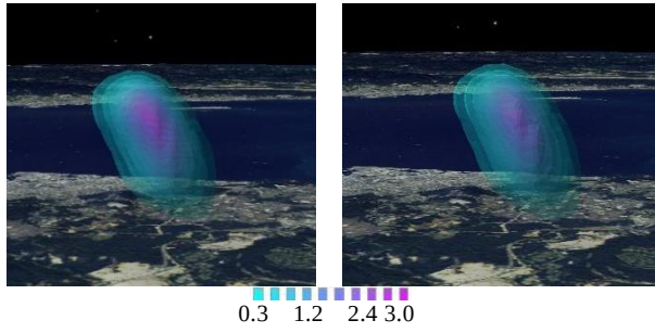
Fig. 12 Three-dimensional distribution of peak rainwater mixing ratio [ \text{gkg}^{-1} ] for (a) No control experiment and (b) Control experiment.
