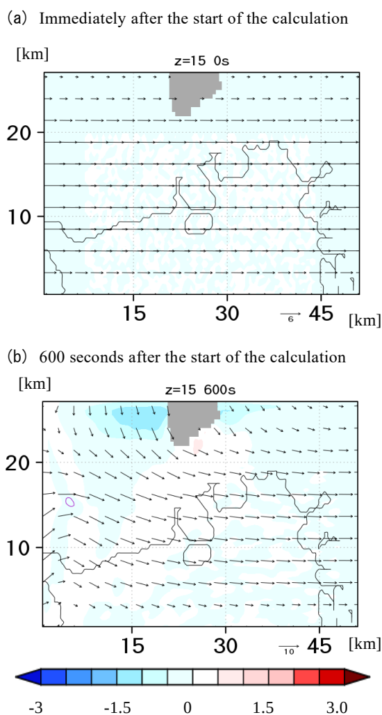
Fig. 5 Wind speed changes. (a) immediately after the start of the calculation, and (b) 600 seconds after the start of the calculation.
