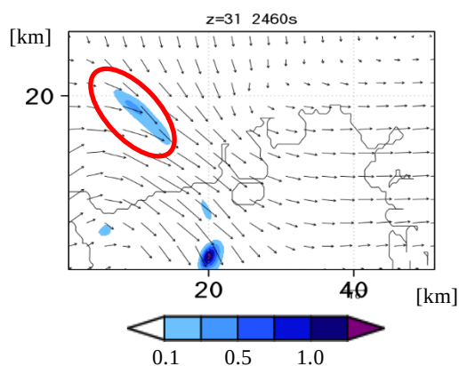
Fig. 7 Precipitation generated in Experiment 2. Vectors indicate horizontal wind and shading indicates rainwater mixing ratio [ \text{gkg}^{-1} ].
