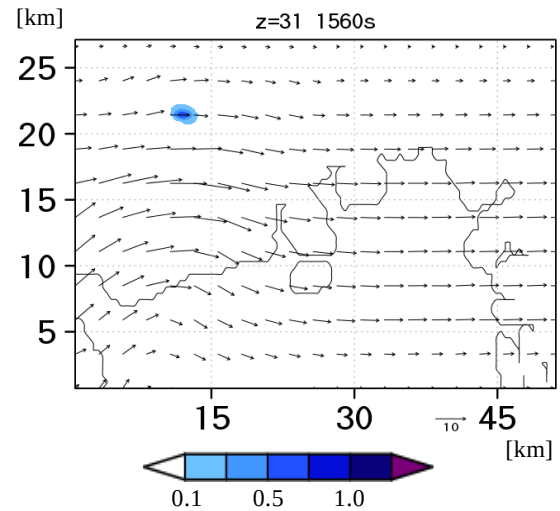
Fig. 9 Precipitation generated in Experiment 3. Vectors indicate horizontal wind and shading indicates rainwater mixing ratio [ \text{gkg}^{-1} ].
