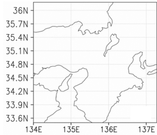
Fig. 2 Computational domain of CReSS
