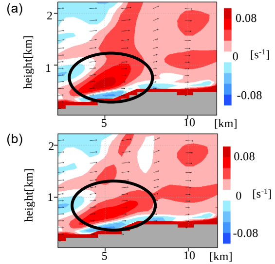
Fig. 14 Vertical distribution of horizontal vorticity. (a) No control experiment and (b) Control experiment. Vertical axis is altitude [km].
