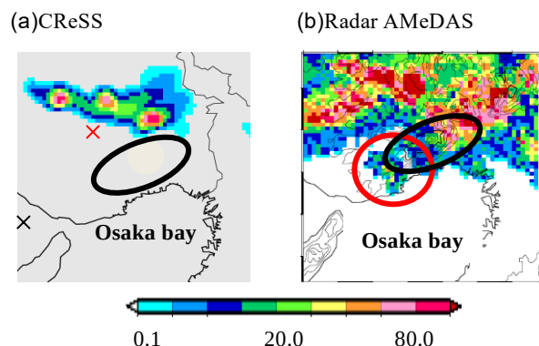
Fig. 3 (a) CReSS reproduced results and (b) radar AMeDAS observations of ground rainfall intensity [ \text{mmh}^{-1} ]. The black circle is Mt. Rokko.
