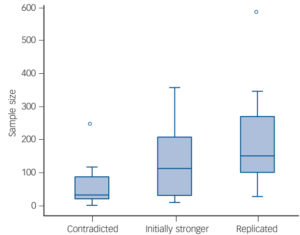
Fig. 2 Distribution of total sample size of the three study categories. Two extreme values are excluded: one was a contradicted study ( n=1759 ) and the other was a replicated study ( n=3282 ).
