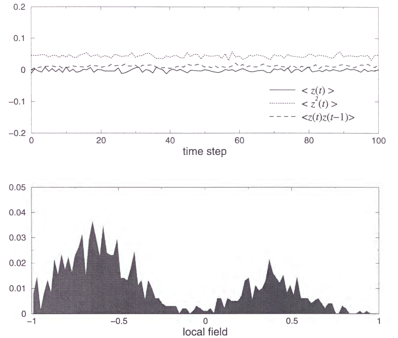
Figure 2.2: Top : Typical time evolution of statistics of crosstalk noise z(t) for a = 0.3 , \alpha = 0.15 , \theta = 0 , g = 0.33 , and the initial overlap m(0) = 0.6 . Bottom : Snap shot of distribution of local field h(t) .
