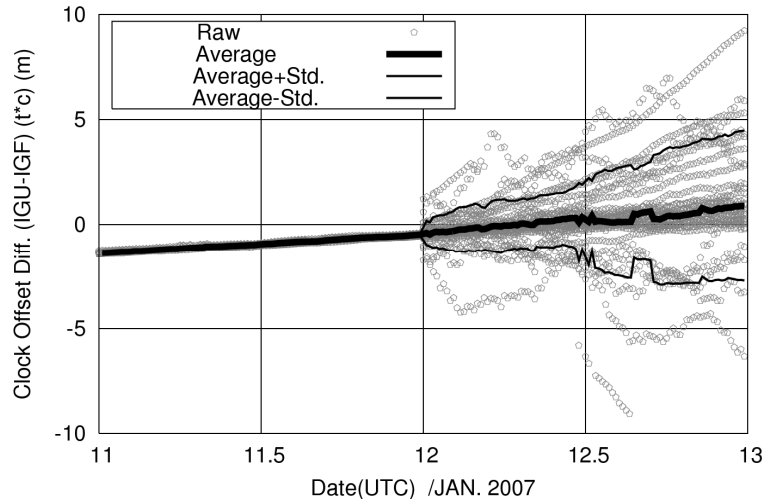
Figure 3. 13: Clock offset differences of IGU from IGF for all GPS satellites for two days (from 00 UTC, 11 Jan. to 00 UTC, 13, Jan., 2007) expressed in the unit of length (m). The gray open circles represent each difference; the black thick line, the average; and the two black thin lines, the average plus positive (negative) standard deviations. (Adapted from Shoji 2009)
