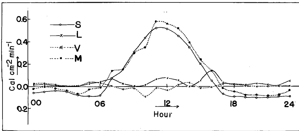
Fig. 4 Daily variation of thermal balance components. (19th March 1963)
