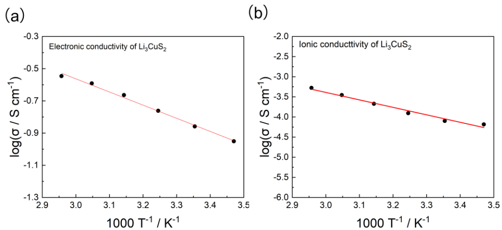
Figure 5.3. Arrhenius plot of (a) electronic conductivity of \text{Li}_3\text{CuS}_2 , and (b) ionic conductivity of \text{Li}_3\text{CuS}_2 .
