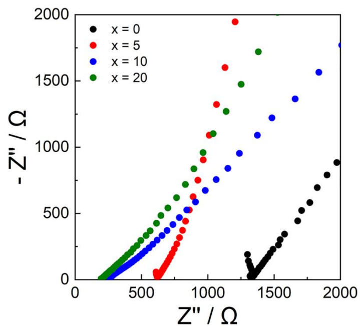
Figure 4.6. Nyquist plots of (100-x)(0.75\text{Li}_2\text{S}-0.25\text{V}_2\text{S}_3)-x\text{LiI} cathode with x = 0, 5, 10, 20 obtained by using electron-blocking cell at 25^\circ\text{C} .
