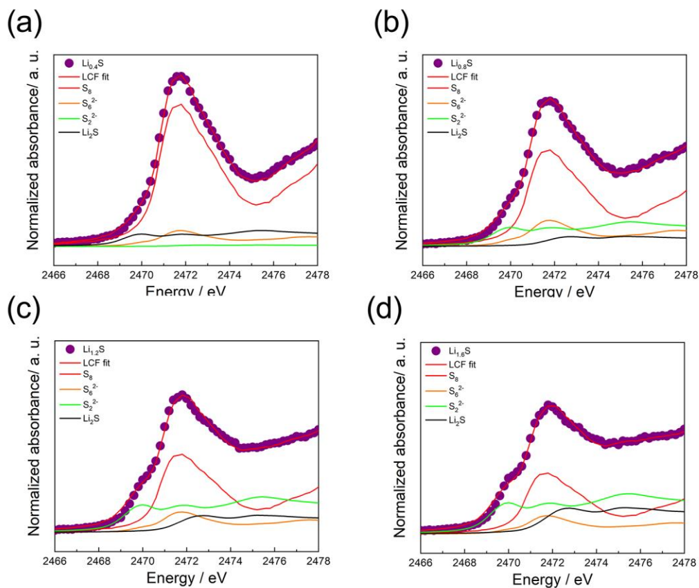
Figure 3.7. Linear combination fitting result of sulfur K -edge XANES of microporous carbon-supported sulfur cathode at discharge state of \text{Li}_{0.4}\text{S} , \text{Li}_{0.8}\text{S} , \text{Li}_{1.2}\text{S} and \text{Li}_{1.6}\text{S} .
