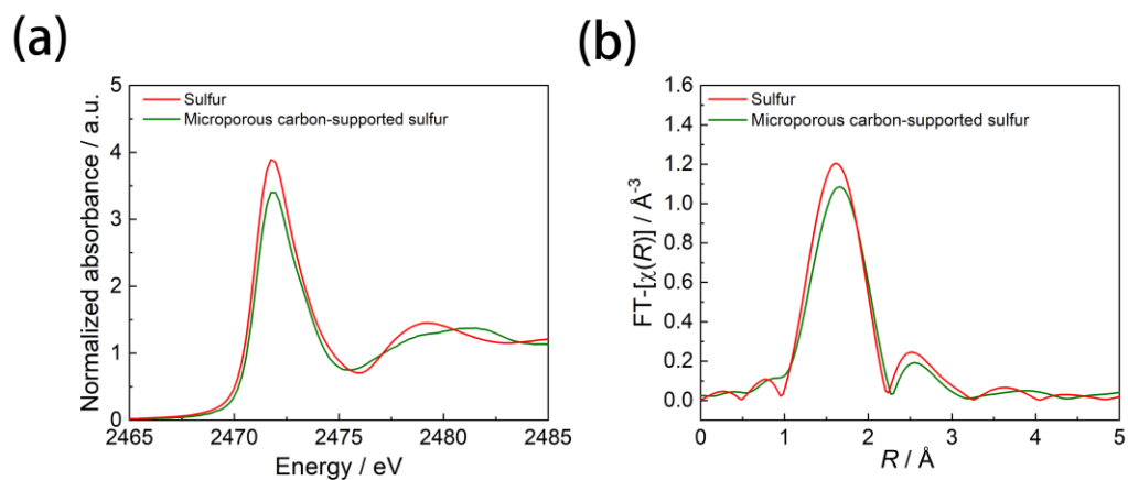
Figure 3.5. (a) S K-edge XANES profiles and (b) S K-edge Fourier-transformed EXAFS profiles obtained from XAS measurements for sulfur and microporous carbon-supported sulfur cathodes.
