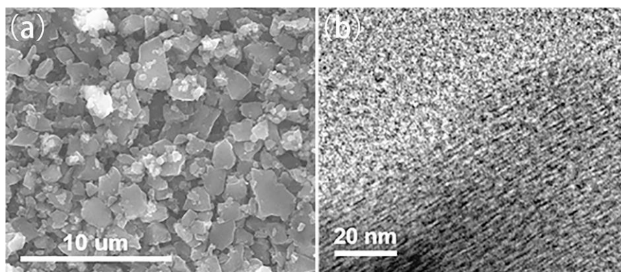
Figure 3.1. (a) SEM and (b) TEM images of microporous carbon.
