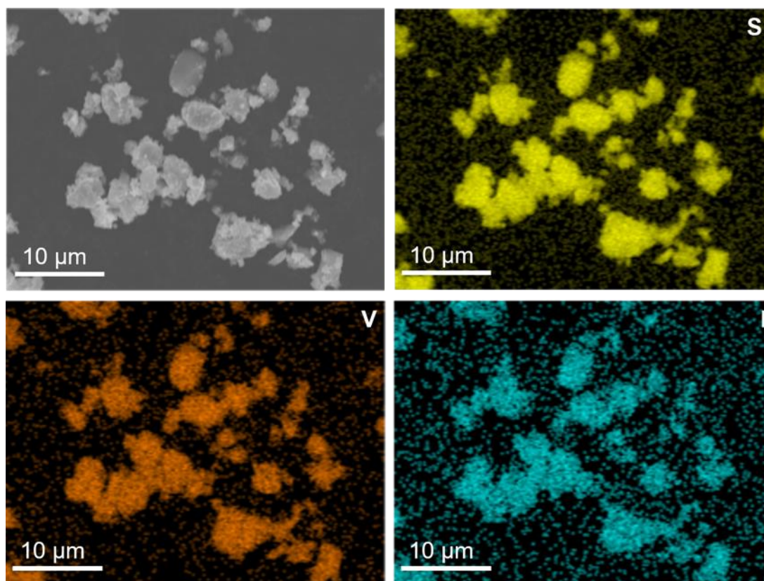
Figure 4.5. SEM-EDX mapping of 90(0.75Li 2 S-0.25V 2 S 3 )-10LiI cathode.
