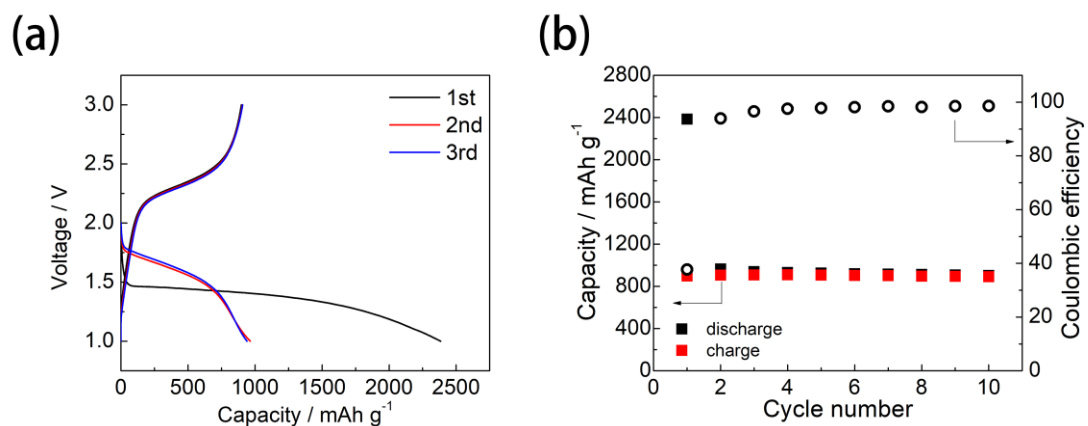
Figure 3.4. Charge/discharge profile (a) and cycle performance (b) of the microporous carbon-supported sulfur cathode.
