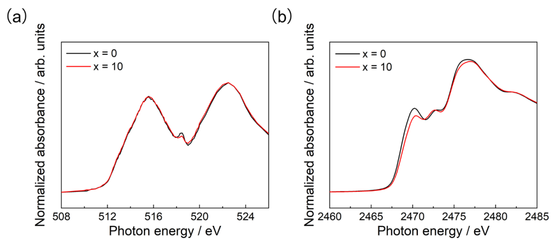
Figure 4.12. XANES of (a) V L -edge and (b) S K -edge for 0.75\text{Li}_2\text{S}-0.25\text{V}_2\text{S}_3 and 90(0.75\text{Li}_2\text{S}-0.25\text{V}_2\text{S}_3)-10\text{LiI} pristine.
