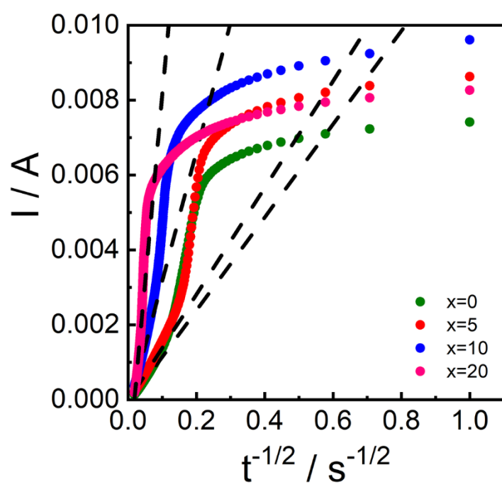
Figure 4.10. Cottrell plots of 100-x(0.75\text{Li}_2\text{S}-0.25\text{V}_2\text{S}_3)-x\text{LiI} with X=0, 5, 10, 20 .
