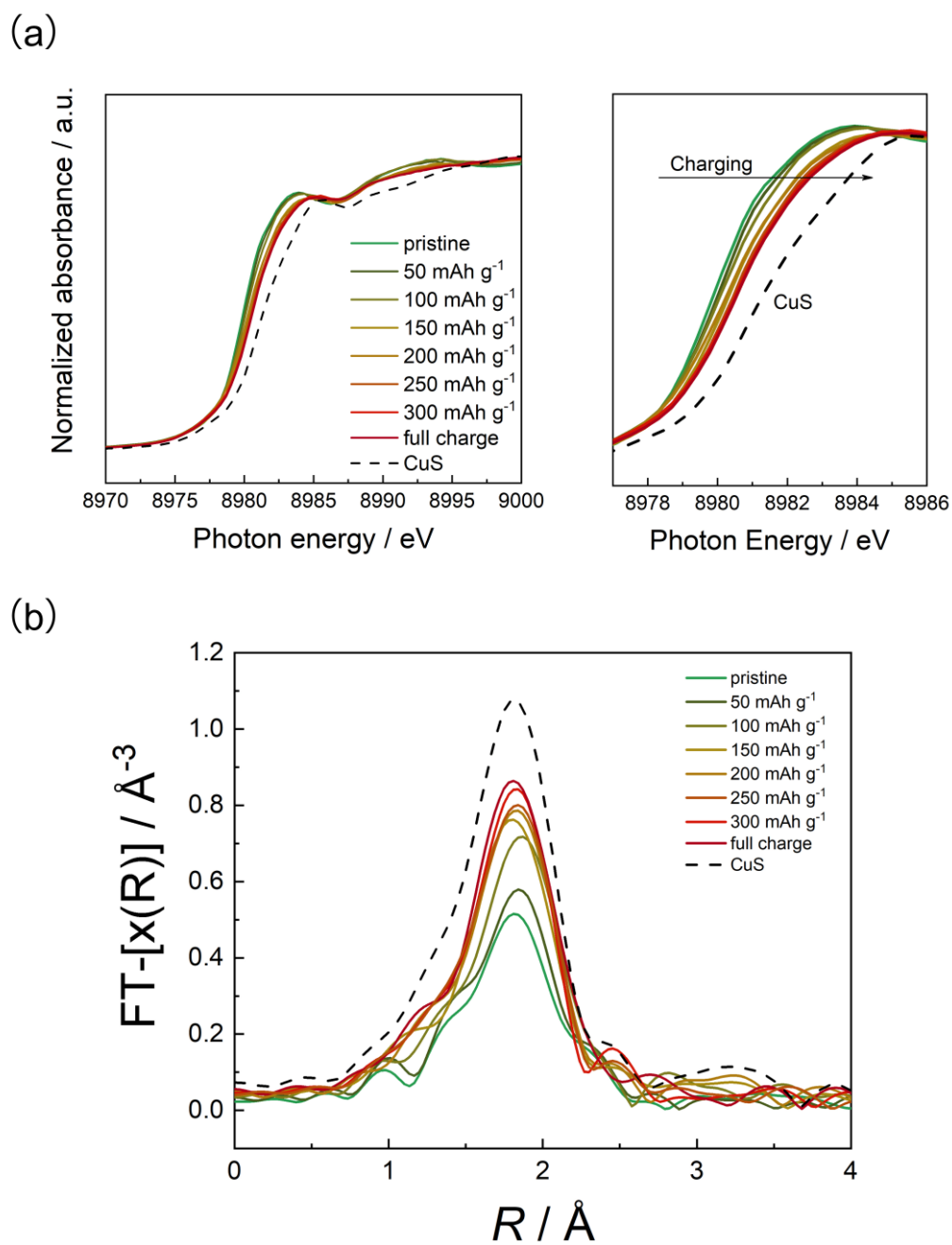
Figure 5.10 (a) XANES of copper k-edge of \text{Li}_3\text{CuS}_2\text{-Li}_3\text{PS}_4 during charge, (b) EXAFS of \text{Li}_3\text{CuS}_2\text{-Li}_3\text{PS}_4 during charge.
