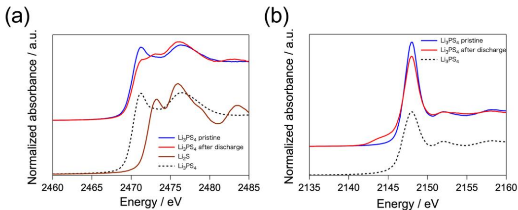
Figure 2.12. X-ray Absorption Near Edge Structure (XANES) for (a) S K -edge and (b) P K -edge of the \text{Li}_3\text{PS}_4 electrolyte after kept at the potential of 0 V (vs. \text{Li}^+/\text{Li} ). The XANES spectra of the \text{Li}_3\text{PS}_4 sample before and after electrochemical measurement were collected with partial fluorescence mode at BL13 in Rits SR, Japan.
