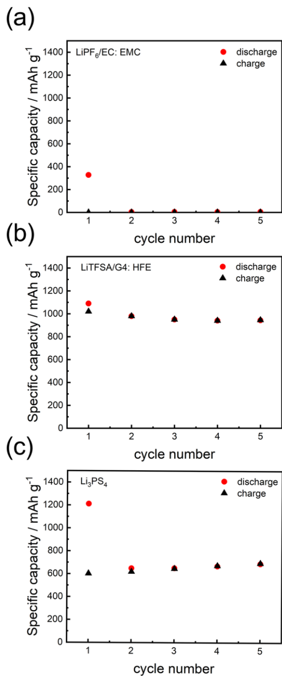
Figure 2.5. Cyclability for sulfur/CNovel cathode at (a) in the LiPF 6 /EC: EMC conventional liquid electrolyte, (b) in the LiTFSA/G4: HFE concentrated liquid electrolyte, and (c) in the Li 3 PS 4 solid-state electrolyte.
