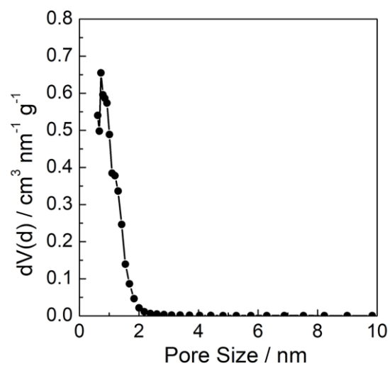
Figure 3.2. Pore size distribution of the microporous carbon obtained by N 2 adsorption isotherm measurement at -196 °C.
