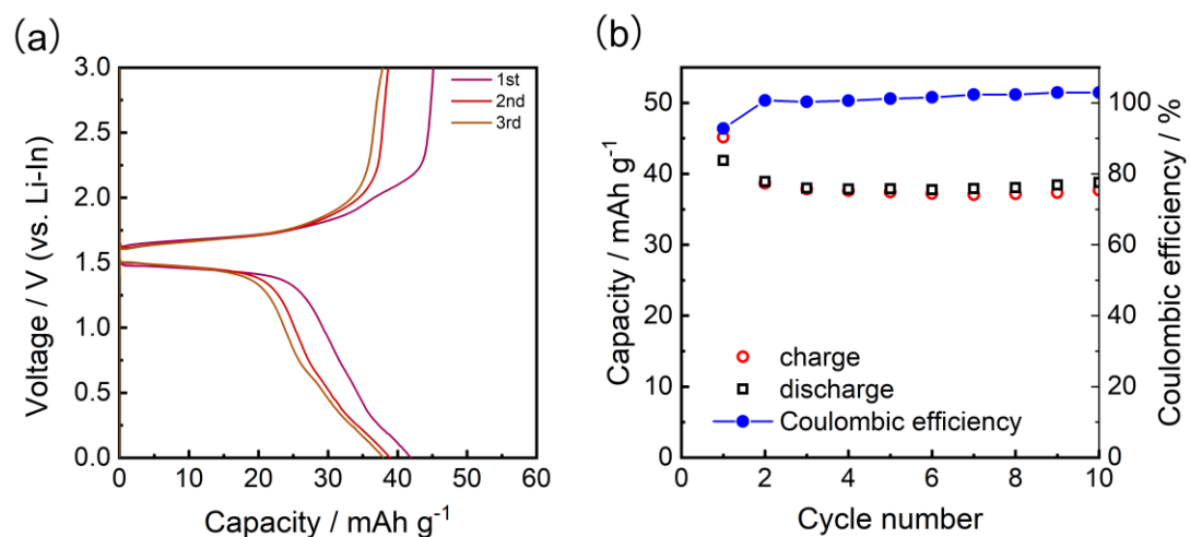
Figure 5.4 (a) Charge/discharge curves of Li 3 CuS 2 cathode at current density 0.13 mA / cm 2 , (b) charge and discharge cyclability of Li 3 CuS 2 at 0.13 mA / cm 2 .
