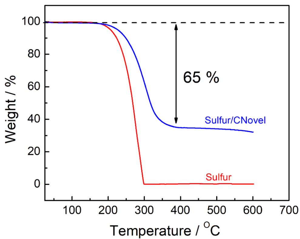
Figure 2.1. Thermo gravimetric analysis curves of sulfur and sulfur/CNovel powder.
