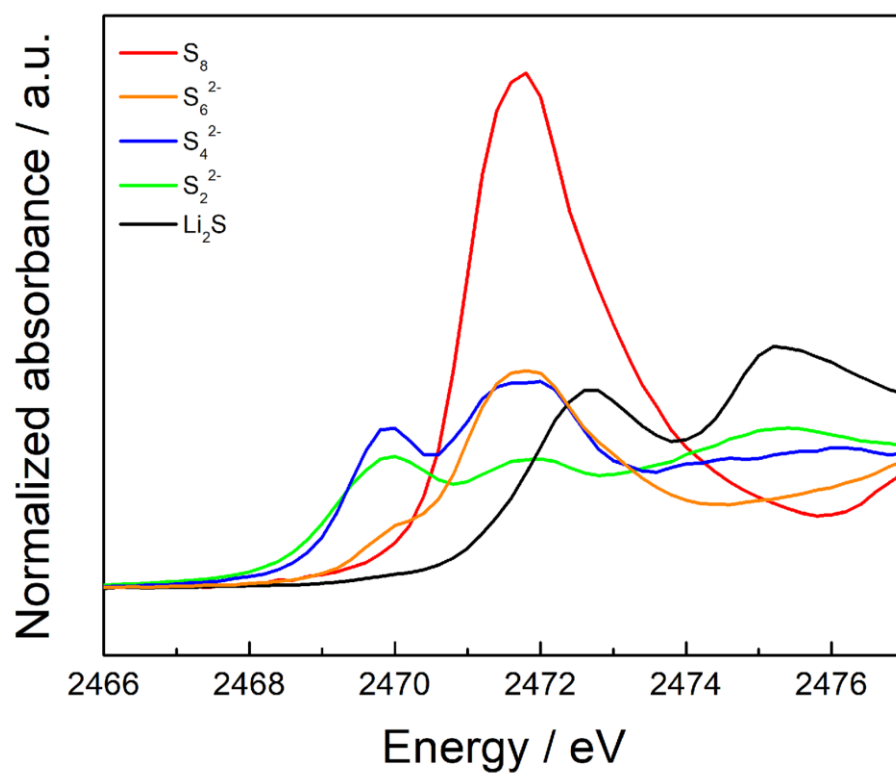
Figure 2.7. Sulfur K -edge XANES of standard materials S_8 , S_6^{2-} , S_4^{2-} , S_2^{2-} and Li_2S .
