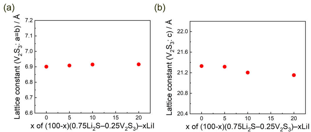
Figure 4.3. lattice constant of V_2S_3 in (100-x)(0.75Li_2S-0.25V_2S_3)-xLiI ( x = 0, 5, 10 , and 20) composites (a) a and b axis (b) c axis.
