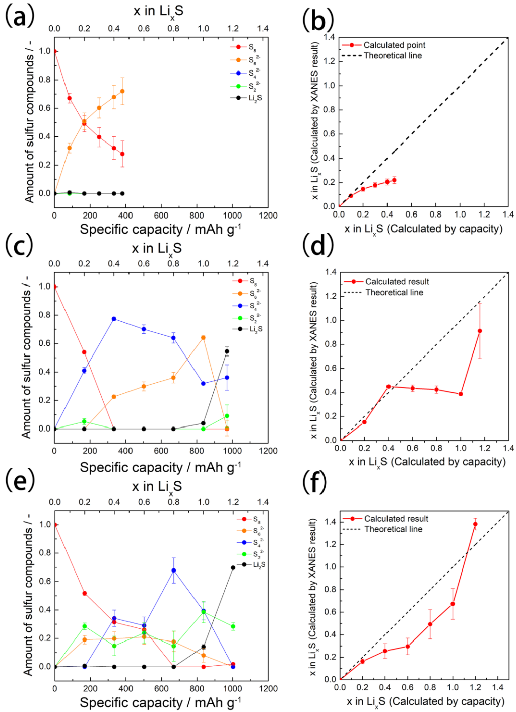
Figure 2.10. Sulfur compound ratio of the sulfur/CNovel cathode during first discharge process calculated by the linear combination fitting (LCF) analysis for the XANES spectra and lithium composition calculated by the LCF analysis and electrochemical capacity; (a), (b) in the LiPF 6 /EC: EMC conventional liquid electrolyte, (c), (d) in the LiTFSA/G4: HFE concentrated liquid electrolyte, (e), (f) in the Li 3 PS 4 solid-state electrolyte.
