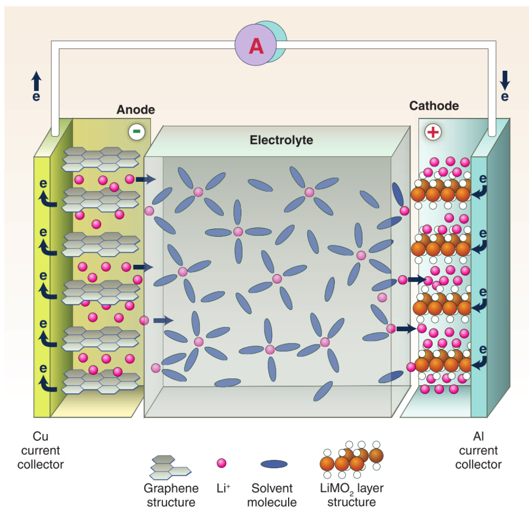
Figure 1.1. Schematic of a lithium ion battery.
