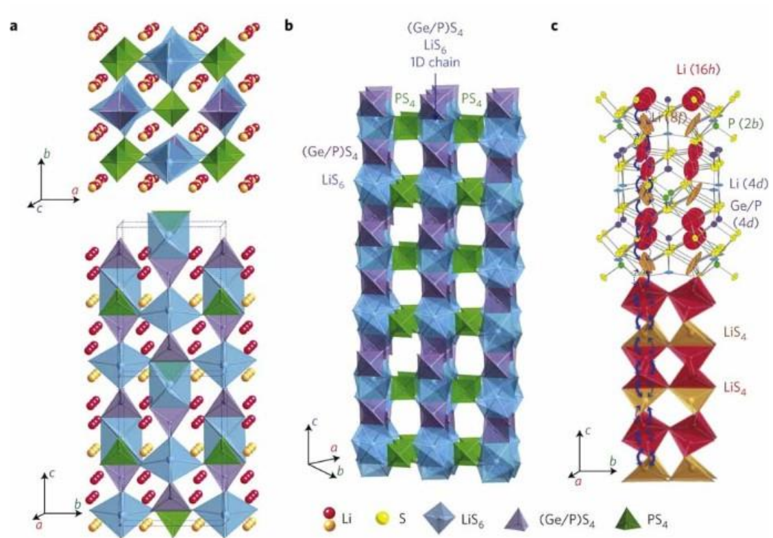
Figure 1.10. Crystal structure of \text{Li}_{10}\text{GeP}_2\text{S}_{12} .
