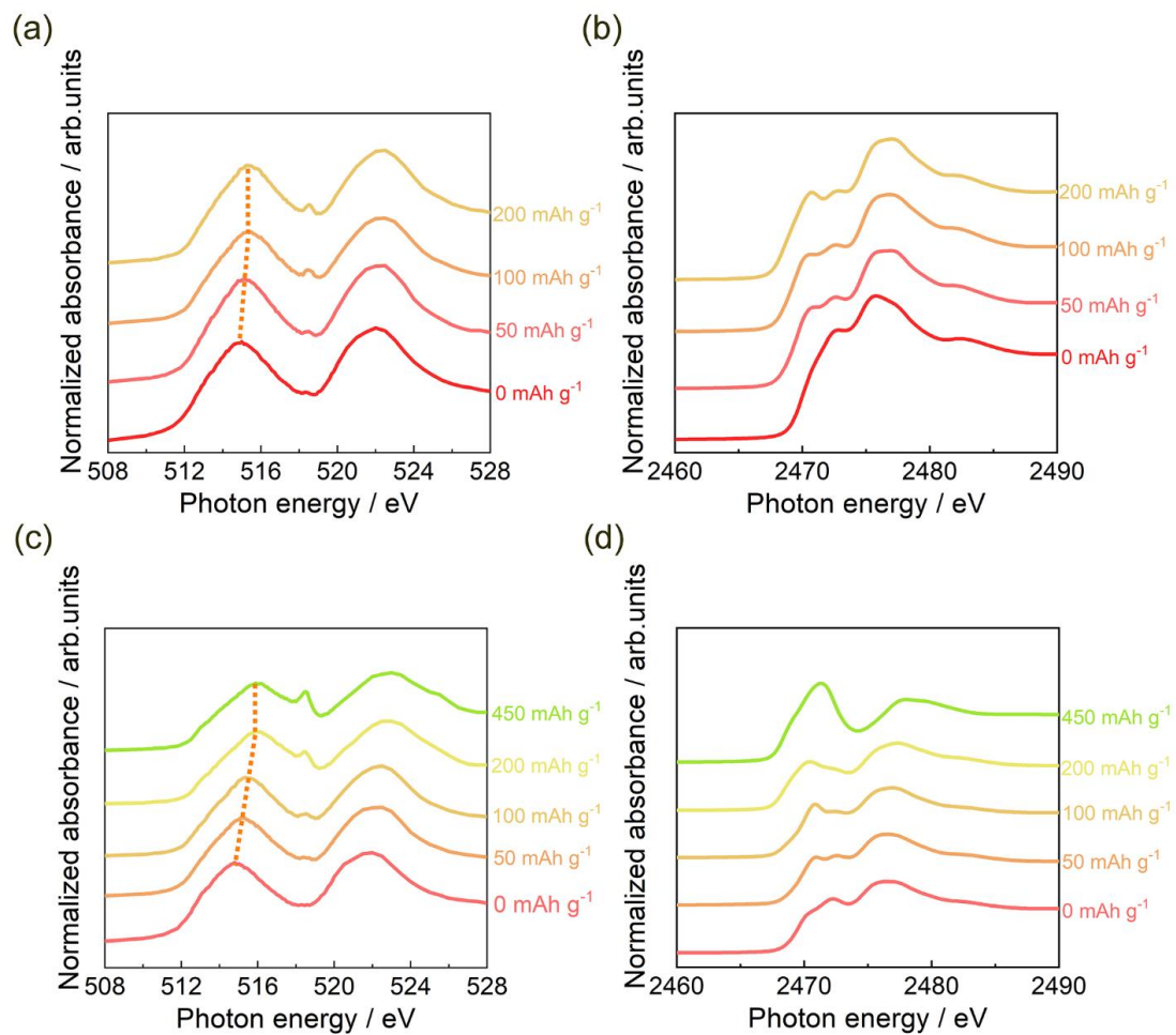
Figure 4.15. XANES for (a) V L -edge, (b) S K -edge of 100(0.75Li 2 S-0.25V 2 S 3 ) during the second charge process at different state of charge (0 mAh g -1 , 50 mAh g -1 , 100 mAh g -1 and 200 mAh g -1 ), (c) V L -edge, and (d) S K -edge of 90(0.75Li 2 S-0.25V 2 S 3 )-10LiI cathode during the second charge at different state of charge (0 mAh g -1 , 50 mAh g -1 , 100 mAh g -1 , 200 mAh g -1 and 450 mAh g -1 ).
