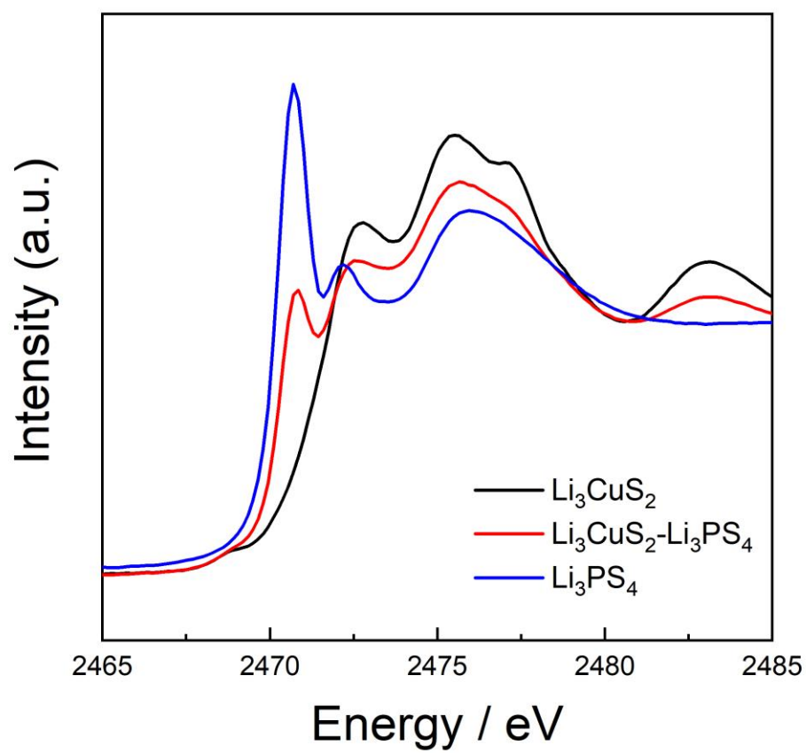
Figure 5.8. S K-edge XANES of Li 3 PS 4 , Li 3 CuS 2 and Li 3 CuS 2 -Li 3 PS 4 .
