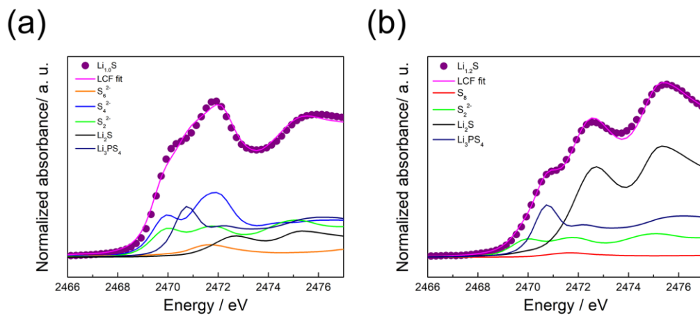
Figure 2.9. Linear combination fitting result of sulfur K -edge XANES of sulfur/CNovel cathode in all solid-state lithium sulfur battery by using stander material with \text{Li}_3\text{PS}_4 at discharge state of (a) \text{Li}_{1.0}\text{S} and (b) \text{Li}_{1.2}\text{S} .
