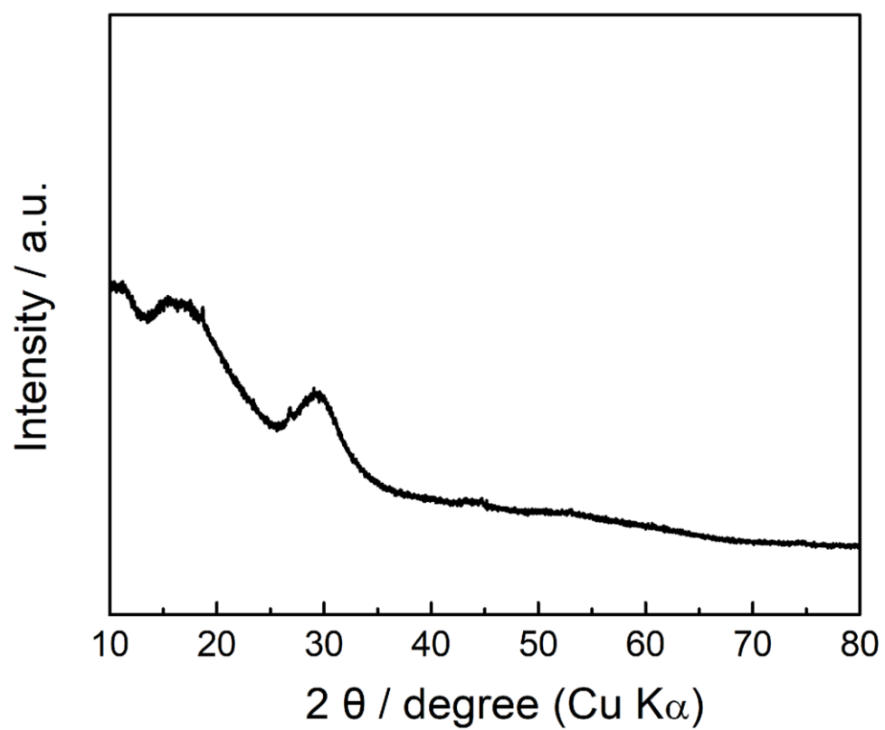
Figure 2.2. XRD pattern of the prepared \text{Li}_3\text{PS}_4 .
