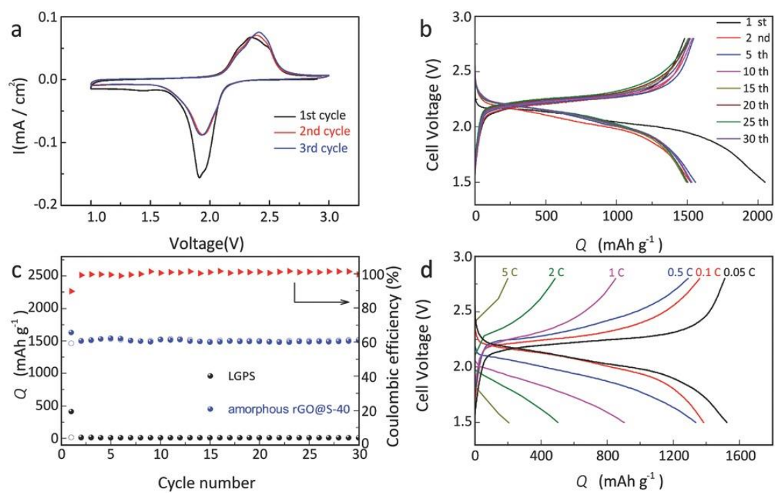
Figure 1.7. Cyclic voltammogram of the amorphous rGO@S-40 composite.
