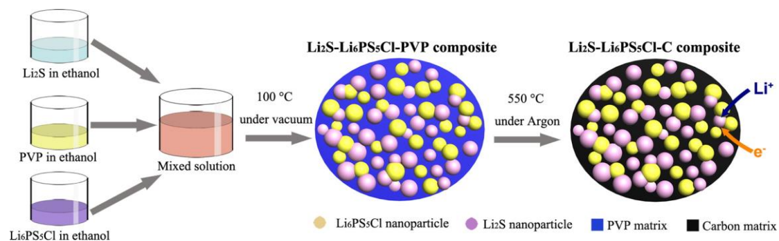
Figure 1.8. Schematic illustration of the bottom-up synthesis of the mixed conducting \text{Li}_2\text{S} nanocomposite.
