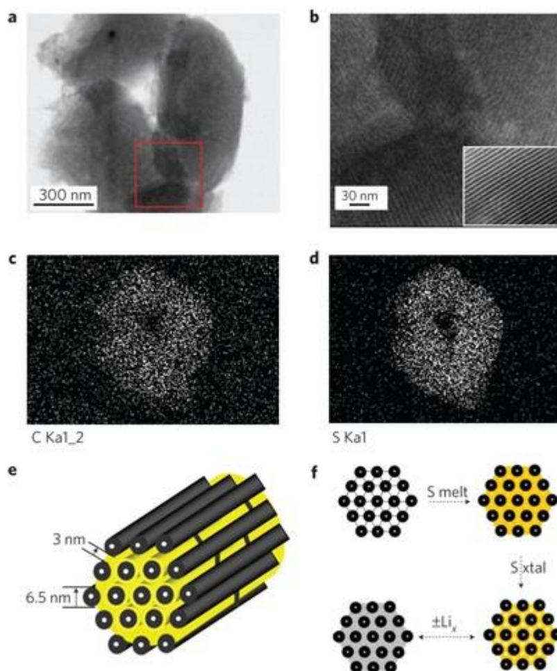
Figure 1.3. TEM image and elemental maps of a CMK-3/S-155 composite particle and schematic diagrams of the structure and redox processes.
