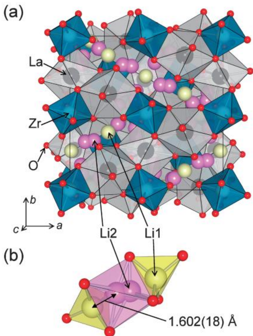
Figure 1.9. (a) Crystal structure of cubic \text{Li}_7\text{La}_3\text{Zr}_2\text{O}_{12} . (b) Coordination polyhedral around the Li1 and Li2 sites.
