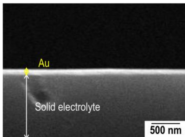
Figure 1.12. Cross-sectional SEM image of the interface between Au thin films and \text{Li}_2\text{S-P}_2\text{S}_5 solid electrolytes.
