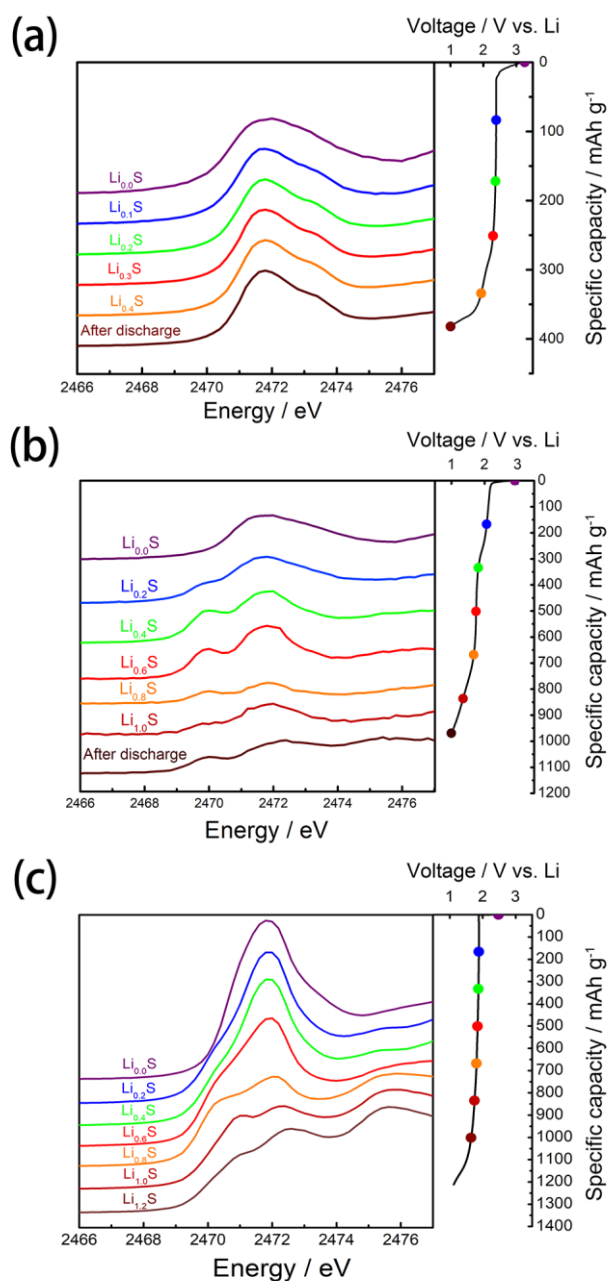
Figure 2.6. (a) S K-edge XANES of sulfur/CNovel cathode at different discharge states (a) in the \text{LiPF}_6/\text{EC}:\text{EMC} conventional liquid electrolyte, (b) in the \text{LiTFSA}/\text{G4}:\text{HFE} concentrated liquid electrolyte, and (c) in the \text{Li}_3\text{PS}_4 solid-state electrolyte.
