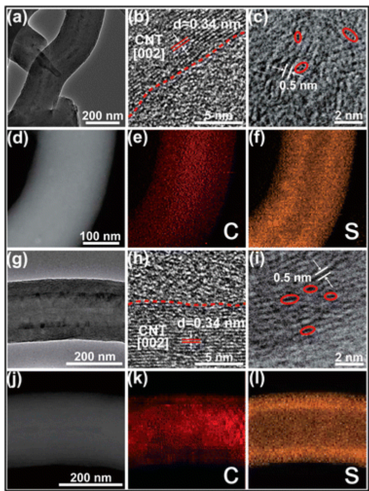
Figure 1.4. Structural characterization of S/(CNT@MPC) before and after 200 cycles at 0.1 C.
