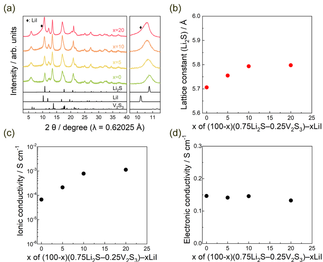
Figure 4.1. (a) X-ray diffraction patterns of (100-x)(0.75\text{Li}_2\text{S}-0.25\text{V}_2\text{S}_3)-x\text{LiI} ( x = 0, 5, 10 , and 20 ) composites, (b) lattice constant of \text{Li}_2\text{S} in (100-x)(0.75\text{Li}_2\text{S}-0.25\text{V}_2\text{S}_3)-x\text{LiI} ( x = 0, 5, 10 , and 20 ) composites, and (c) and (d) ionic and electronic conductivities, respectively, of (100-x)(0.75\text{Li}_2\text{S}-0.25\text{V}_2\text{S}_3)-x\text{LiI} ( x = 0, 5, 10 , and 20 ) composites at 25^\circ\text{C} .
