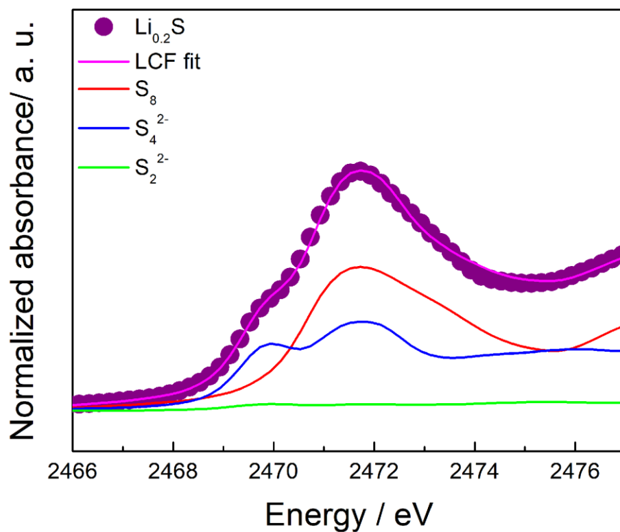
Figure 2.11. Linear combination fitting result of sulfur K -edge XANES of sulfur/CNovel cathode in LiTFSA/G4: HFE concentrated liquid electrolyte at discharge state of \text{Li}_{0.2}\text{S} .
