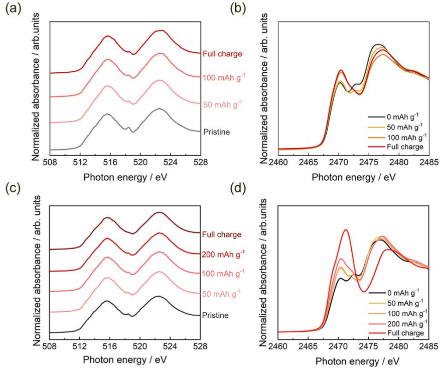
Figure 4.11. (a) V L -edge and (b) S K -edge X-ray absorption near edge structure spectra of the 100(0.75Li 2 S–0.25V 2 S 3 ) cathode during the first charge process at different charge states (pristine, 50 mAh g -1 , 100 mAh g -1 , and full charge), (c) V L -edge, and (d) S K -edge X-ray absorption near edge structure spectra of the 90(0.75Li 2 S–0.25V 2 S 3 )–10LiI cathode during the first charge process at different charge states (pristine, 50 mAh g -1 , 100 mAh g -1 , 200 mAh g -1 , and full charge).
