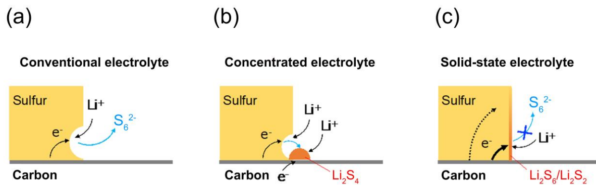
Figure 2.14. Reaction model of sulfur cathodes in (a) conventional electrolyte, (b) concentrated electrolyte and (c) solid-state electrolyte.
