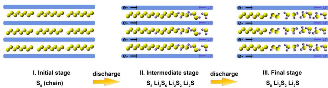
Figure 3.8. Reaction model for the microporous carbon-supported sulfur cathodes.
