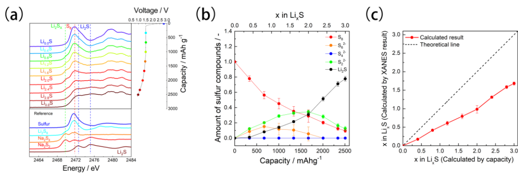
Figure 3.6. (a) Sulfur K-edge XANES spectra obtained from the operando XAS measurements of the microporous carbon-supported sulfur cathode. (b) Sulfur compound ratio of the microporous carbon-supported sulfur cathode during the first discharge, calculated by the linear combination fitting (LCF) analysis of XANES spectra. (c) Lithium compositions calculated from the LCF analysis and electrochemical capacity data.
