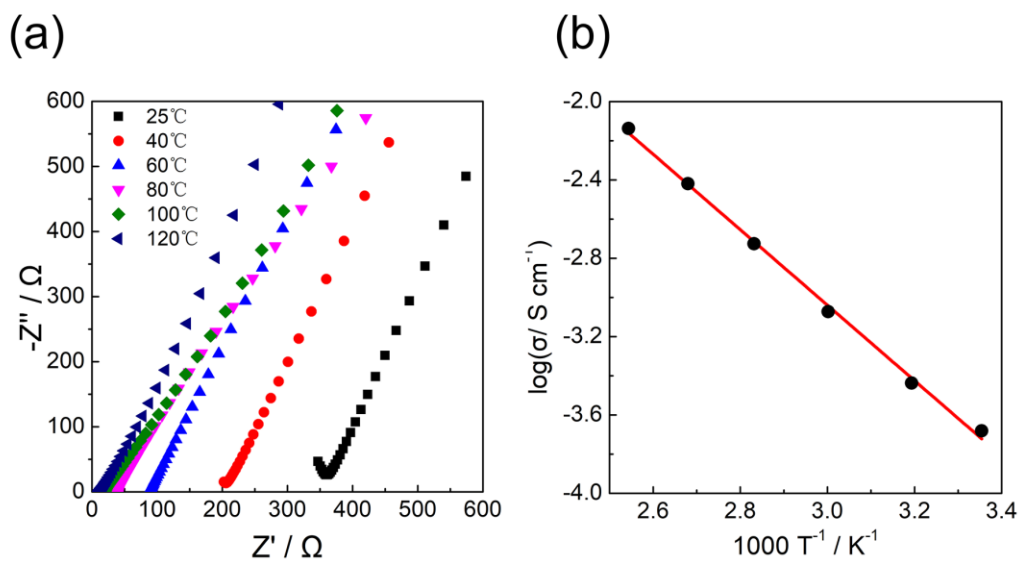
Figure 2.3. (a) Nyquist plots of the prepared \text{Li}_3\text{PS}_4 at different temperature, (b) Temperature dependence of the ionic conductivity of \text{Li}_3\text{PS}_4 .
