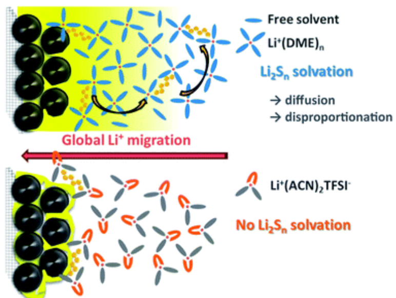
Figure 1.6. Concept of a nonsolvent for polysulphides in a Li–S battery.
