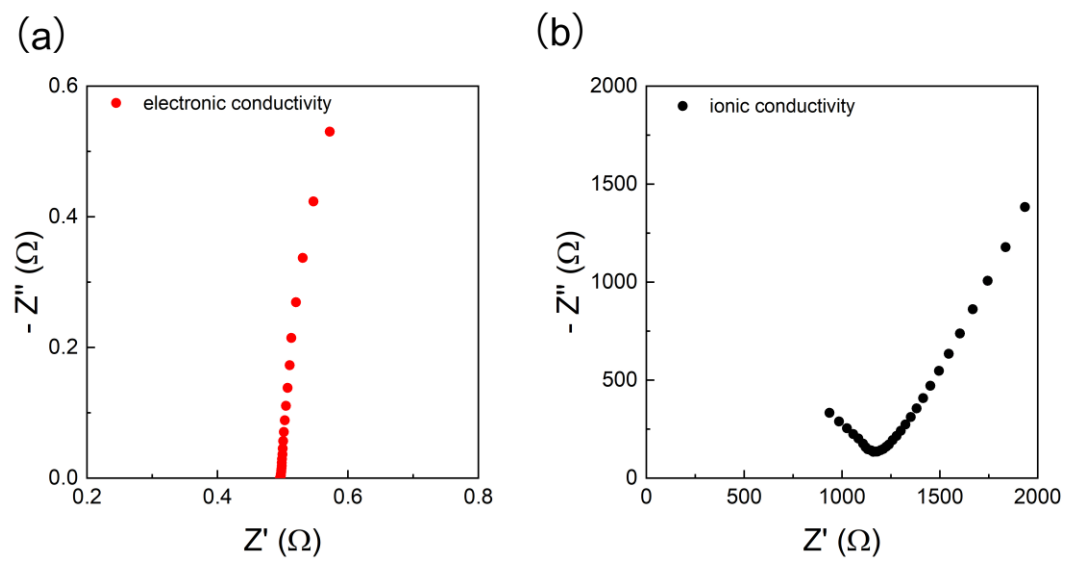
Figure 5.2. (a) electronic conductivity of \text{Li}_3\text{CuS}_2 , (b) ionic conductivity of \text{Li}_3\text{CuS}_2 .
