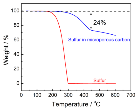
Figure 3.3. Thermogravimetric analysis curves of sulfur and microporous carbon-supported sulfur under an Ar atmosphere at a heating rate of 5 °C/min.
