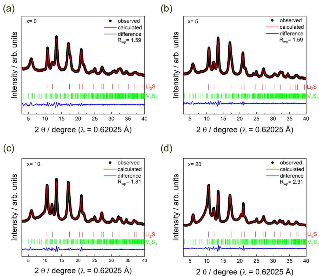
Figure 4.2. XRD pattern and Le Bail analytical fitting profile of (100-x)(0.75\text{Li}_2\text{S}-0.25\text{V}_2\text{S}_3)-x\text{LiI} (a) x=0 , (b) x=5 , (c) x=10 , and (d) x=20 .
