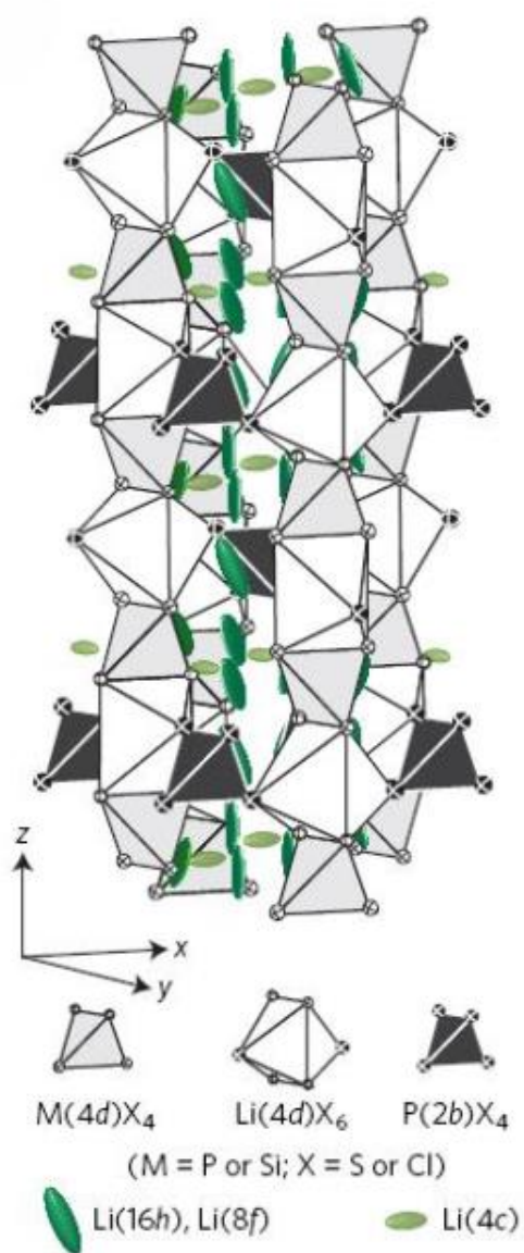
Figure 1.11. Crystal structure of Li_{9.54}Si_{1.74}P_{1.44}S_{11.7}Cl_{0.3} .
