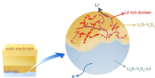
Figure 4.18. Model of self-forming ion conduction pathway in \text{Li}_2\text{S-V}_2\text{S}_3\text{-LiI} composites.
