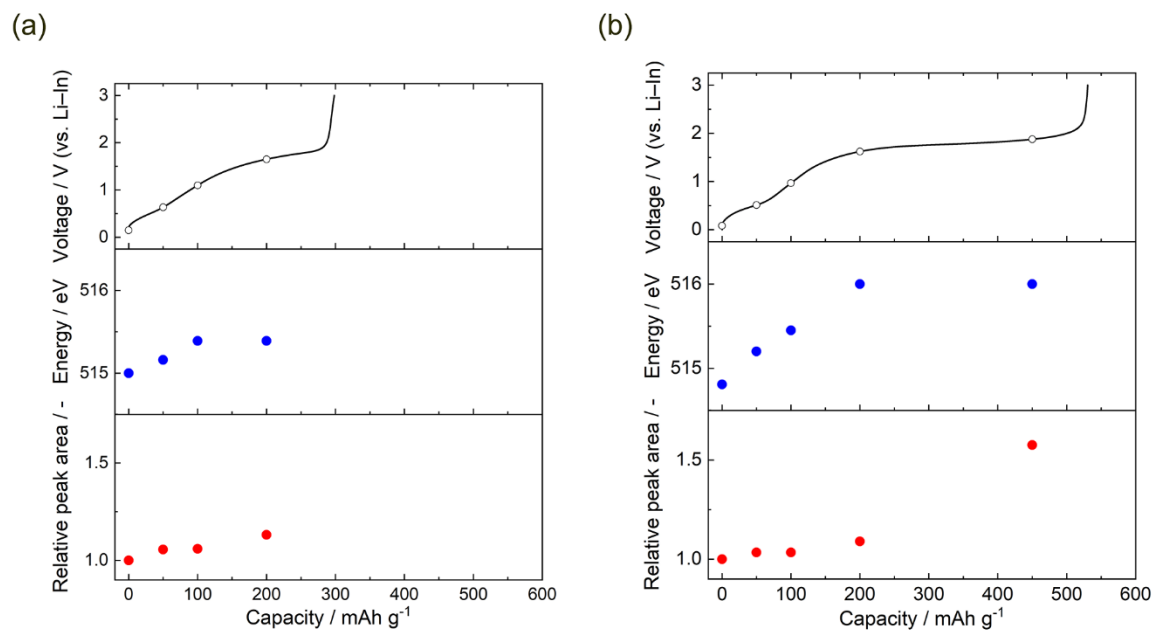
Figure 14. Charge curve (top), peak top energy in the V L -edge X-ray absorption near edge structure (XANES) spectra (middle), and relative peak area in the S K -edge XANES spectra (bottom) of the (a) 100(0.75Li 2 S–0.25V 2 S 3 ) and (b) 90(0.75Li 2 S–0.25V 2 S 3 )10LiI cathodes during the second charge process.
