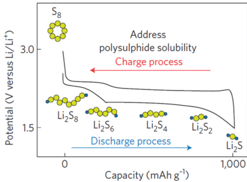
Figure 1.2. Voltage profiles of a Li-S cell.
