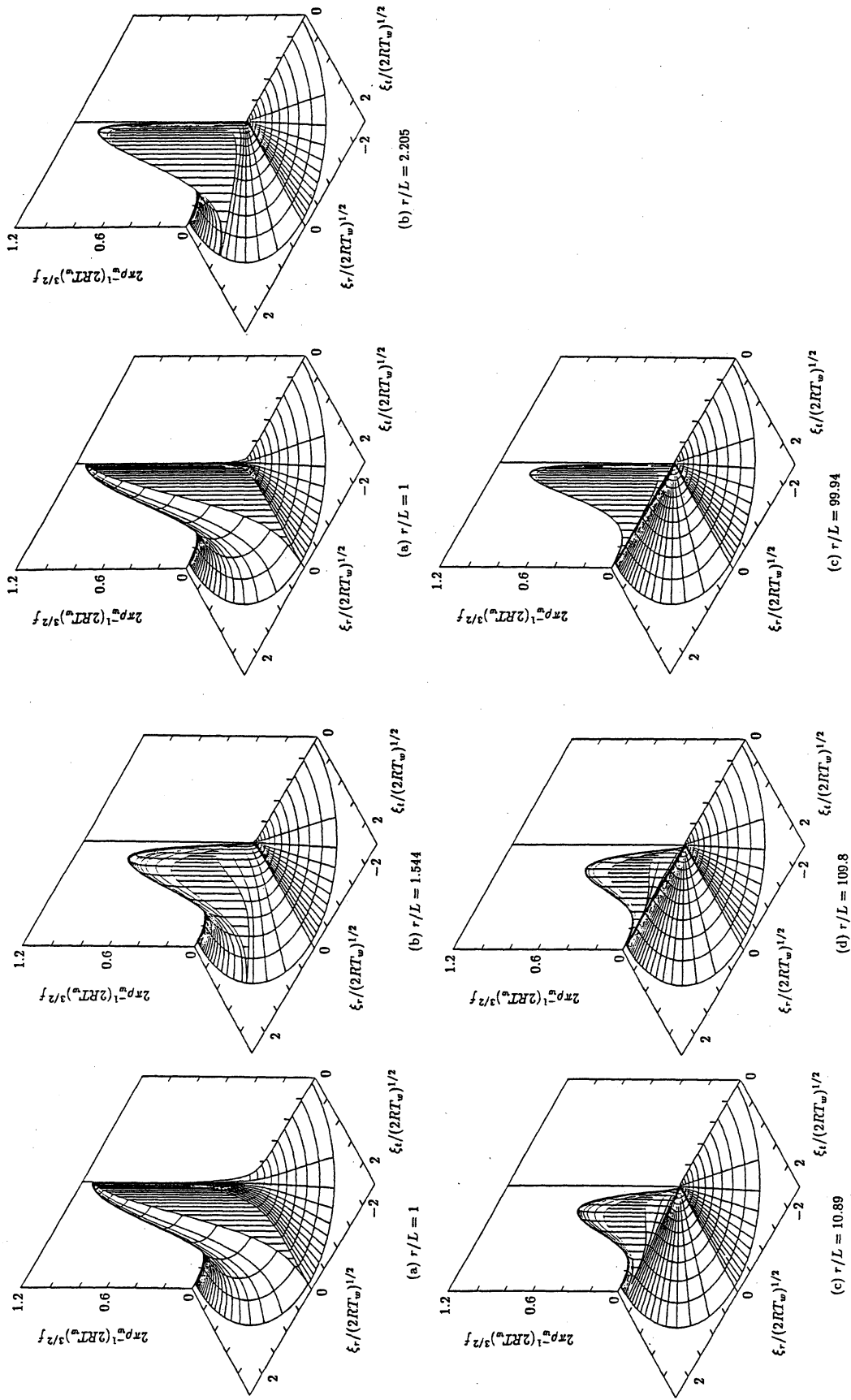
FIG. 11. The nondimensional velocity distribution function 2\pi\rho_w^{-1}(2RT_w)^{3/2}f at Kn_w = 10 . (a) r/L = 1 , (b) r/L = 2.205 , and (c) r/L = 99.94 .
