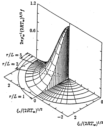
FIG. 12. The nondimensional velocity distribution function 2\pi\rho_w^{-1}(2RT_w)^{3/2}f at Kn_w = \infty . The distribution is the part \xi_r/\xi > [1 - (L/r)^2]^{1/2} of the function 2\pi^{-1/2}\exp(-\xi^2/2RT_w) .
