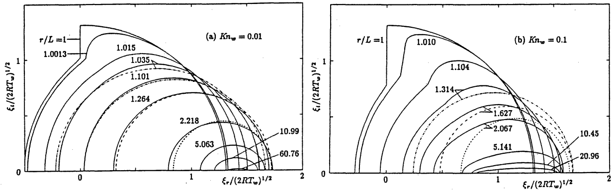
FIG. 14. The contour of 2\pi\rho_w^{-1}(2RT_w)^{3/2}f = 0.2 for various points r/L . (a) Kn_w = 0.01 and (b) Kn_w = 0.1 . The contour of the local Maxwellian is shown by: ---- [ r/L = 1.035 ( Kn_w = 0.01 )], --- [ r/L = 1.101 ( Kn_w = 0.01 ), 1.314 ( Kn_w = 0.1 )], ---- [ r/L = 1.264 ( Kn_w = 0.01 ), 1.627 ( Kn_w = 0.1 )], and ..... [ r/L = 2.218 ( Kn_w = 0.01 ), 2.067 ( Kn_w = 0.1 )]. The dashed line ---- corresponds to Figs. 7(a) and 13(a) ( Kn_w = 0.01 ) or Figs. 8(c) and 13(b) ( Kn_w = 0.1 ). The flow deviates considerably from the local Maxwellian over the whole field when Kn_w = 0.1 .
