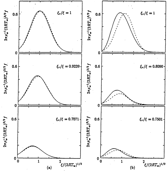
FIG. 13. Comparison with the local Maxwellian. (a) Kn_w = 0.01 and r/L = 1.264 ; (b) Kn_w = 0.1 and r/L = 1.627 . The dashed line represents the local Maxwellian 2\pi\rho_w^{-1}(2RT_w)^{3/2}f_e . The f_e has the same density, flow velocity, and temperature as f . The f in (a) corresponds to Fig. 7(a) and \bullet in Fig. 15, and that in (b) to Fig. 8(c) and \circ in Fig. 15.
