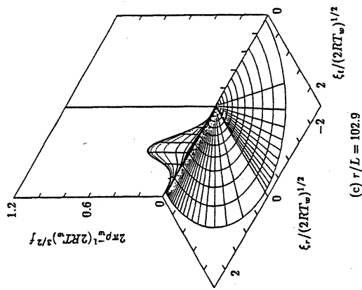
FIG. 9. The nondimensional velocity distribution function 2\pi\rho_w^{-1}(2RT_w)^{3/2}f at Kn_w = 0.1 (II): the transition region to free molecular region. (a) r/L = 5.141 , (b) r/L = 20.96 , and (c) r/L = 102.9 .
