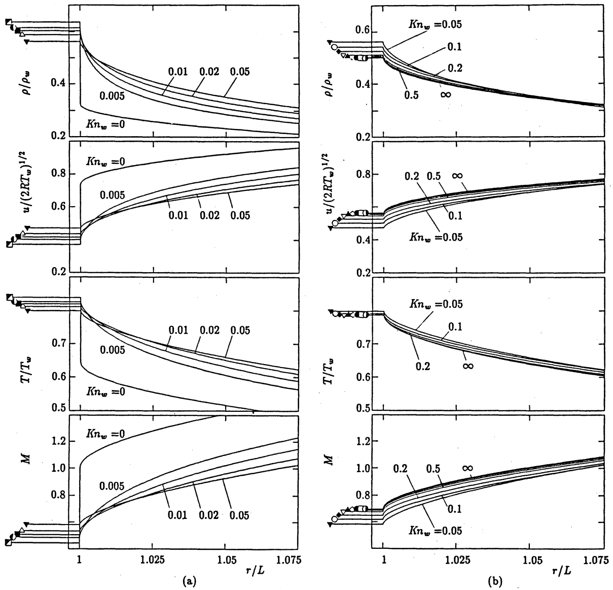
FIG. 1. The profiles of the macroscopic variables \rho/\rho_w , u/(2RT_w)^{1/2} , T/T_w , and M in the neighborhood of the sphere for various Knudsen numbers Kn_w . (a) Kn_w = 0-0.05 and (b) 0.05-\infty . The value on the sphere are marked with \blacksquare for Kn_w = 0 , \bullet for 0.005, \blacksquare for 0.01, \triangle for 0.02, \blacktriangledown for 0.05, \circ for 0.1, \blacklozenge for 0.2, \nabla for 0.5, \blacktriangle for 1, \diamond for 2, \bullet for 5, \square for 10, and \bigcirc for \infty .
