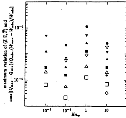
FIG. 17. The \hat{r}\theta_\zeta lattice dependence of (\hat{\rho}, \hat{u}, \hat{T}) , (Q_{\max} - Q_{\min})/Q_{\min} and (W_{\max} - W_{\min})/W_{\min} . The maximum variation of (\hat{\rho}, \hat{u}, \hat{T}) over the whole lattice points on 1 \leq \hat{r} \leq \hat{r}_D for different numbers I and (K, \bar{K}) of the \hat{r}\theta_\zeta lattice points are marked with hollow symbols. The \hat{r}\theta_\zeta lattice dependence of \max[(Q_{\max} - Q_{\min})/Q_{\min}, (W_{\max} - W_{\min})/W_{\min}] is marked with black symbols. Let LS be the \hat{r}\theta_\zeta lattice system, described in the first paragraph in Sec. V D, with which the results in Sec. V A, B, and C are obtained (Note that it depends on Kn_w ). M_0 is the same lattice system as LS for Kn_w = 0.01, 0.1 , and 10 , and M_0 is that with double (K, \bar{K}) of LS for Kn_w = 1 . M_n is a test lattice system with double I and (K, \bar{K}) of those of M_{n-1} . The \nabla indicates the maximum variation of (\hat{\rho}, \hat{u}, \hat{T}) between M_{-3} and M_{-2} lattices; \Delta between M_{-2} and M_{-1} ; \square between M_{-1} and M_0 ; \diamond between M_0 and M_1 . The \bullet indicates \max[(Q_{\max} - Q_{\min})/Q_{\min}, (W_{\max} - W_{\min})/W_{\min}] for M_{-3} ; \blacktriangledown for M_{-2} ; \blacktriangle for M_{-1} ; \blacksquare for M_0 ; \blacklozenge for M_1 . From separate tests, the results \square and \blacksquare are not influenced if LS is taken as M_0 for Kn_w = 1 .
