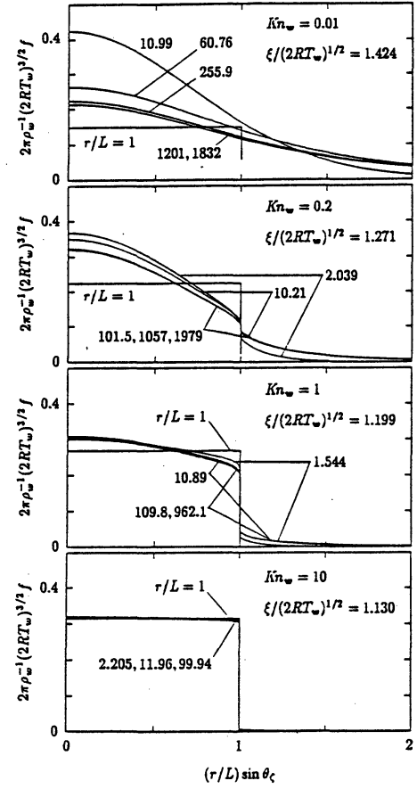
FIG. 16. The nondimensional velocity distribution function 2\pi\rho_w^{-1}(2RT_w)^{3/2}f at some \xi/(2RT_w)^{1/2} versus (r/L)\sin\theta_\zeta ( \theta_\zeta \leq \pi/2 ) for various r/L .
