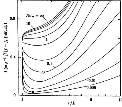
FIG. 15. \delta (= \rho^{-1} \int |f - f_e| \xi_r d\xi_r d\xi_t) versus r/L . The symbols ● and ○ correspond to Figs. 13(a) and 13(b) respectively. The \delta is a measure of deviation of the flow ( f ) from the local Maxwellian distribution ( f_e ) ( \delta = 0 when f = f_e , and \delta = 2 when f and f_e are disjoint).
