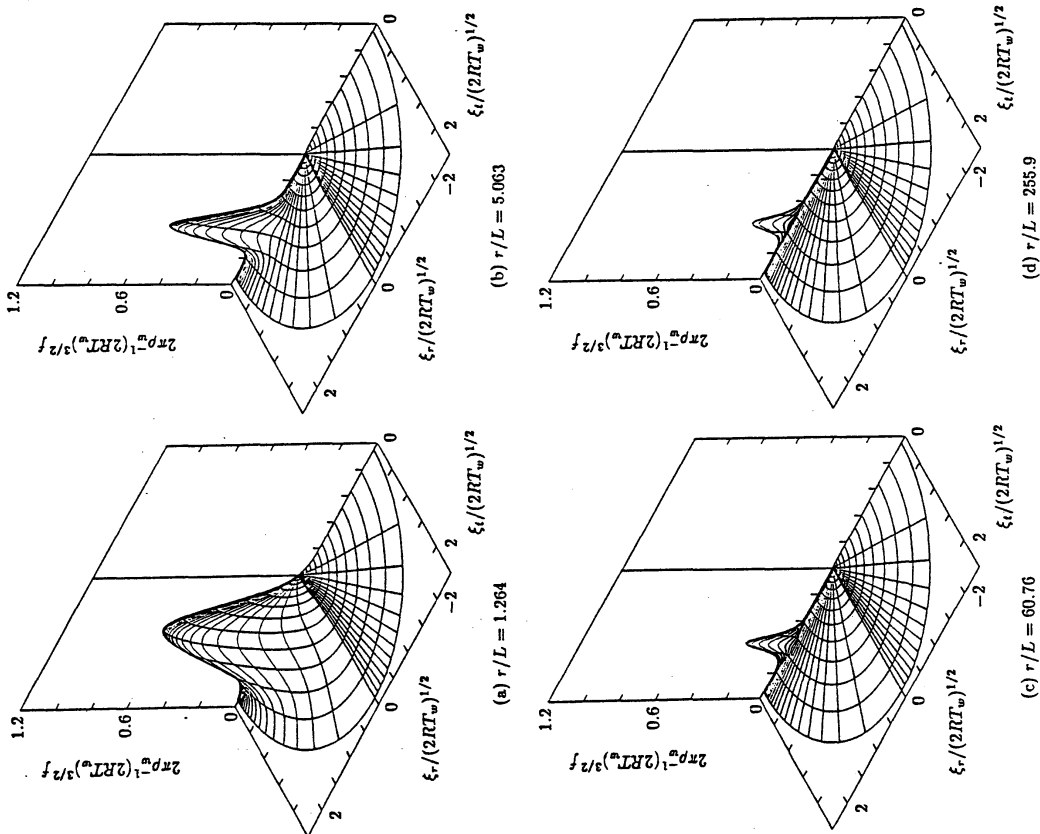
FIG. 7. The nondimensional velocity distribution function 2\pi\rho_w^{-1}(2RT_w)^{3/2}f at Kn_w = 0.01 (II): the continuum, transition, and free molecular regions. (a) r/L = 1.264 , (b) r/L = 5.063 , (c) r/L = 60.76 , and (d) r/L = 255.9 .
