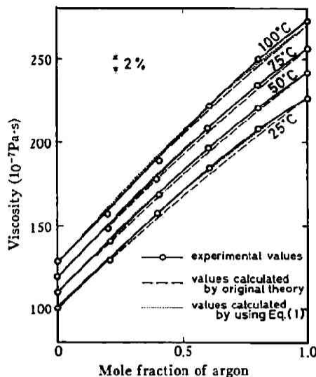
Fig. 4 Comparison of experimental value with original theoretical one and calculated one using Eq. (1) in argon-ammonia system
