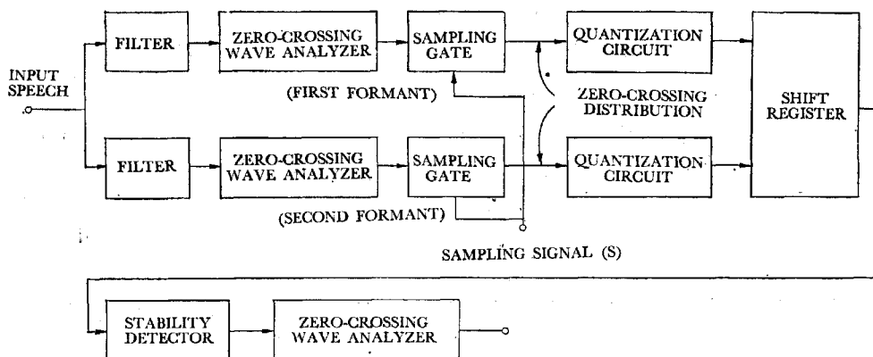
Fig. 2 Block diagram of vowel segmentation part.
