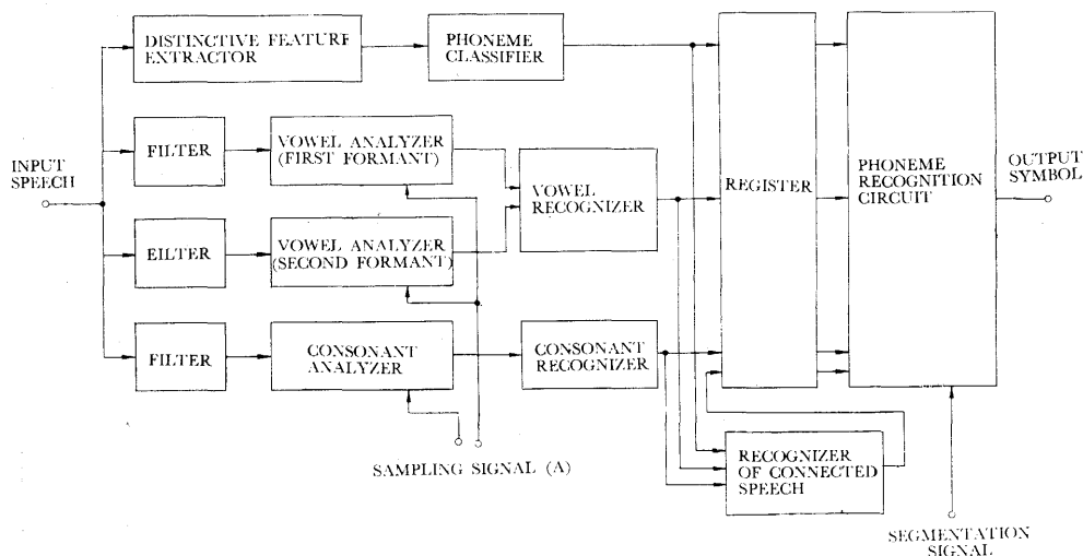
Fig. 7 Block diagram of recognition part.
