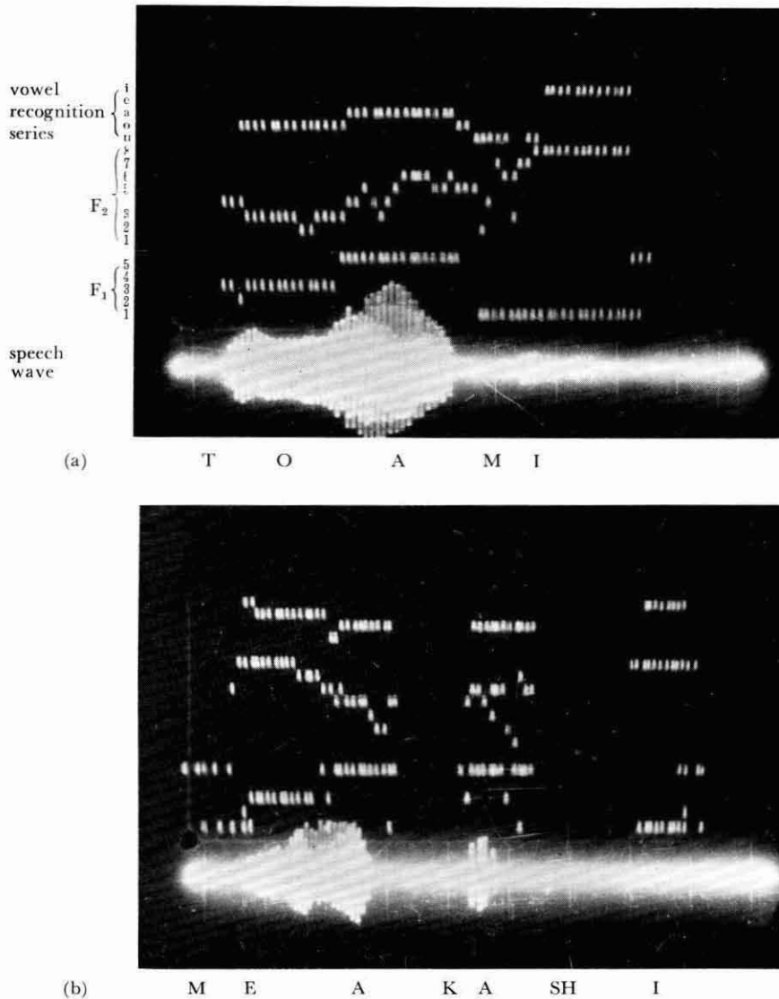
Fig. 4 Zero-crossing time pattern of F_1 and F_2 region sampled each 10 ms, ( T=10\text{ms} ), and instantaneous vowel recognition series. (Speech samples are taken from Japanese words)
