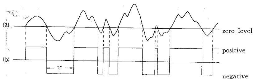
Fig. 3 Examples of (a) original speech wave. (b) zero-crossing wave.
