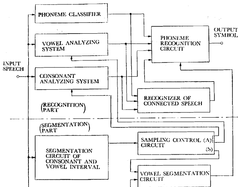
Fig. 1 Block diagram of phonetic typewriter.
