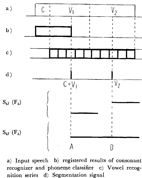
Fig. 8 Time chart of the operation in the phoneme recognition circuit.
