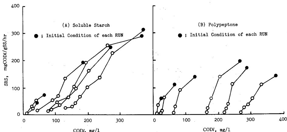
Fig. 4. Relationship between specific rate of substrate uptake (SRS) and CODI.
