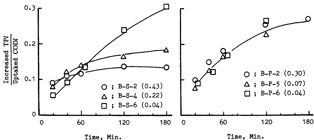
Fig. 8. Effect of substrate concentration on \Delta TPI / \Delta COD .
