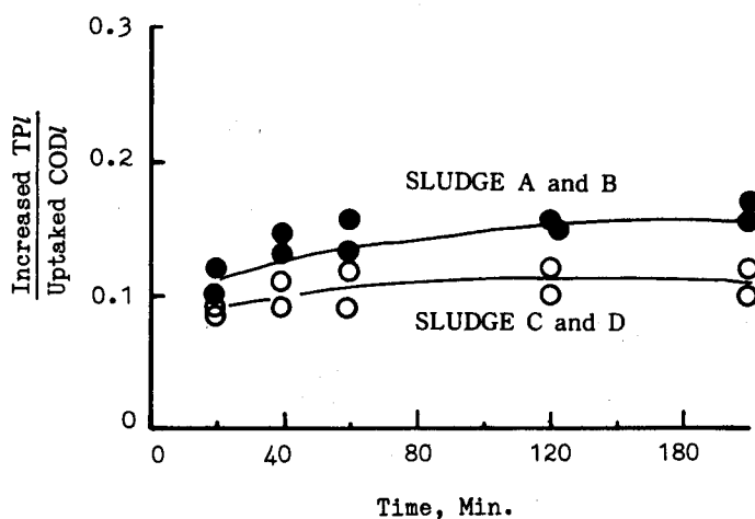
Fig.10. Effect of sludge sort on \Delta TPI/\Delta CODI .
