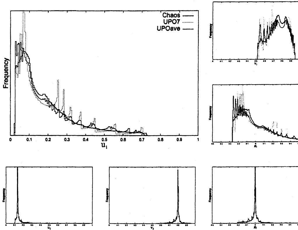
Fig. 4: Histograms of Chaos , UPO 7 , and UPO ave
