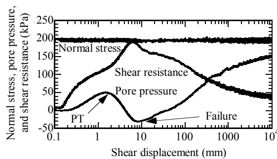
Fig. 7: (a) stress path (b) stress versus displacement of silica sand specimen with D_r = 50\% illustrating inequality between pore pressure and shear resistance at failure
