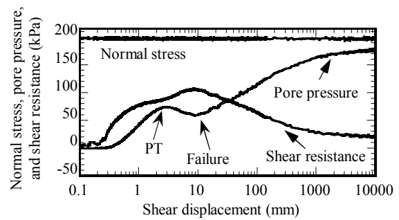
Fig. 6: behavior of a silica sand specimen with Dr = 44\% (a) stress path (b) stress versus displacement
