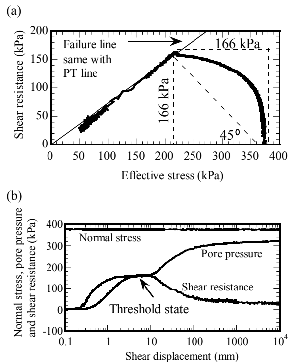
Fig. 5 (a) Stress path (b) Pore pressure and shear resistance behavior in a Takarazuka specimen
