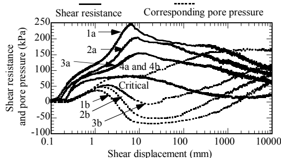
Fig. 8 Shear resistances and the corresponding pore pressures of some sands as density changes (specimens at 196 kPa confining stress)
