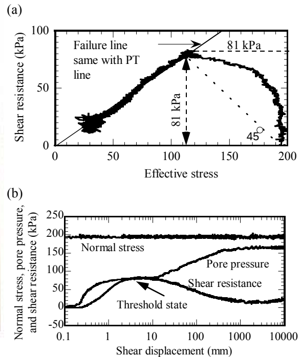
Fig. 4 (a) Stress path showing a threshold condition (b) Pore pressure and shear resistance behavior in a silica sand specimen
