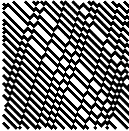
Figure 11. A nonequilibrium steady state without energy flow. Parameter values are (\alpha, \beta, \gamma, \delta) = (0.8, 0.2, 0.1875, 0.75) , e^{1/T_L} = 4.0 , and e^{-1/T_R} = 0.25 .
