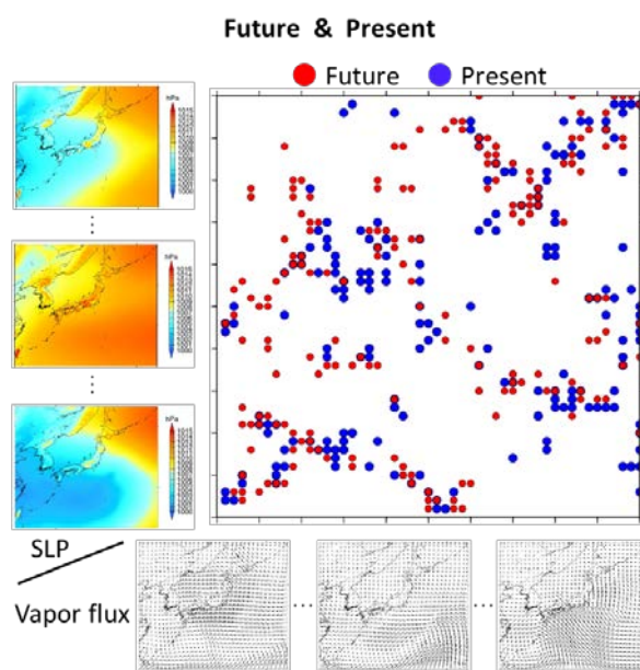
Fig.13 Combination of SOM maps. The X axis corresponds a SOM map of vapor flux, and Y axis corresponds a SOM map of SLP. The red (blue) plots shows future (present) climate data.
