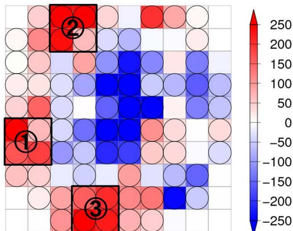
Fig.5 The difference of the number of d4PDF60 data plotted on each node (Future - Present). The nodes in warm (cold) color indicate the increase in future (present) climate. The nodes with ○ have 5% significant differences (Nakakita et al., 2016).
