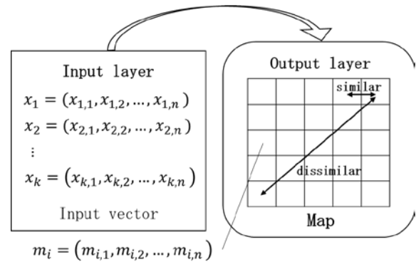
Fig.3 Input layer(left) and output layer(right) of SOM. m_i ( i=1,2,\dots,l ) are reference vectors, x_j ( j=1,2,\dots,k ) are input vectors, l is the number of the SOM map nodes, k is the number of input vectors, and n is the dimension of input vectors.
