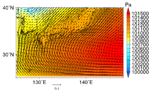
Fig.6 One of the atmospheric patterns at cluster three of Fig.4.3. SLP (shading; Pa) and vapor flux at surface (vector; \text{kgkg}^{-1}\text{ms}^{-1} ) (Nakakita et al., 2016).
