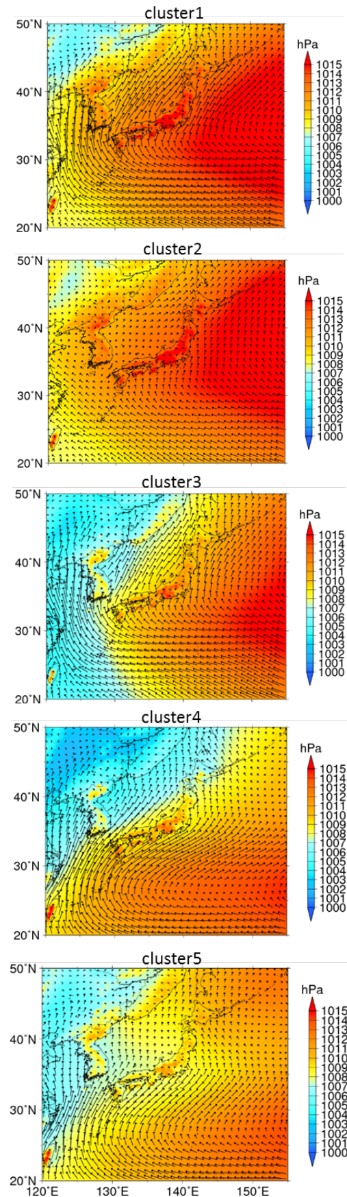
Fig.17 One of the atmospheric patterns at cluster①~⑤ from top to bottom. SLP (shading; hPa) and vapor flux (vector; \text{kg kg}^{-1} \text{ms}^{-1} ).
