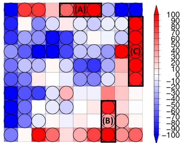
Fig.7 The difference of the number of d4PDF20 data plotted on each node (Future - Present). The nodes in warm (cold) color indicate the increase in future (present) climate. The nodes with ○ have 5% significant differences.
