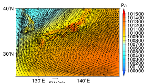
Fig.8 One of the atmospheric patterns at cluster C of Fig.4.5. SLP (shading; Pa) and precipitable water flux (vector; \text{kgms}^{-1} ).
