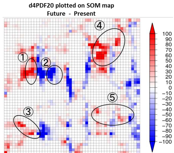
Fig.16 The difference of the number of d4PDF20 data plotted on each SOM nodes (Future - Present). The nodes in warm (cold) color shows the increase in future (present) climate. The number of ①~⑤ correspond the numbers of Fig.5.5.
