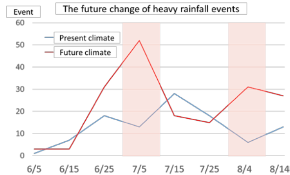
Fig.2 The future change of the frequency of heavy rainfall events in Baiu season from SOUSEI RCM05 data. The red zone means 5% significant increasing.
