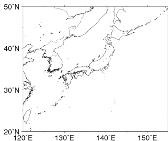
Fig.12 Calculation area of improved SOM.
