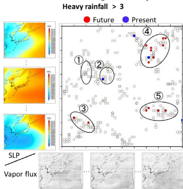
Fig.15 Only the data which have more than three heavy rainfall events are colored on Fig.5.4 SOM map.
