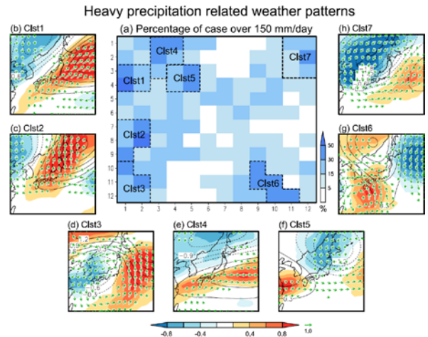
Fig.4 (a) Frequency (percentage) of days for maximum local precipitation to exceed 150mm/day at each node. The black dashed lines denote the seven clusters of SOM nodes that are most strongly associated with heavy rainfall. (b)-(h) Examples of patterns in the seven clusters extracted from the 12×12 SOM nonlinear classification as heavy precipitation-related weather pattern. Daily-mean 850-hPa EPT (red and blue shading), 200-hPa GH (black contour), and 850-hPa wind (green vectors) anomalies for June-July during 1958-2011 (Ohba et al., 2014).
