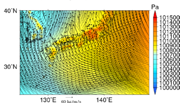
Fig.9 One of the atmospheric patterns at cluster A of Fig.4.5. SLP (shading; Pa) and precipitable water flux (vector; \text{kgms}^{-1} ).
