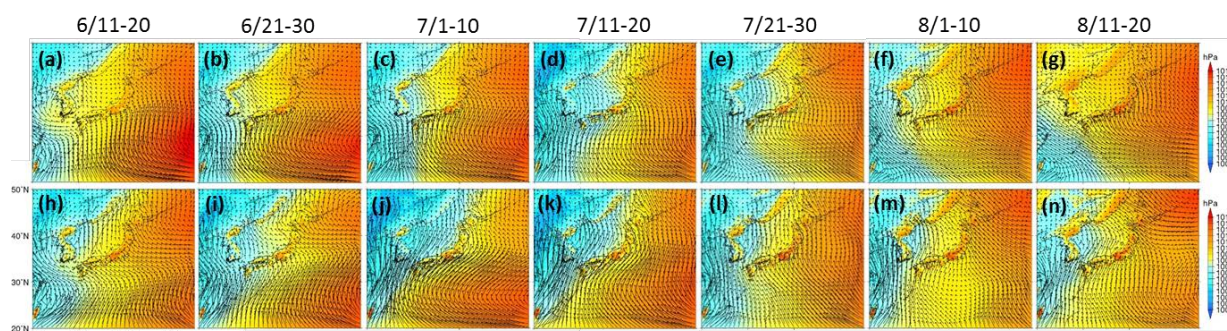
Fig.19 SLP (shading; hPa) and vapor flux (vector; \text{kgkg}^{-1}\text{ms}^{-1} ) for the periods (a) 11-20 June, (b) 21-30 June, (c) 1-10 July, (d) 11-20 July, (e) 21-30 July, (f) 1-10 August, (g) 11-20 August averaged over 25 years of the present climate experiments (1979-2003) of SOUSEI AGCM20. (h)-(n): Same as (a)-(g) but averaged over 25 years of the future climate experiments (2075-2099).
