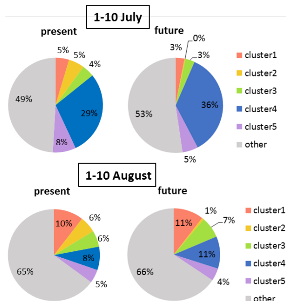
Fig.18 The percentage about which clusters on SOM map the data for the beginning of July and August of d4PDF20 are calssified into. There are 6 categories, cluster 1~5 and other nodes, upper shows 1-10 July, below shows 1-10 August. Left shows present and right shows future climate.
