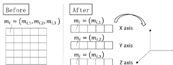
Fig.10 Left shows a standard 2 dimensional SOM map, and right shows 1 dimensional SOM map each variables after improved, in case the number of variables for SOM is three.
