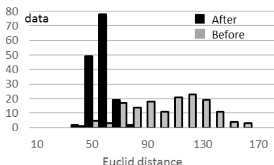
Fig.11 The comparison of Euclid distances which are calculated when the input data are classified on a SOM node with SOM method before improved and after improved.
