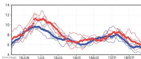
Fig.1 The blue (red) lines show the daily precipitation in present (future) climate calculated by KAKUSHIN AGCM60 ensembles and the dot lines show average of ensembles (Kanada et al., 2012).
