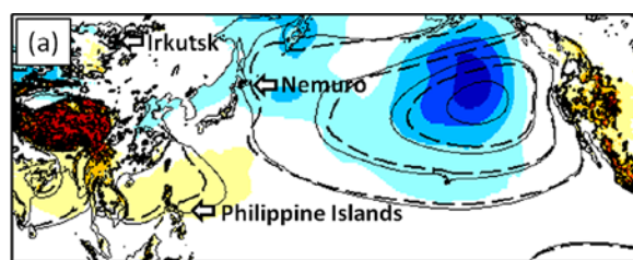
Fig.20 The difference of sea level pressure between the present and future climate (shading) in August derived by AGCM20. Solid and dash contours are sea level pressure in the present and future climate respectively (Hanafusa et al., 2013).
