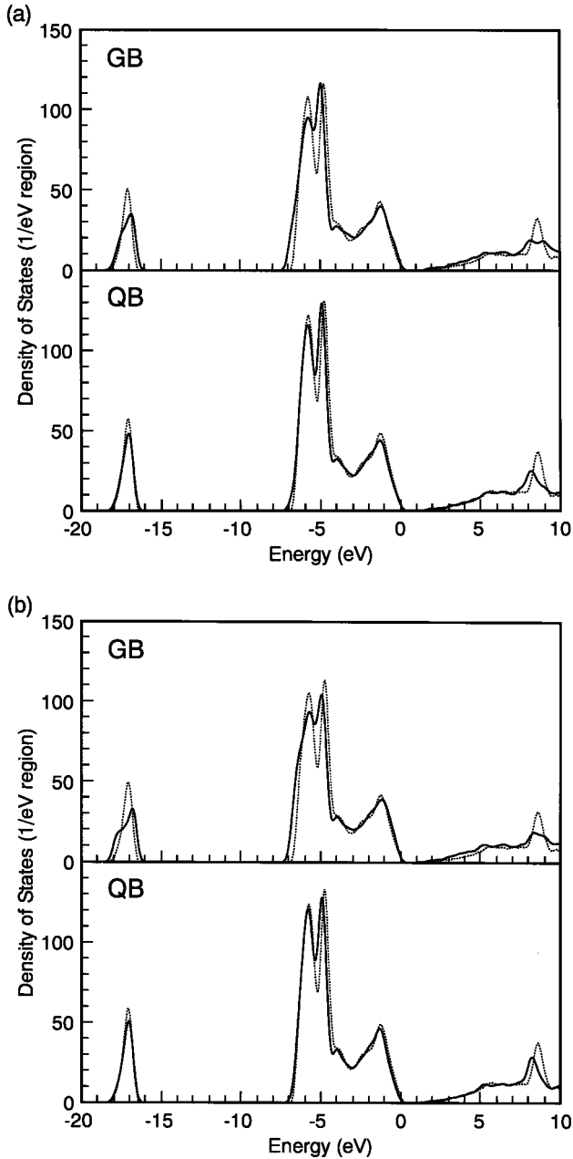
FIG. 4. Local density of states (LDOS) for the supercells of (a) boundary A and (b) boundary B. The upper and the lower show the LDOS's in the grain-boundary (GB) and quasibulk (QB) regions, respectively. The DOS for the bulk primitive cell is also shown with dotted curves, which is normalized by the number of atoms in each region. The top of the valence band for the bulk primitive cell is chosen as 0 eV. The LDOS's for the boundary supercells are shifted to align the average of the lower valence band in the quasibulk region with that for the bulk primitive cell.
