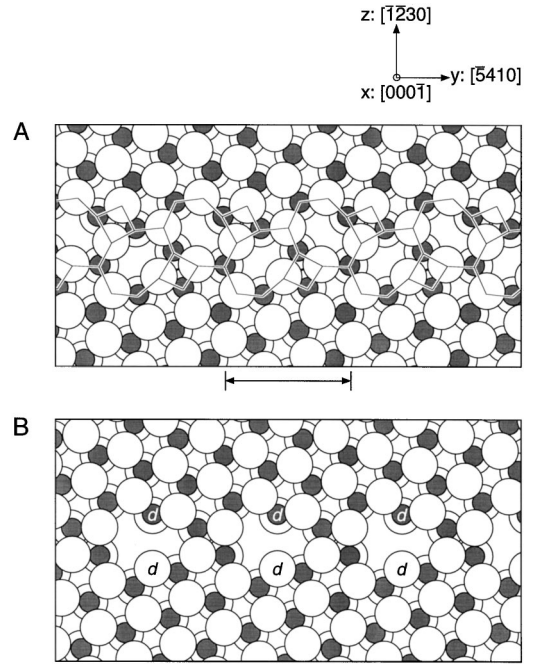
FIG. 1. Equilibrium boundary geometries calculated by the empirical method. The scale indicates the periodicity unit of the boundary. The filled and open circles denote Zn and O atoms, respectively. In the [0001] view, three of the four basal planes in the ZnO unit cell can be seen in the order of O-Zn-O. For the boundary A, core structure is described as a sequence of fourfold- and eightfold-coordinated channels. For the boundary B, atoms possessing dangling bonds are labeled with d .
