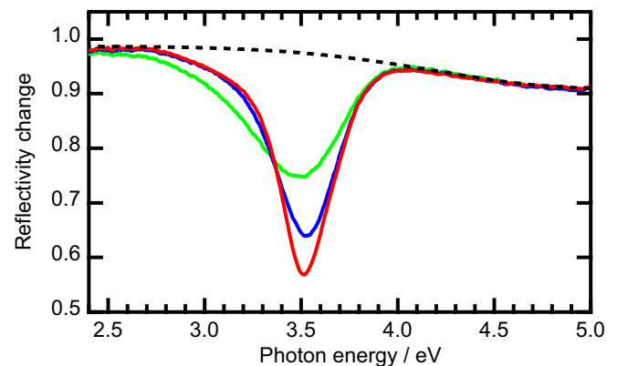
FIG. 16. (Solid curves) some of the original data of the reflectivity change depicted in Fig. 6. (Dashed curve) A Gaussian function obtained by fitting the background component of the spectra.
