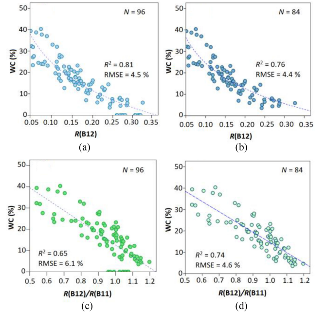
Fig. 5. Correlation between WC and (a) the simulated reflectance at S2A band 12, (b) R(B12) excluding WC = 0 % data, (c) reflectance ratio of B12 versus band 11, R(B12)/R(B11) , and (d) R(B12)/R(B11) excluding WC = 0 % data. The best regression curves of negative logarithmic [(a) and (b)] or linear [(c) and (d)] functions are overlaid on each graph. R^2 and RMSE denote the coefficient of determination and root-mean-squares error, respectively.
