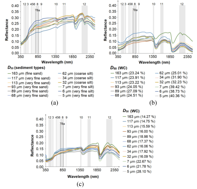
Fig. 7. Reflectance spectra of the initial 12 samples with different D_{50} under three WC conditions with S2A bands. (a) Fully dry ( WC = 0\% ). (b) Half-saturated (almost half the WC of full saturation). (c) Fully saturated.
