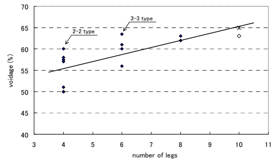
Fig.11 Relationship between number of legs and voidage
