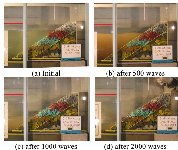
Photo 2. Cross sectional view of blocks movement
