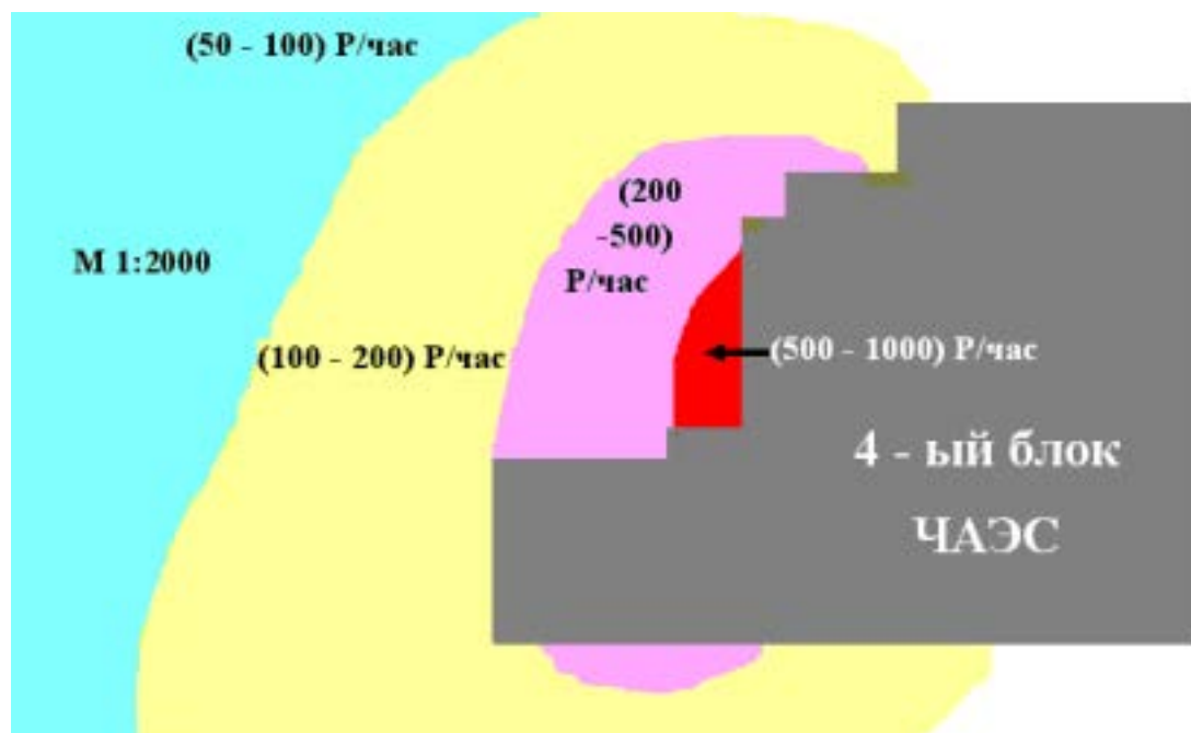
Fig. 3. The radiation situation on the CHNPP Unit-4 site at 26.04.1986 ( P/\text{час} = R/\text{hr} ).
