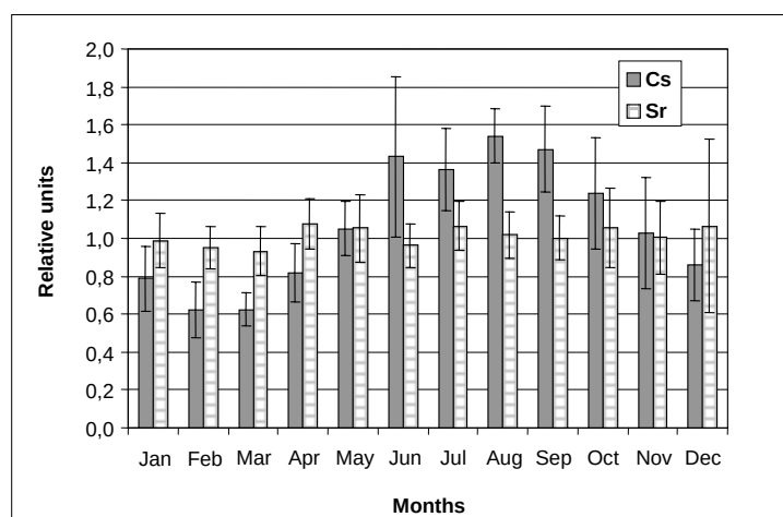
Fig. 5. Seasonal behaviour of total ^{137}\text{Cs} and ^{90}\text{Sr} in water of the Cooling Pond.
