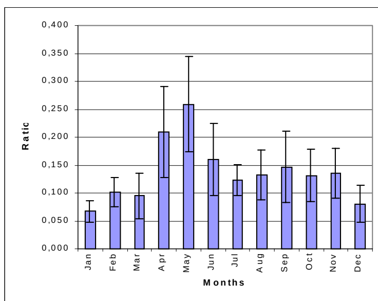
Fig. 6. Seasonal behaviour of ratio of suspended to total ^{137}\text{Cs} in water of the Cooling Pond.
