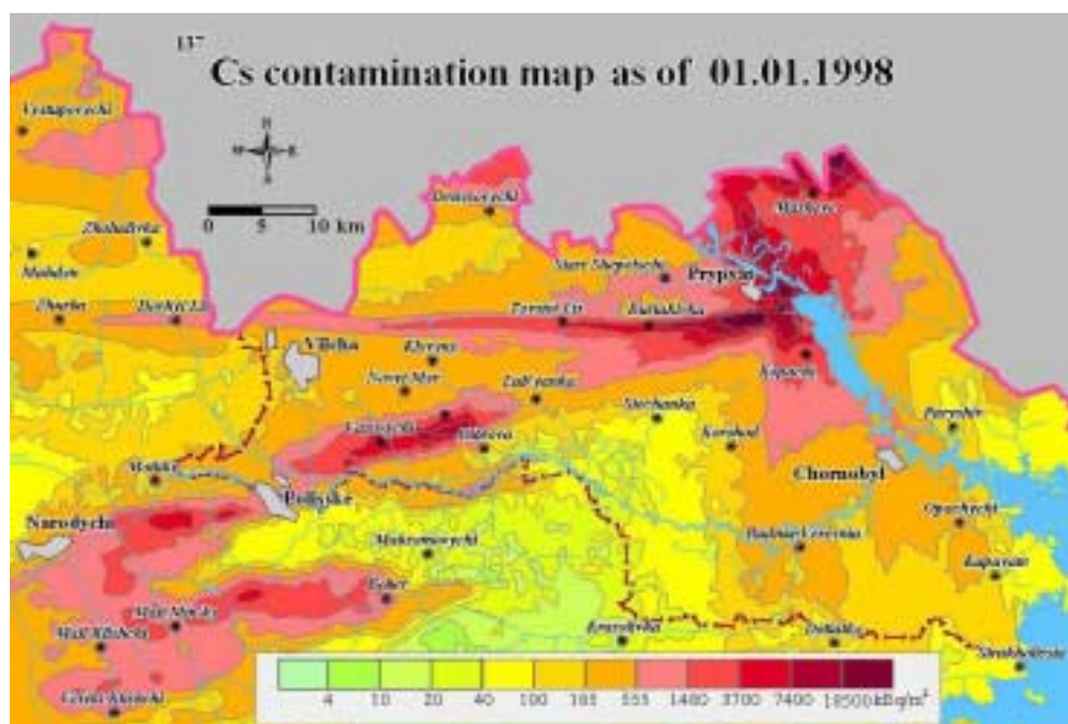
Fig. 4. ^{137}\text{Cs} contamination map of the adjacent territory to Chornobyl NPP (Ukrainian part).
