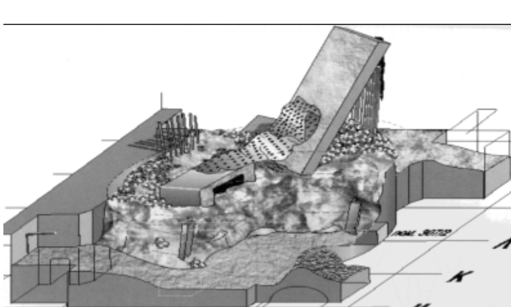
Fig.3 Computer model of the premise 305/2 and the reactor shaft.
