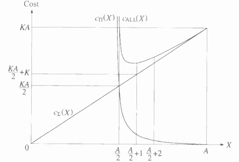
Figure 6.5: Behavior of cost functions.
