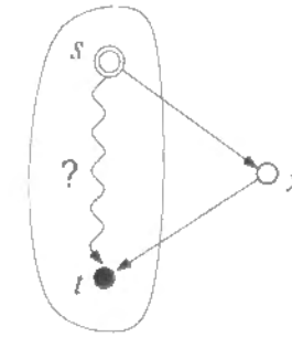
Figure 5.13: Proof of Lemma 5.13.
