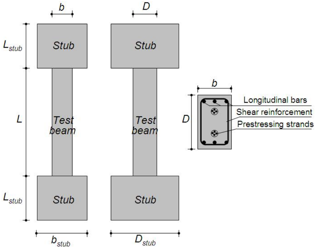
Fig. 3.1 Test specimens
