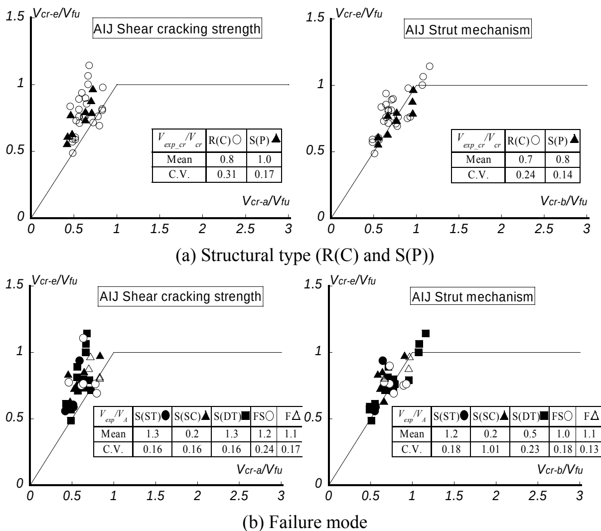
Fig. 3.39 Comparison between observed and analytical shear cracking strength
