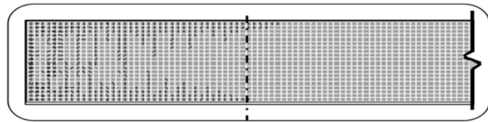
(b) No.2 (with round PT tendon, \rho_r=0.7\% )
