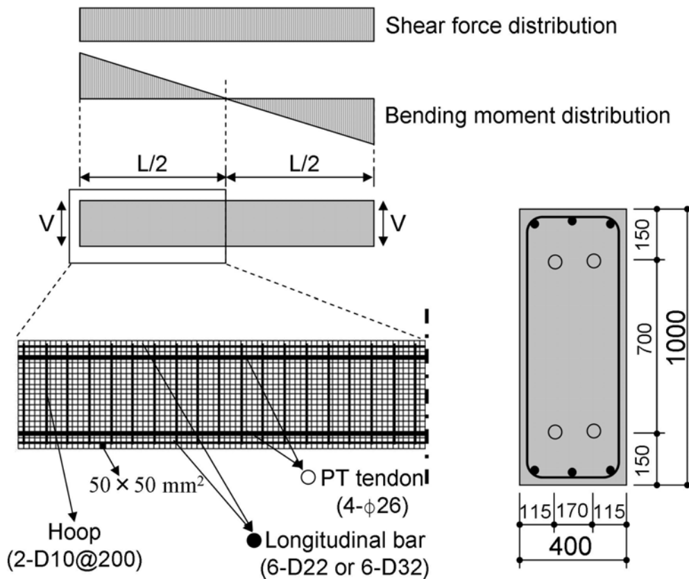
Fig. 7.9 Reinforcing detail
