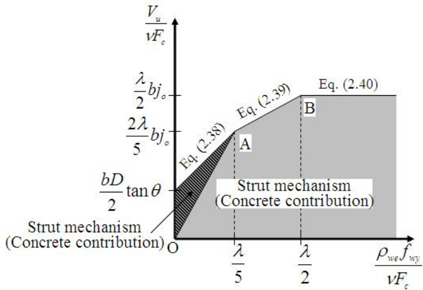
Fig. 2.10 Relationship between amount of shear reinforcement and shear strength by AIJ guide line [2.78]
