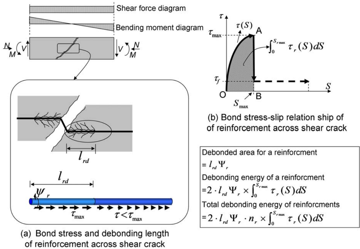
Fig. 5.6 Calculation method of debonding energy of reinforcement
