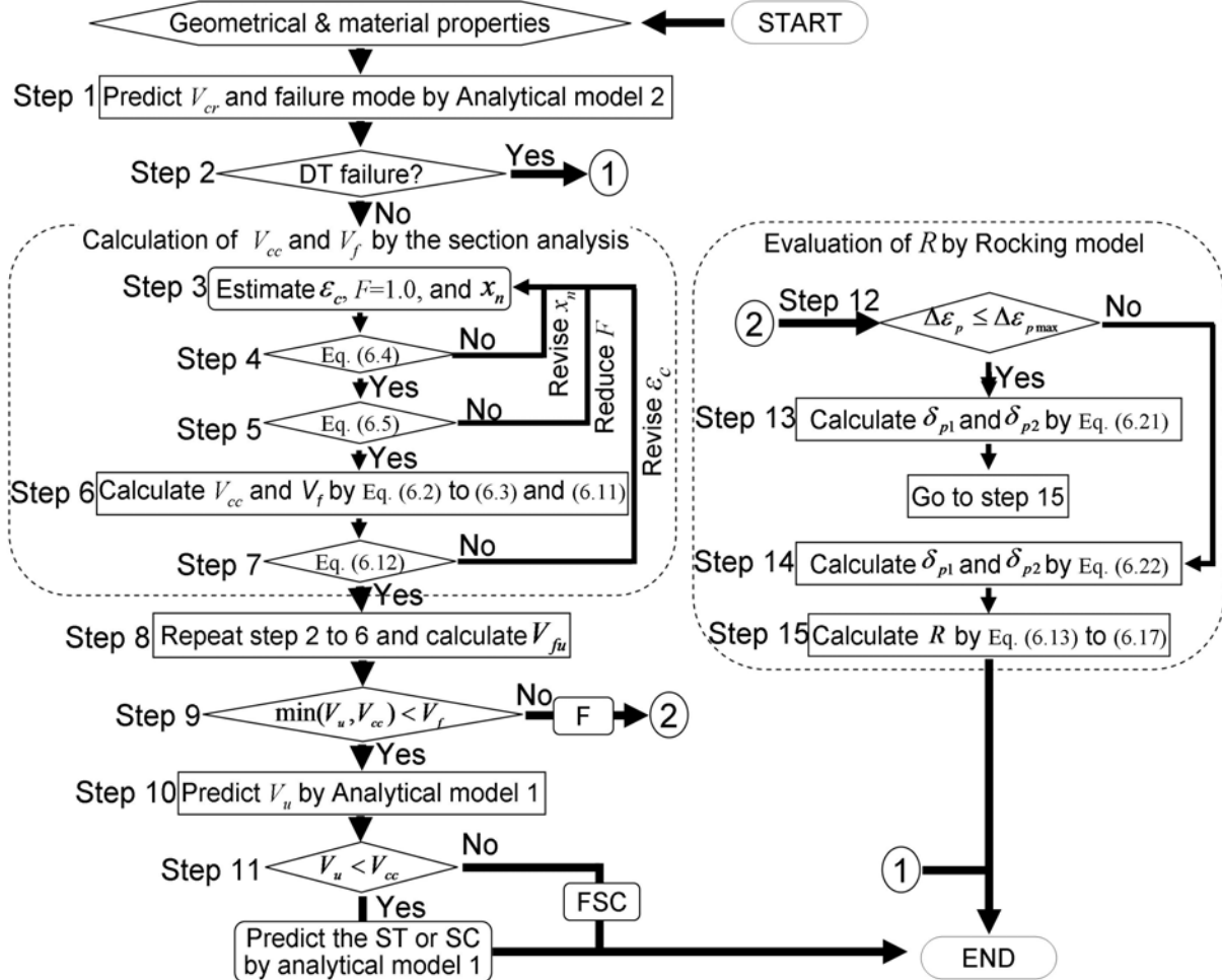
Fig. 6.8 Calculation procedure of proposed method.
