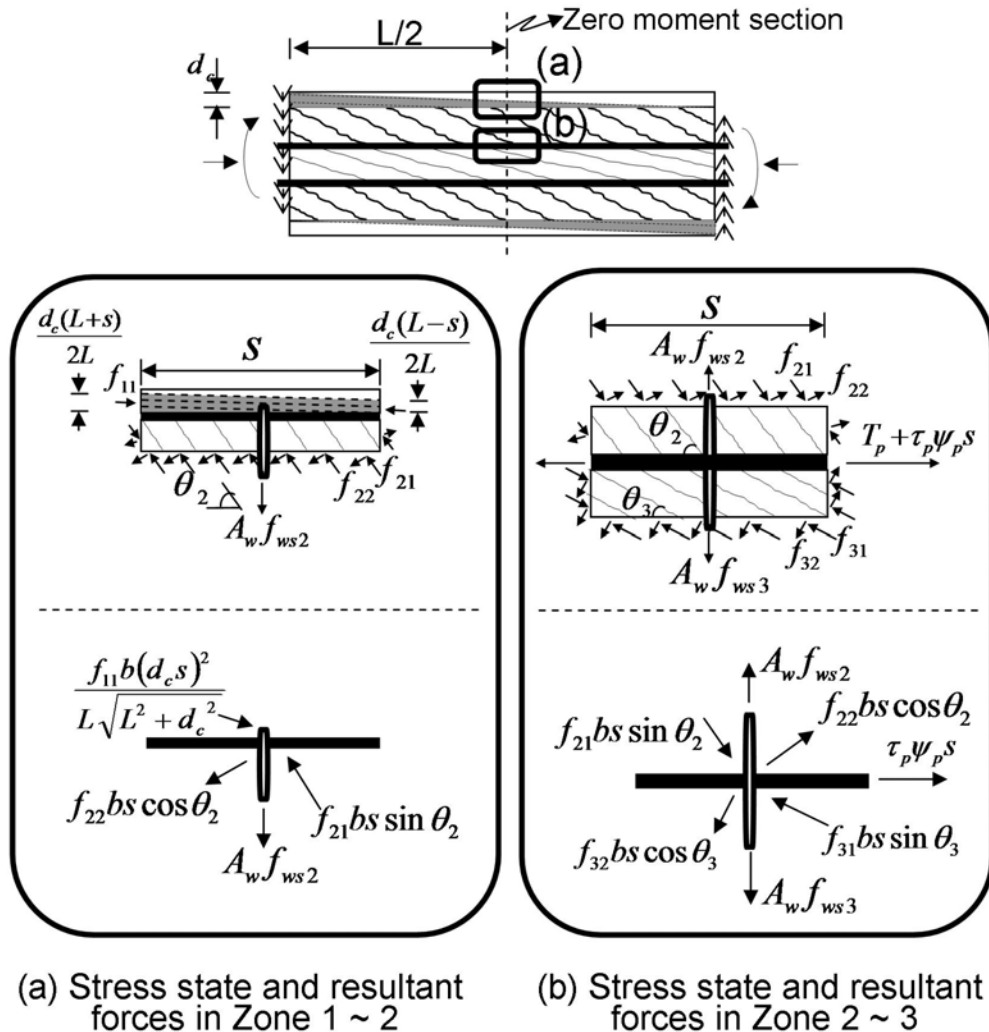
Fig. 4.4 Stress state and resultant force in each zone
