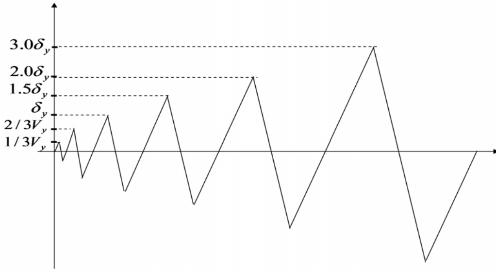
Fig. 7.11 Loading histories
