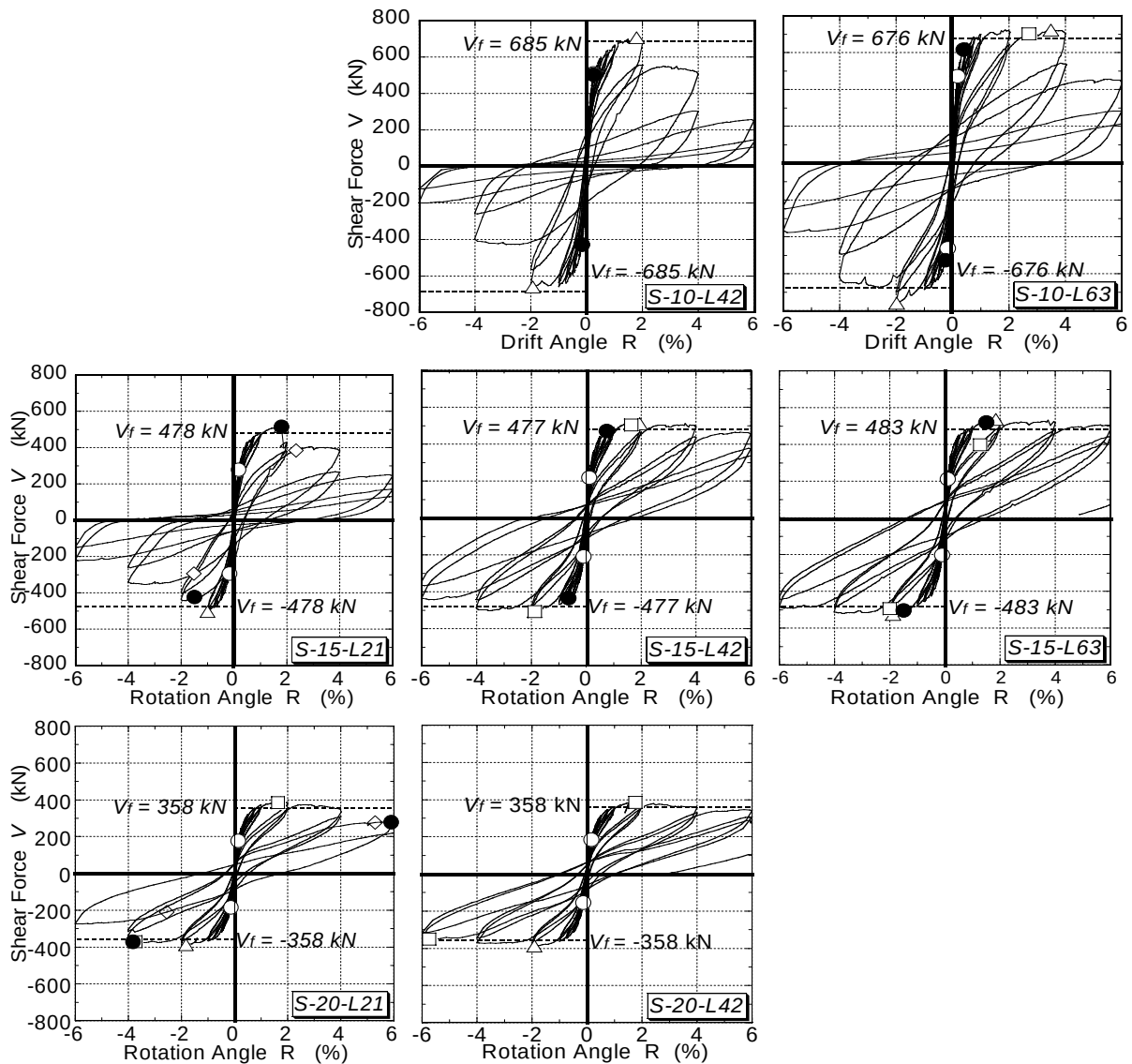
Fig. 3.12 Shear force, V – drift angle, R , relations
