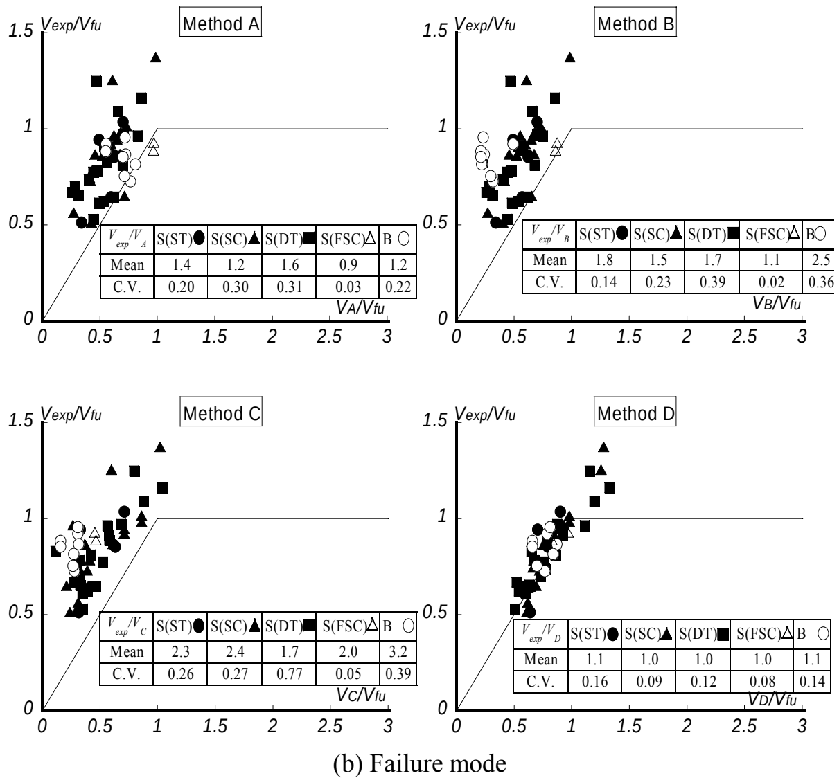
Fig. 3.40 Comparison between experimental and analytical shear strength
