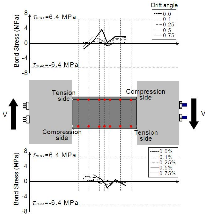
Fig. 3.36 Distribution of bond stress of non-prestressed longitudinal bar
