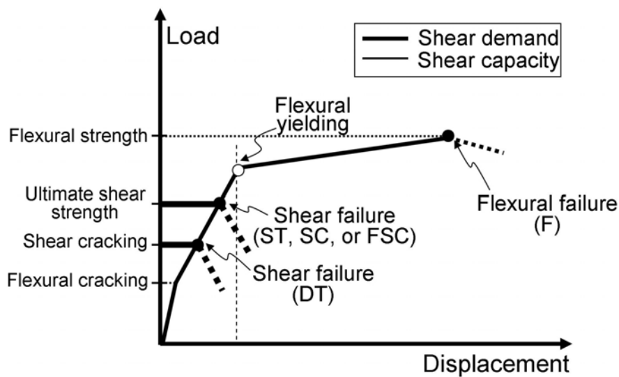
Fig. 6.2 Load-displacement relation and shear capacity
