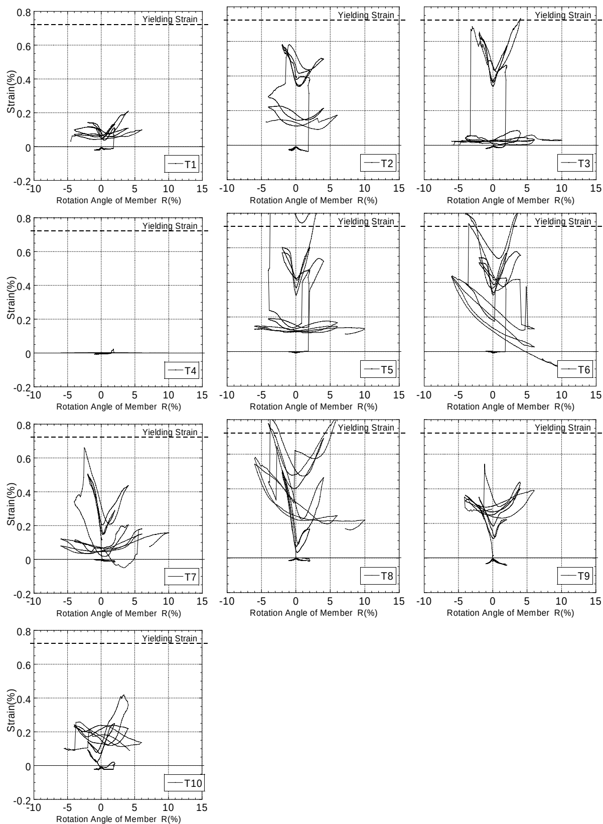
Fig. A.14 Strain distribution of shear reinforcements in Test 1
