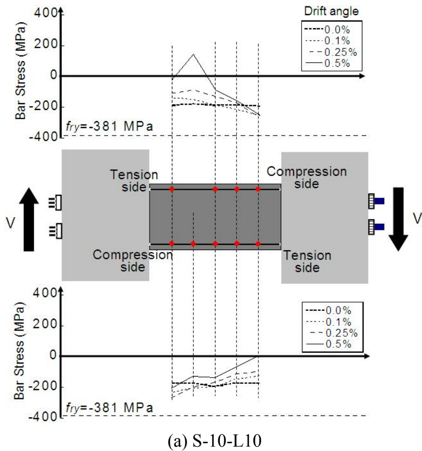
Fig. 3.33 Stress distribution of non-prestressed longitudinal bar
