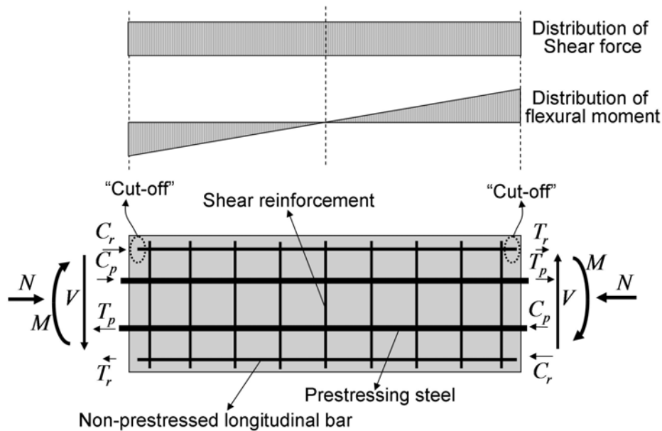
Fig. 4.1 Post-tensioned precast concrete member subjected to pure shear
