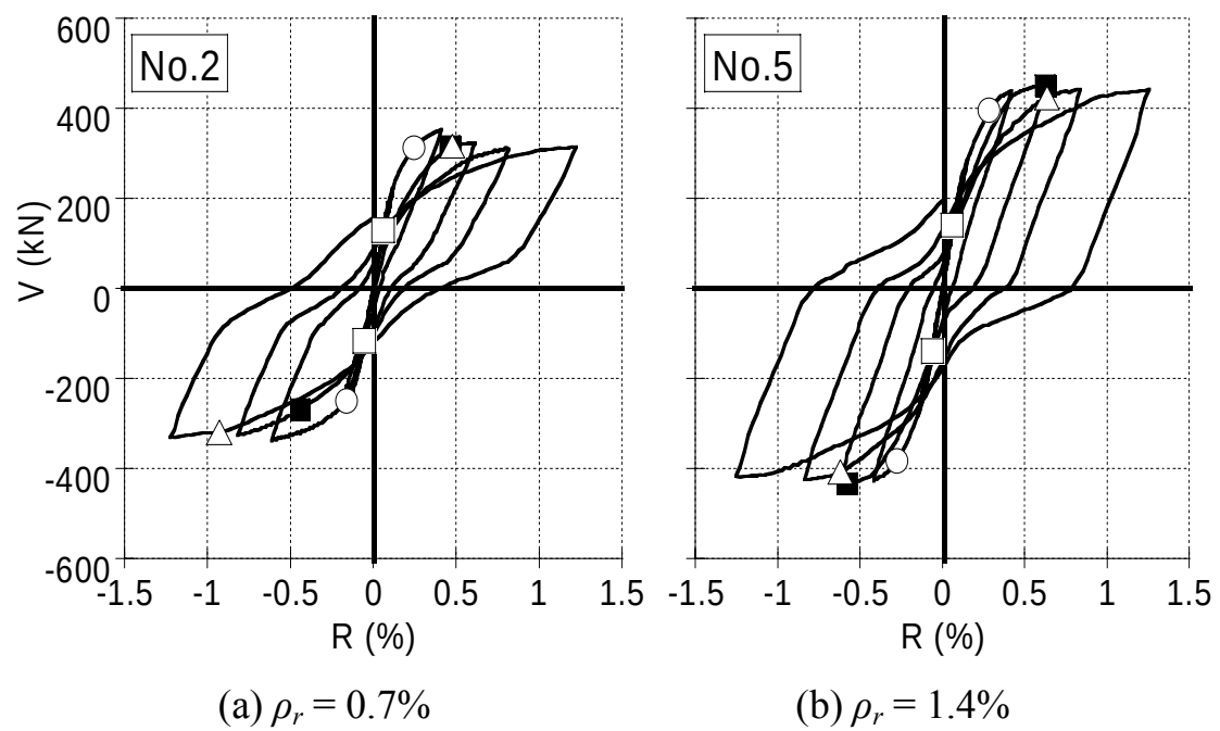
Fig. 7.13 Load-drift angle relation for the beams with bonded round bar
