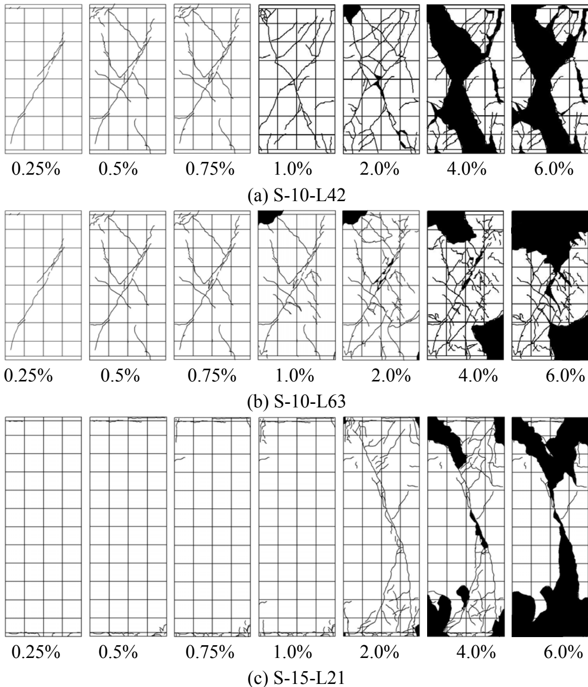
Fig. 3.13 Crack patterns
