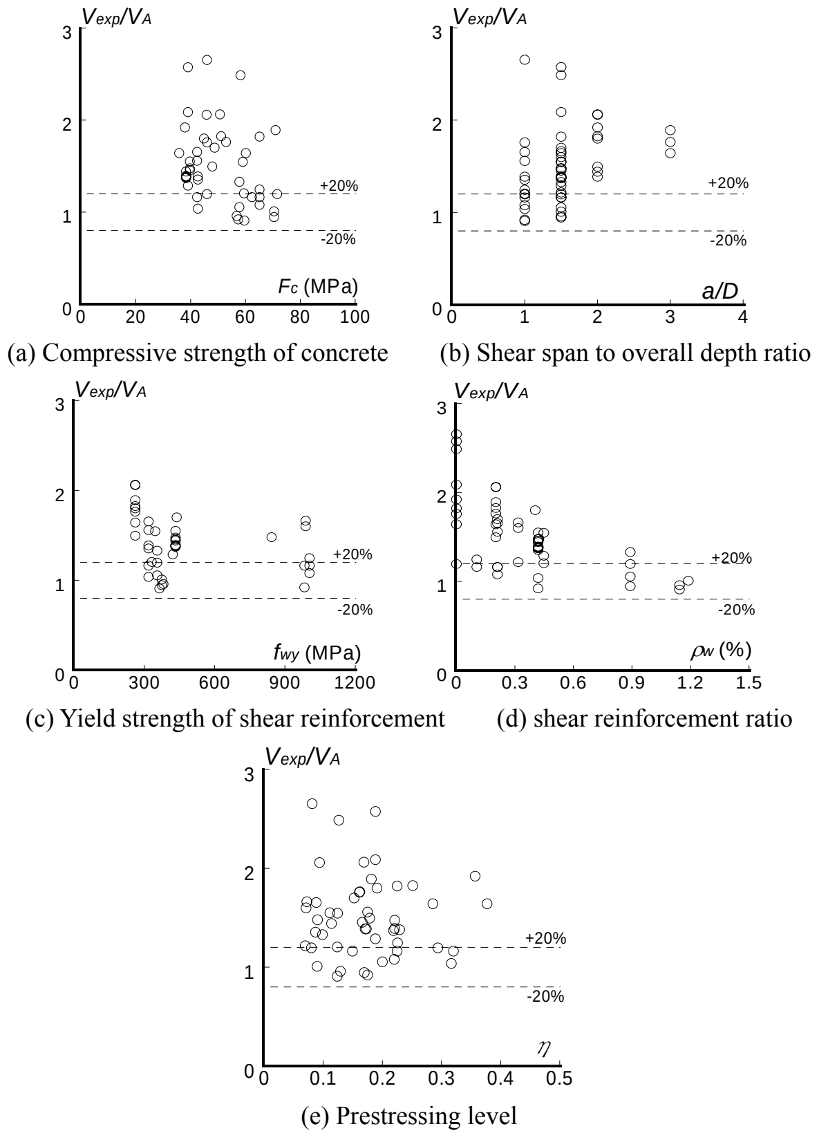
Fig. 3.41 Relationship between V_{exp}/V_A and experimental paramters
