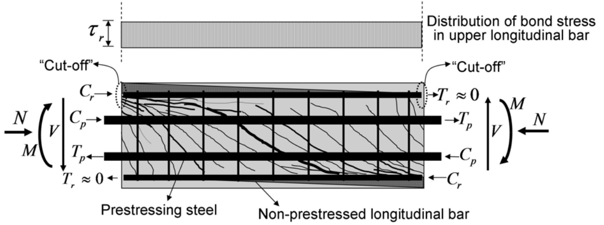
Fig. 4.3 Distribution of bond stress of upper non-prestressed longitudinal bar
