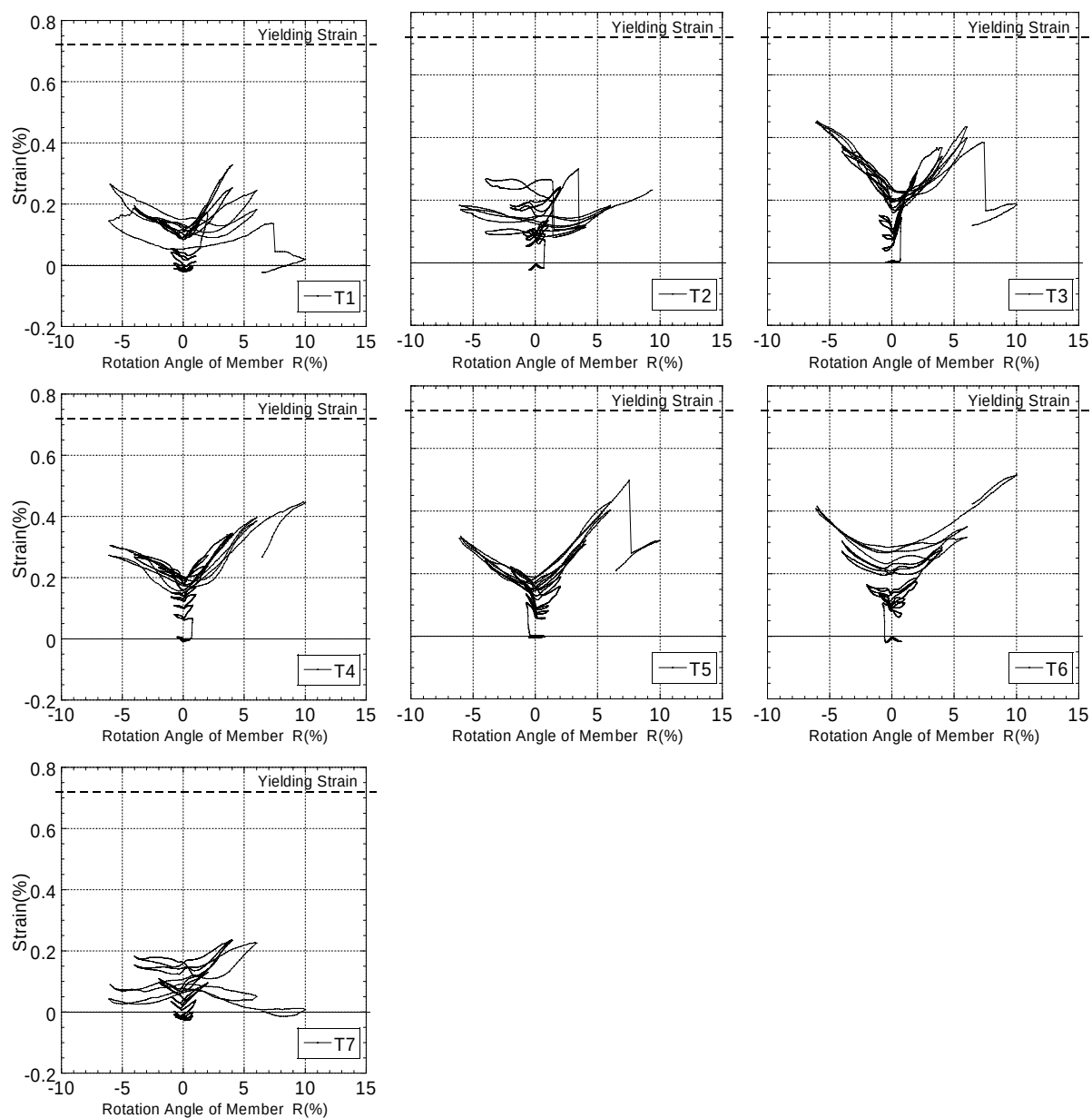
Fig. A.14 Strain distribution of shear reinforcements in Test 1
