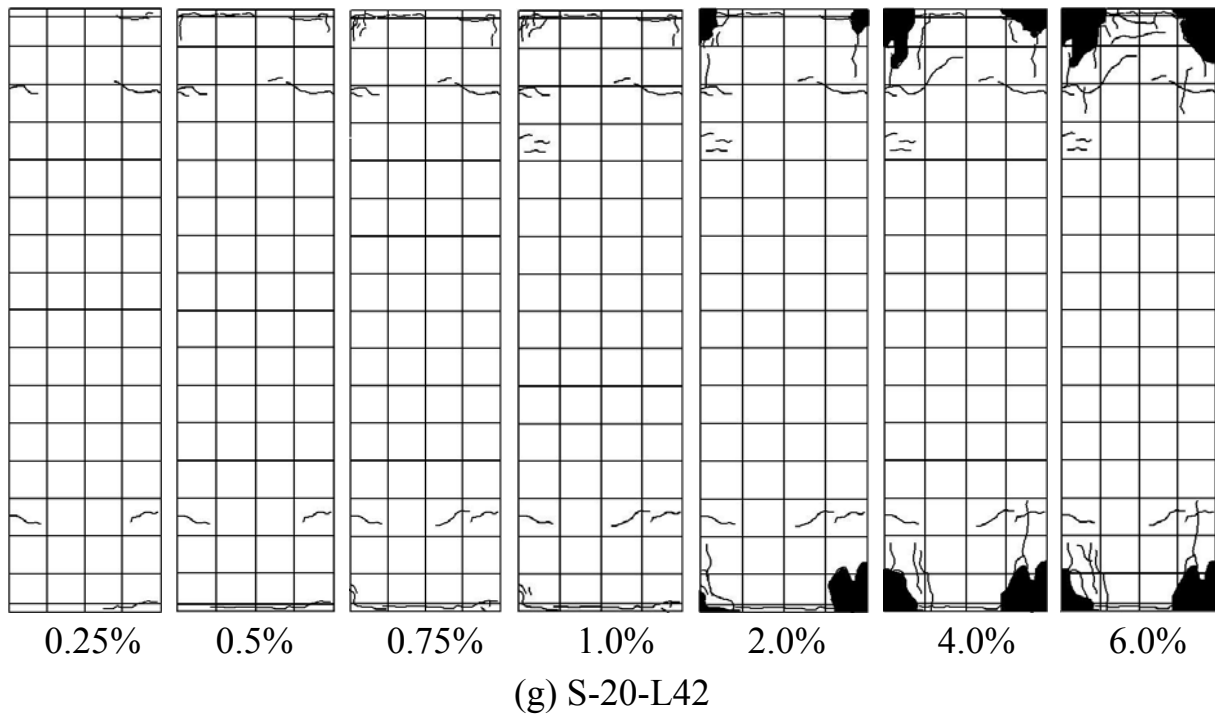
Fig. 3.13 Crack patterns
