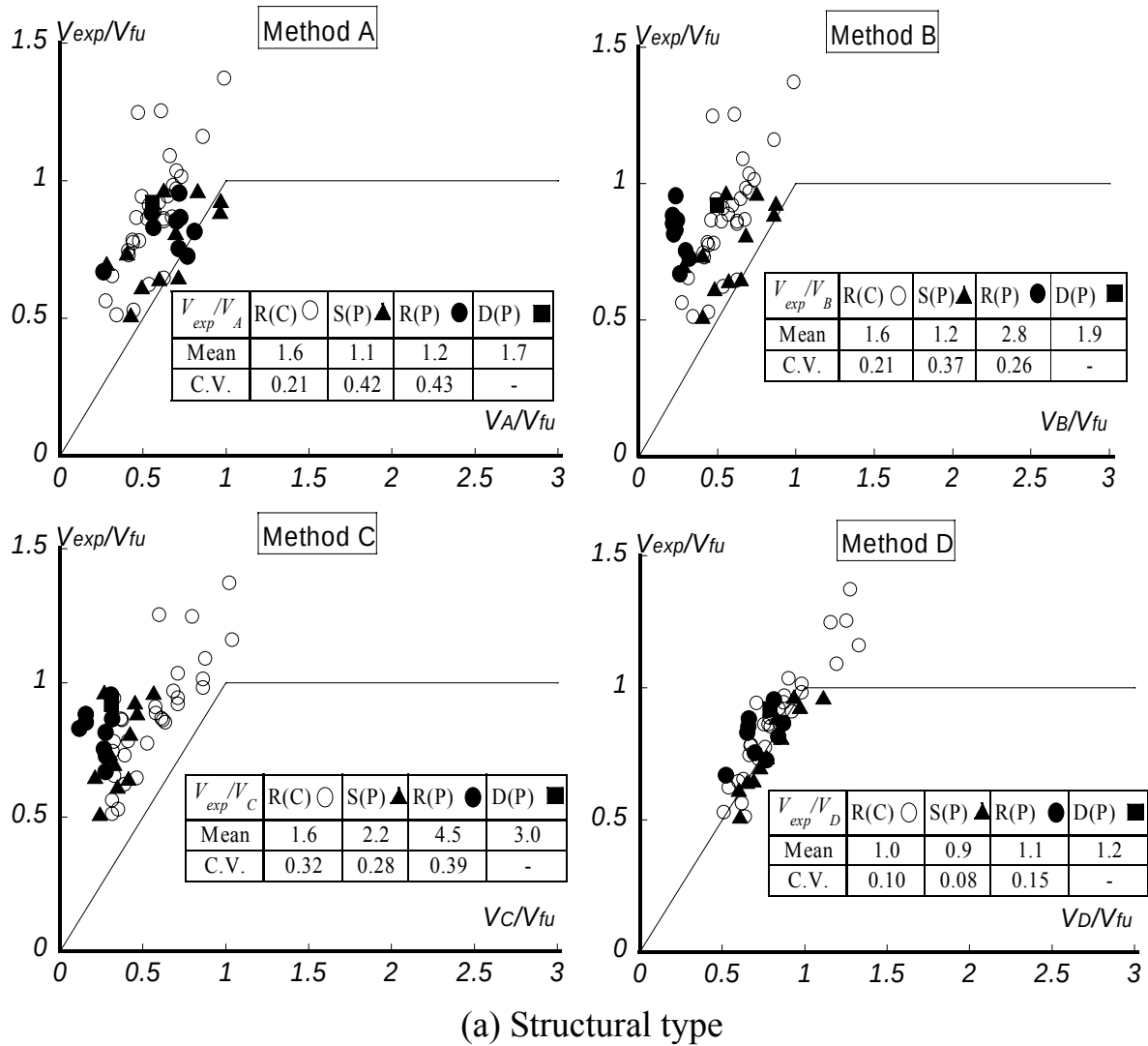
Fig. 3.40 Comparison between experimental and analytical shear strength
