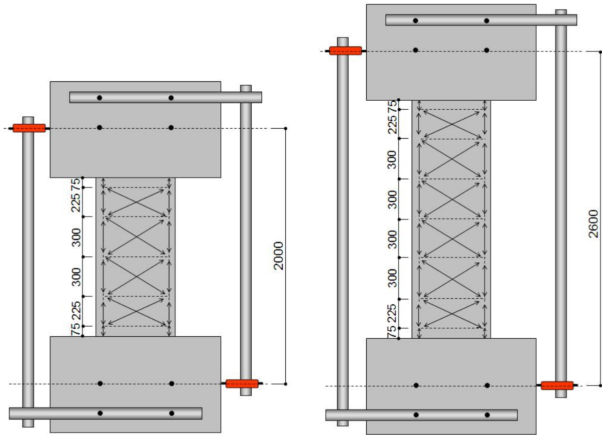
(a) Specimens with a/D=1.0
