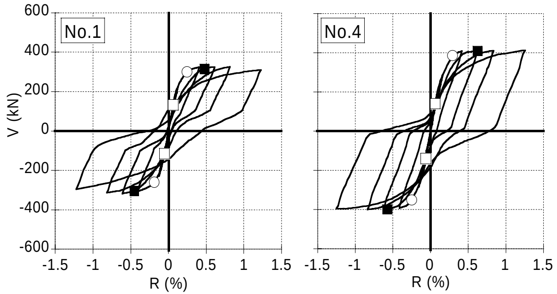
Fig. 7.12 Load-drift angle relation for the beams with unbonded tendon
