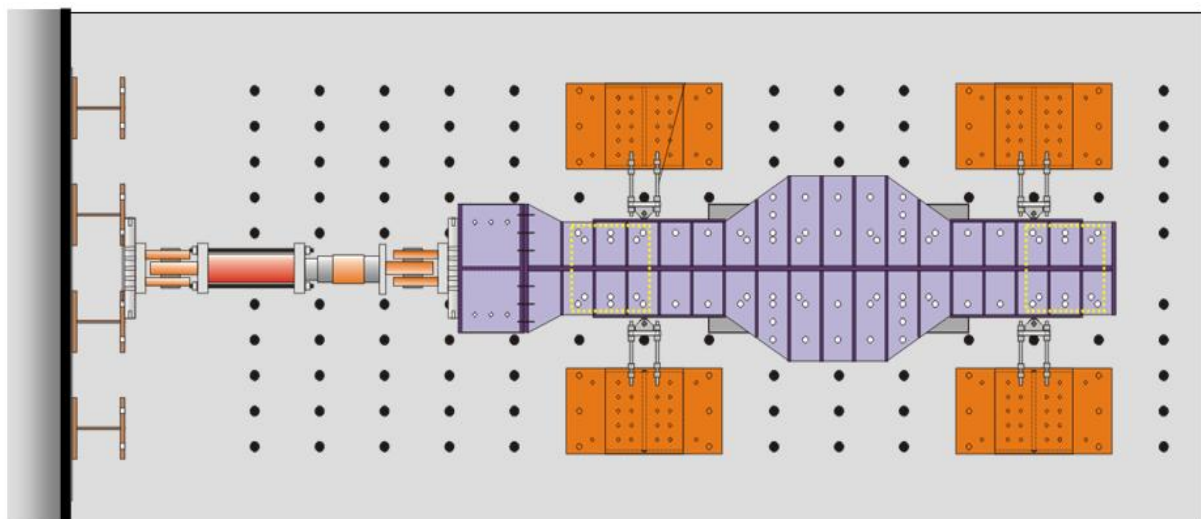
(b) Plan Fig. 3.8 Loading setup
