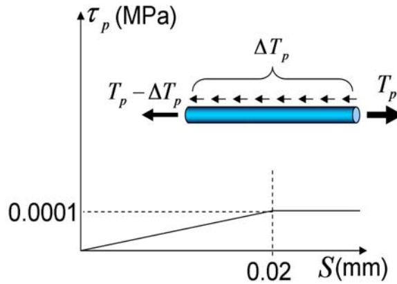
Fig. 7.5 Bond stress-slip relationship
