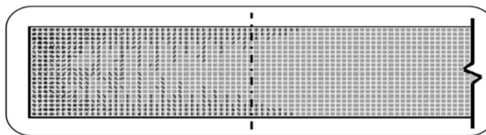
(c) No.3 (with deformed PT tendon, \rho_r=1.4\% )
