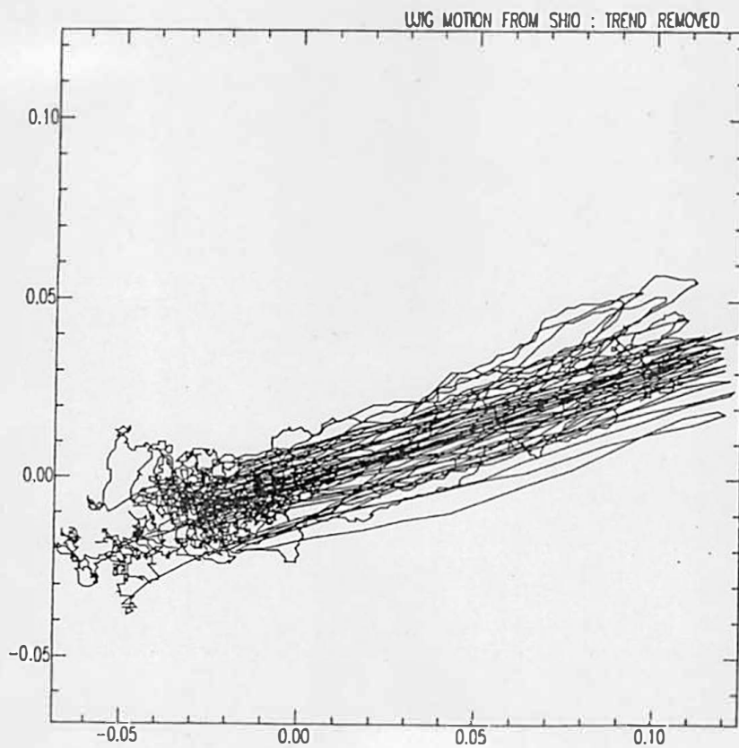
Fig.5 Enlarged plot of the first part of the experiment (upper) and the one for the linear trend removed (lower).
