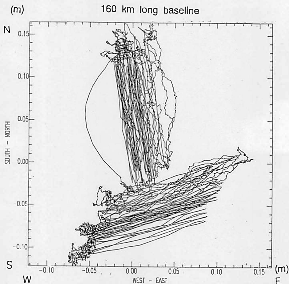
Fig.4 The same as Fig.2 but from the base site 160 km apart.
