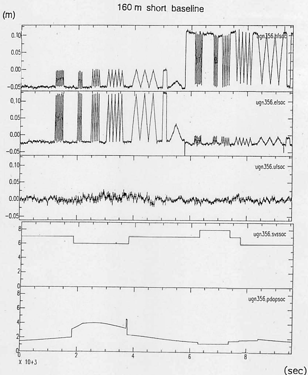
Fig.1 The rover motion determined from the base site 160 m apart. From the top to the bottom, are shown N-S, E-W and vertical components, and the number of satellites and PDOP.
