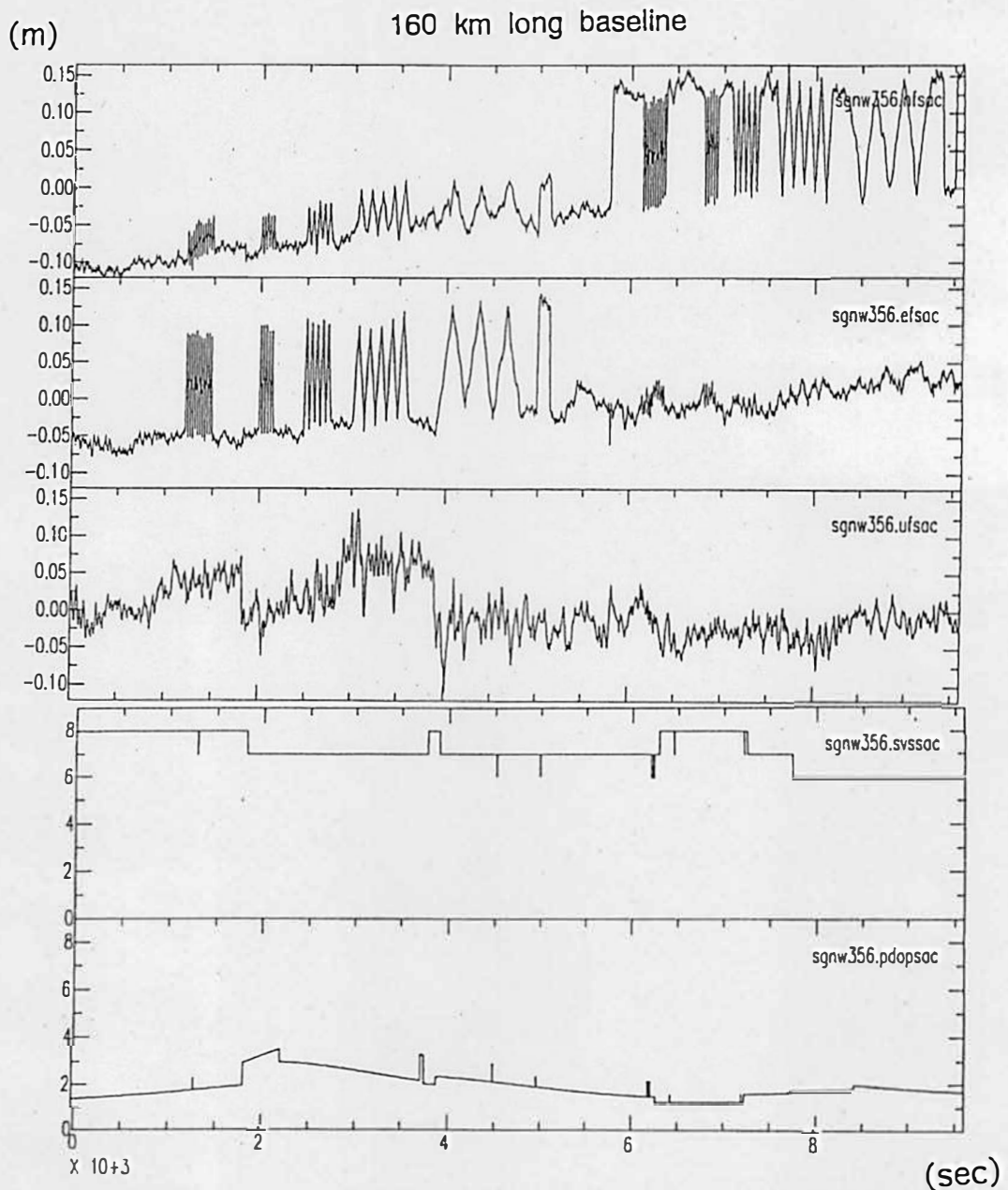
Fig.3 The same as Fig.1 but from the base site 160 km apart.
