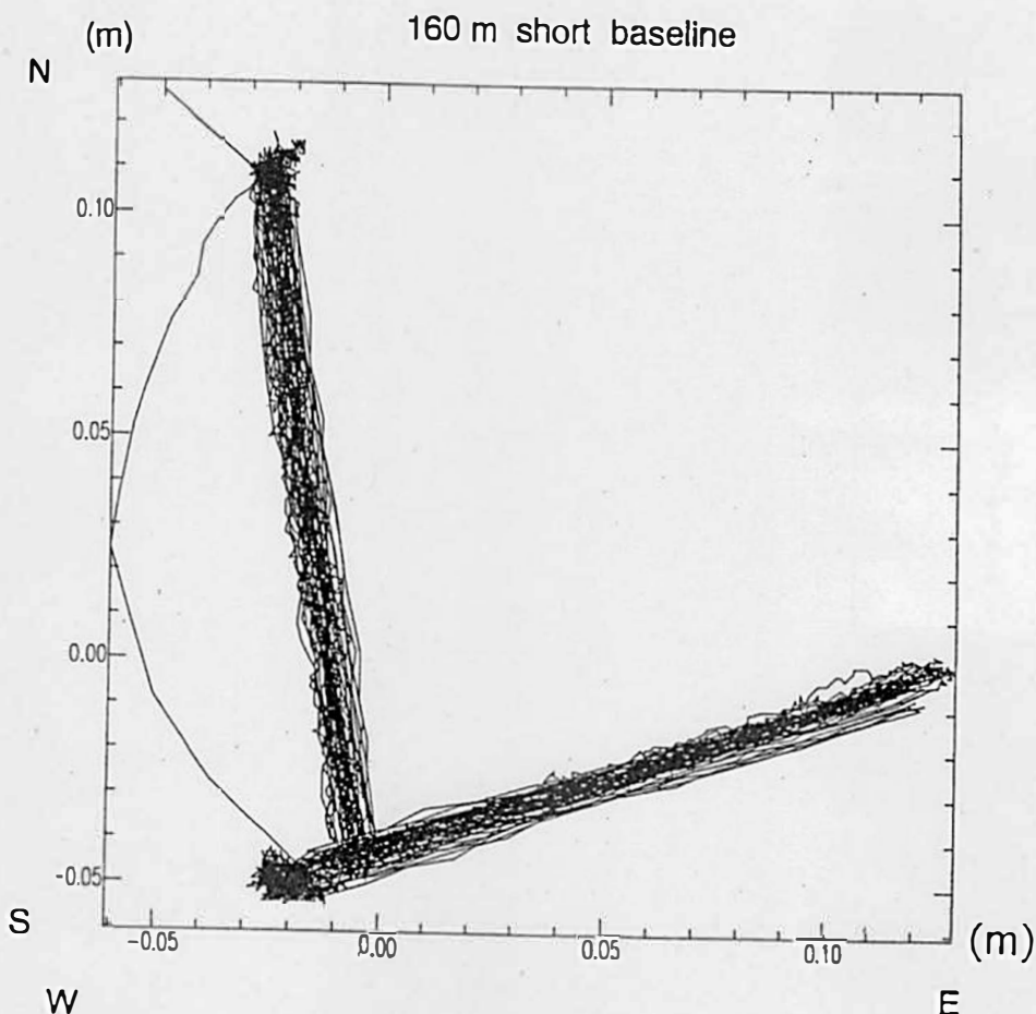
Fig.2 The horizontal motion determined from the base site 160 m apart.
