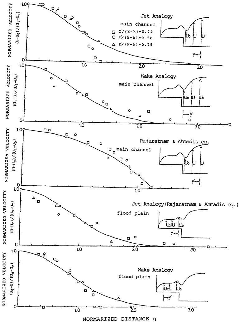
Fig. 9 Lateral distribution of normalized mean velocity.
