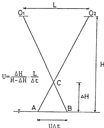
Fig. 1 Cameron effect.
