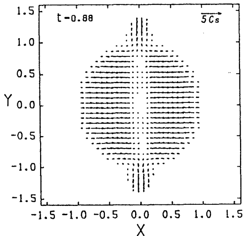
Fig.1. The velocity vectors in the x - y plane at the shock formation stage. Clouds collide along the x -axis with V = 5C_s .
