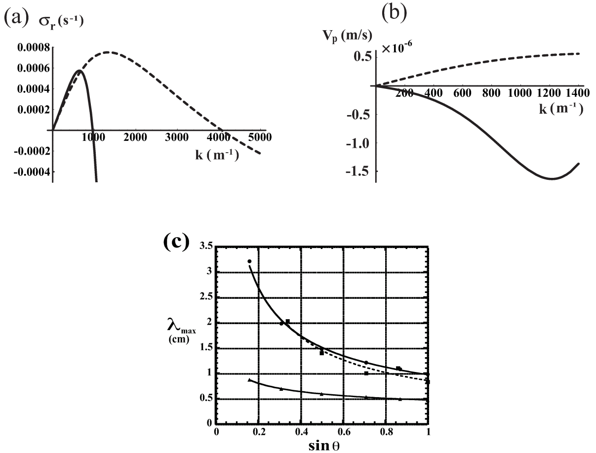
Figure 4. For \bar{V} = 10^{-6} m/s and Q/l = 160(\text{ml/hr})/3\text{cm} , (a) the amplification rate \sigma_r vs the wavenumber k at \theta = \pi/2 . (b) the phase velocity v_p vs the wavenumber k at \theta = \pi/2 . (c) the dependence of wavelength \lambda_{\max} on \sin \theta . Experiment by Matsuda, ■; Ueno's theory, ●; Ogawa and Furukawa's theory, ▲.
