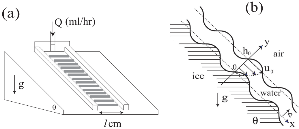
Figure 2. (a) Schematic view of experimental apparatus. Shaded stripes with nearly uniform spacing are protruded part of ripples of ice. (b) Schematic diagram of vertical cross section of the inclined plane. h_0 is the mean thickness of the liquid film and u_0 is the surface fluid velocity.
