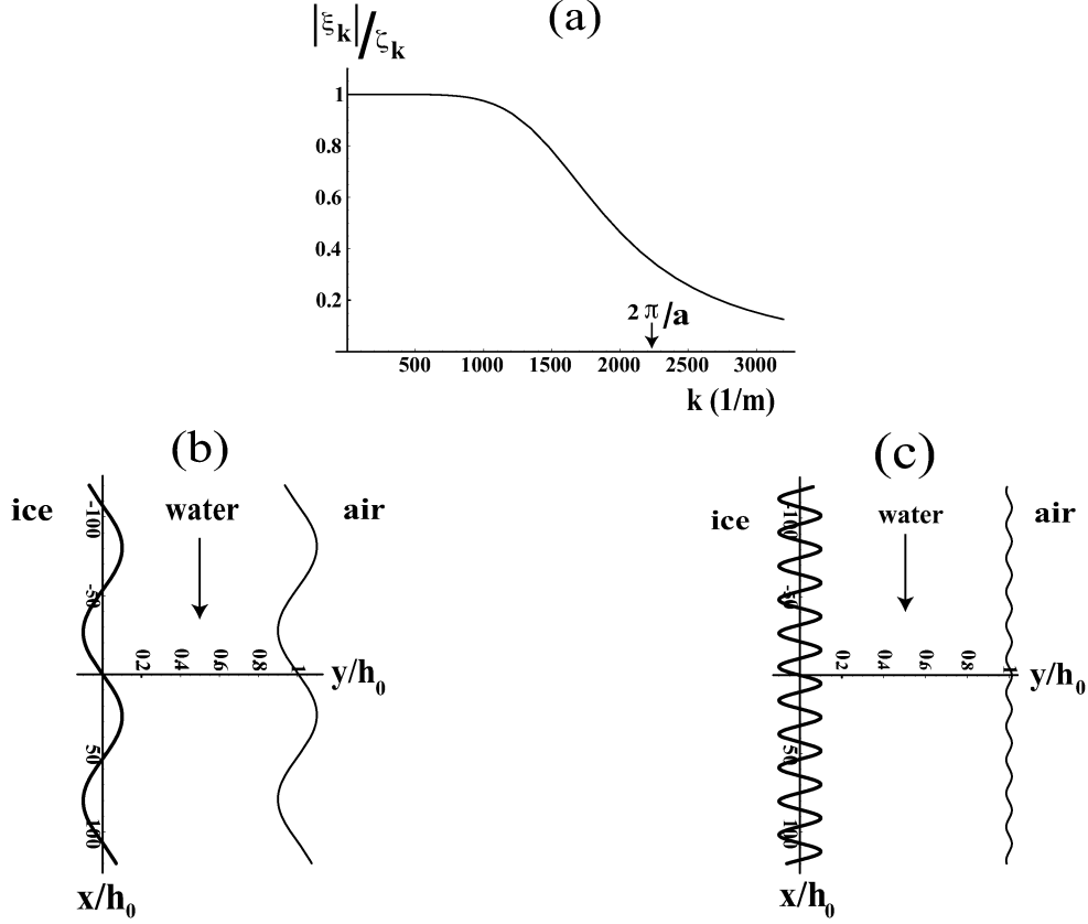
Figure 3. For Q/l = 160(\text{ml/hr})/3\text{cm} and \theta = \pi/2 , (a) the amplitude ratio |\xi_k|/\zeta_k on the wavenumber k . a is the capillary length. The shape of the water-air surface (solid line) for a disturbed ice-water interface (thick solid line) with a amplitude \zeta_k/h_0 = 0.1 when the wavelength of (b) 1 cm ( k \sim 628 \text{ m}^{-1} ) and (c) 2 mm ( k \sim 3142 \text{ m}^{-1} ).
