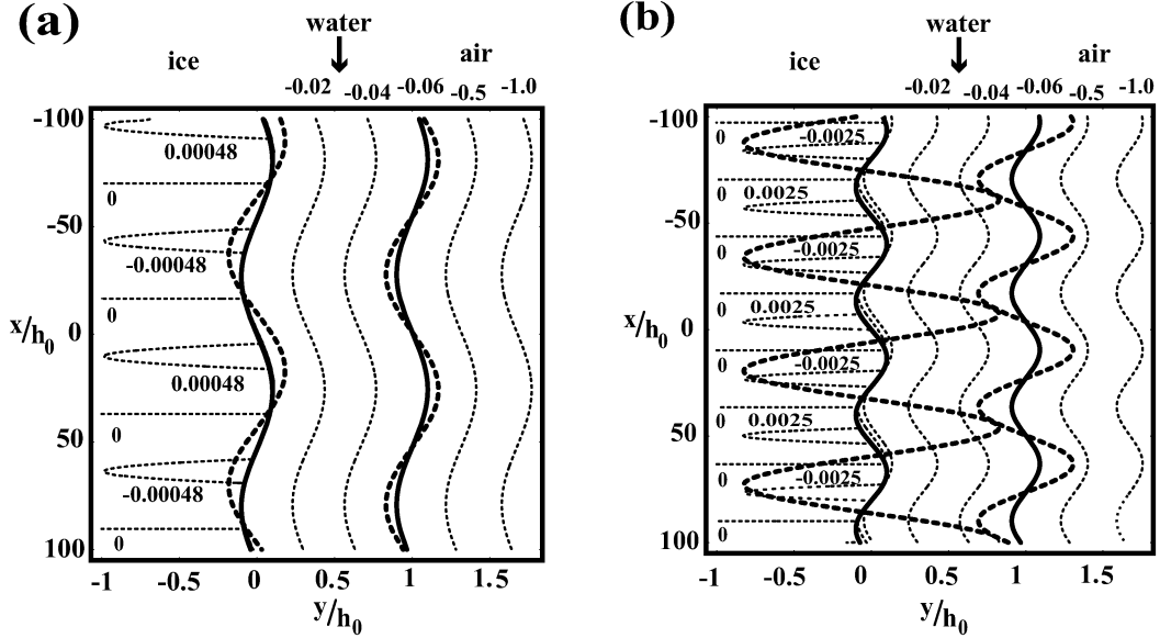
Figure 6. Thick solid lines are the solid-liquid interface \text{Im}[\zeta/h_0] and the liquid-air surface 1 + \text{Im}[\xi/h_0] ; thick dashed lines are distribution of heat flux q_l - q_s at \text{Im}[\zeta/h_0] and distribution of heat flux q_a at 1 + \text{Im}[\xi/h_0] . (a) The wavenumber in the unstable region ( k = 628 \text{ m}^{-1} ). (b) The wavenumber in the stable region ( k = 1256 \text{ m}^{-1} ). Thin dashed lines are isotherm.
