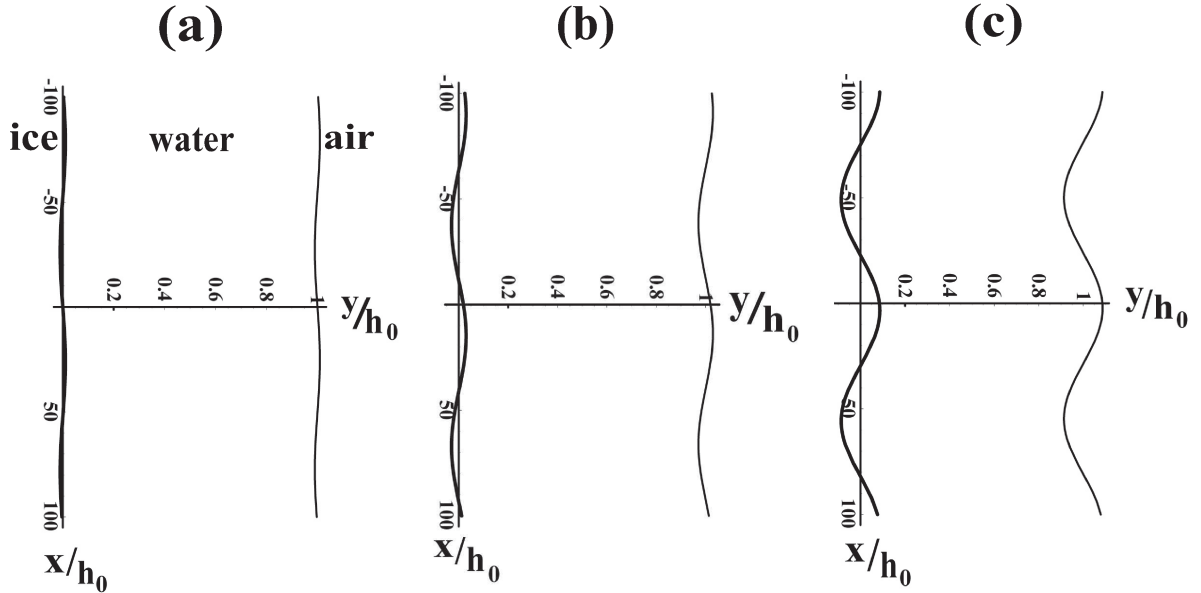
Figure 5. Schematic view of time evolution of the solid-liquid interface. (a) Initial amplitude \zeta_k/h_0 at t = 0 is 0.01. (b) t=0.5 hr. (c) t=1.0 hr.
