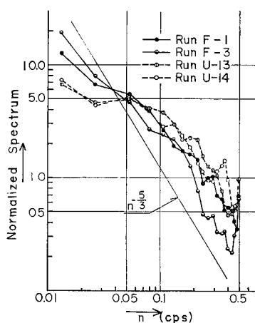
Fig. 4. Spectral density distribution of vertical component of eddy velocity, normalized by the total variance.
