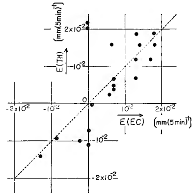
Fig. 7. Comparison between estimated values of evaporation rate by the eddy-correlation method [ E(EC) ], and by the Thorthwaite-Holzman's formula [ E(TH) ].
