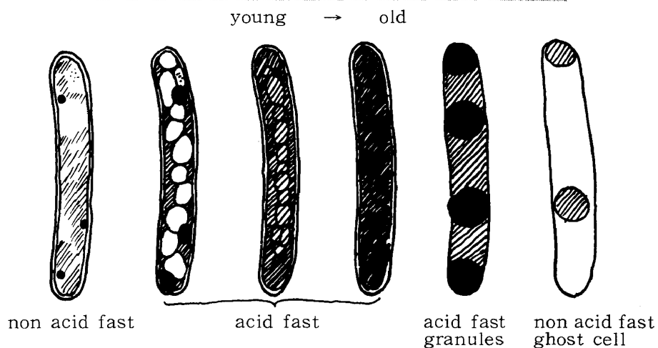
Fig. 7 A schematic diagram showing changes of cell structure of mycobacteria with the lapse of time.
