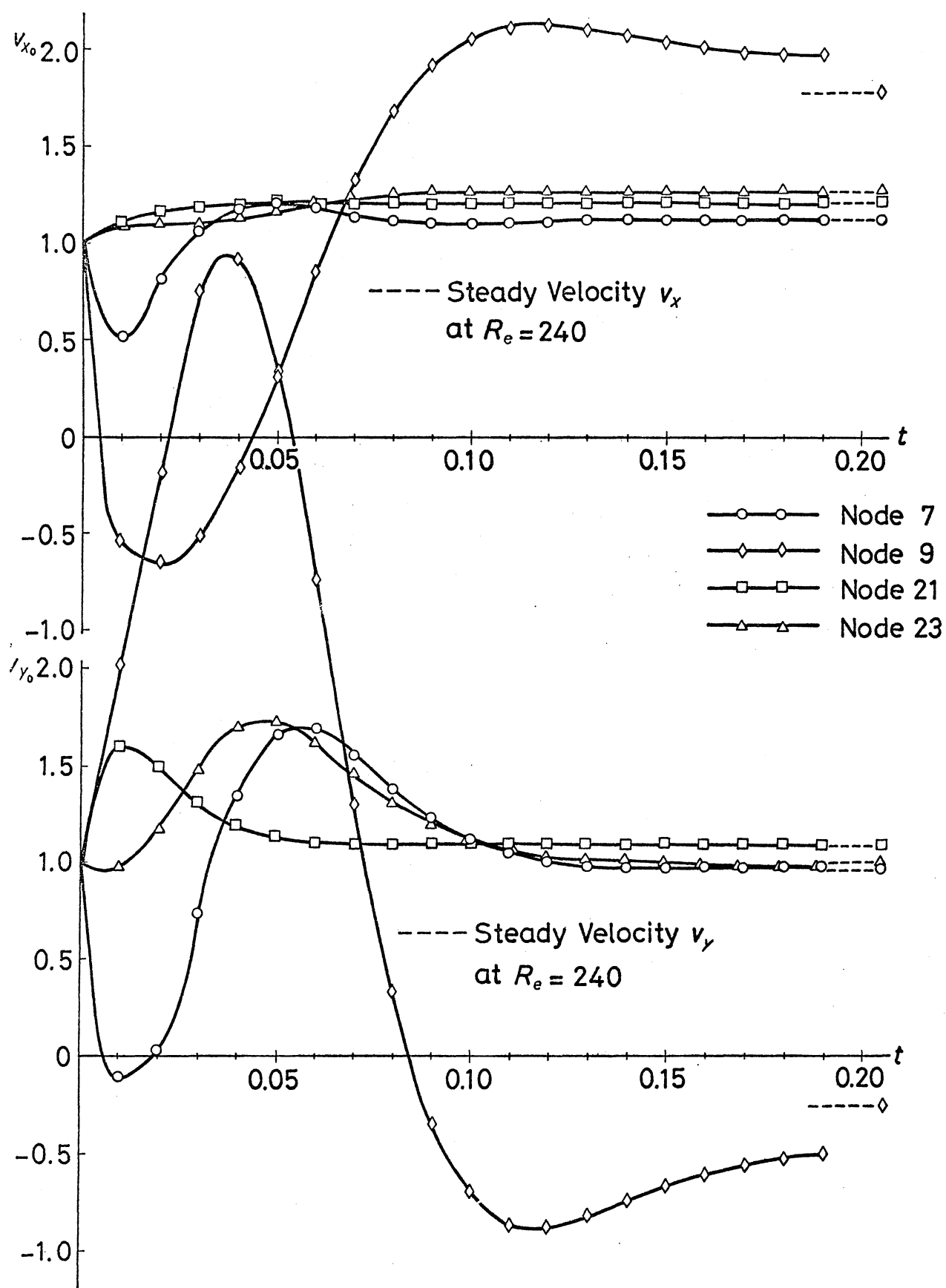
Fig. ( 9 ) Computed Unsteady Velocity from R_e=200 to R_e=240
