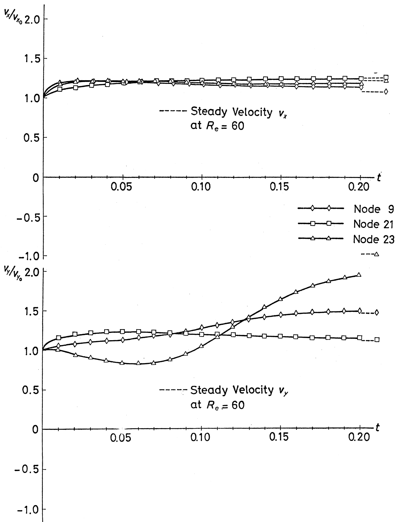
Fig.(6) Computed Unsteady Velocity from R_e = 50 to R_e = 60
