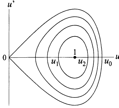
Figure 2: One-parameter family of periodic orbits in (5)
