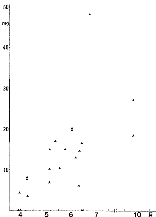
図一1 芦生演習林のスギ樹皮中の試料10g中の \alpha -pinene量(mg)の月変化 Fig. 1. Monthly variation of \alpha -pinene (mg) in the bark of cedar (10g) (Ashu, Kyoto Pref.)
