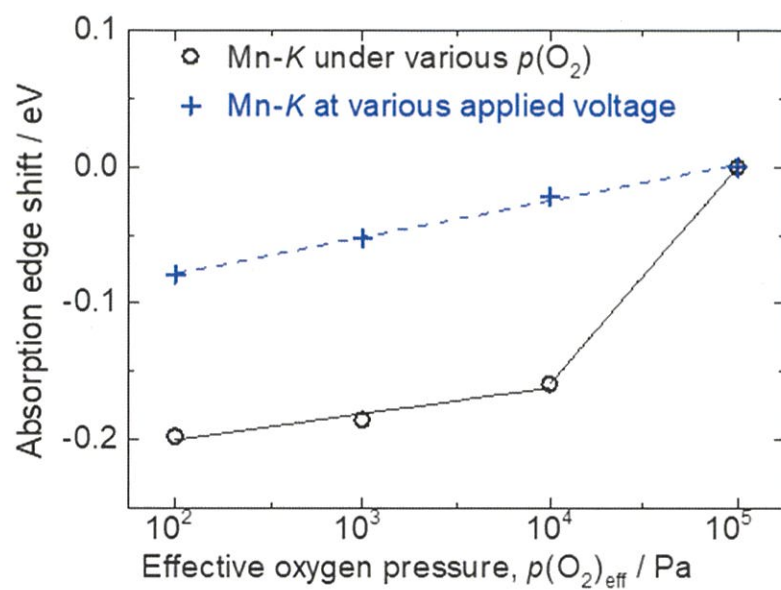
Figure 4.7. Absorption edge shift in Mn K -edge XANES spectrum of LSM as a function of effective oxygen potential at 1073 K. Open circles show the shift measured under various p(\text{O}_2) under open-circuit conditions. Crosses show the shift measured under various applied DC biases at p(\text{O}_2) = 10^5 Pa.
