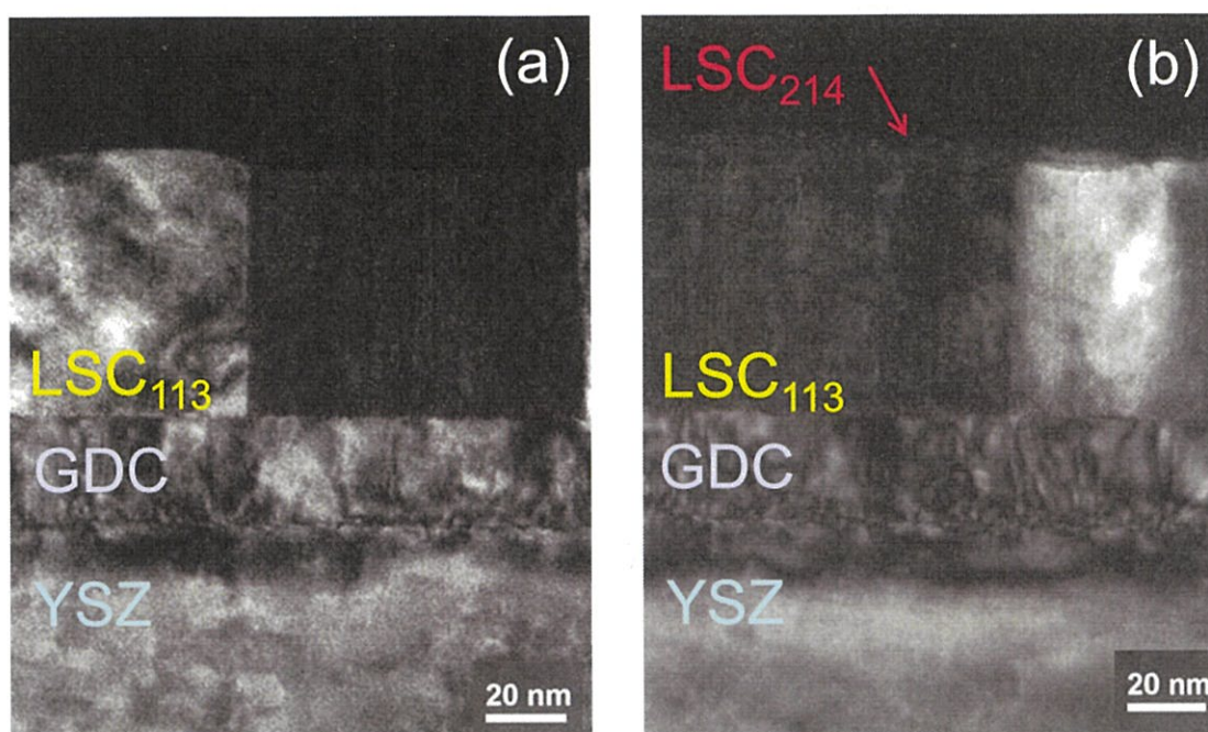
Figure S5.5. Cross-sectional TEM images of (a) \text{LSC}_{113} and (b) \text{LSC}_{113/214} films on YSZ (110). The thickness of each film is \text{LSC}_{113} : 60 nm, GDC: 25 nm and \text{LSC}_{214} : 3 nm. The existence of darkness color in \text{LSC}_{113} layer suggests that the \text{LSC}_{113} films on YSZ (110) single-crystal substrate were polycrystalline phase.
