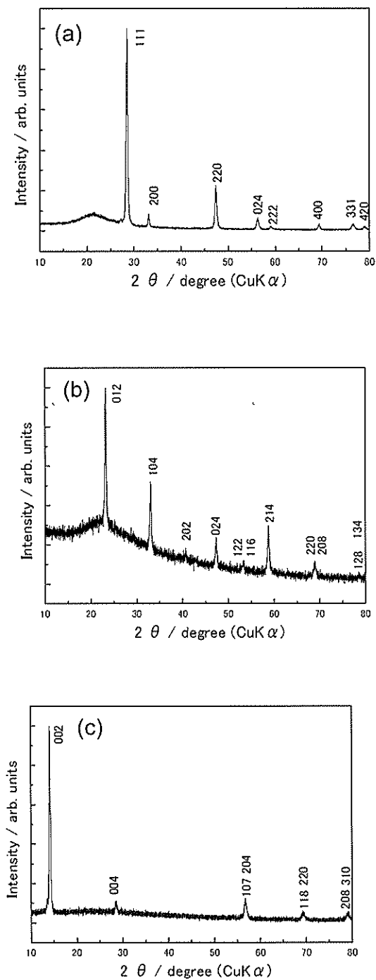
Figure S5.2. XRD patterns of the (a) GDC (gadolinium doped ceria), (b) \text{LSC}_{113} ( \text{La}_{0.6}\text{Sr}_{0.4}\text{CoO}_{3-\delta} ) and (c) \text{LSC}_{214} ( (\text{La}_{0.5}\text{Sr}_{0.5})_2\text{CoO}_{4\pm\delta} ) thin film on the mirror polished silica glass.
