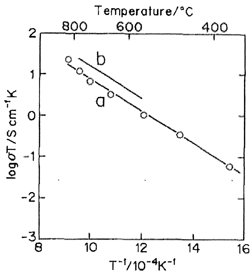
Fig. 3.7. Temperature dependence of conductivity of YSZ films: (a) YSZ thin film prepared by VED method; (b) YSZ (7 mol% \text{Y}_2\text{O}_3 ) by ref. [18].
