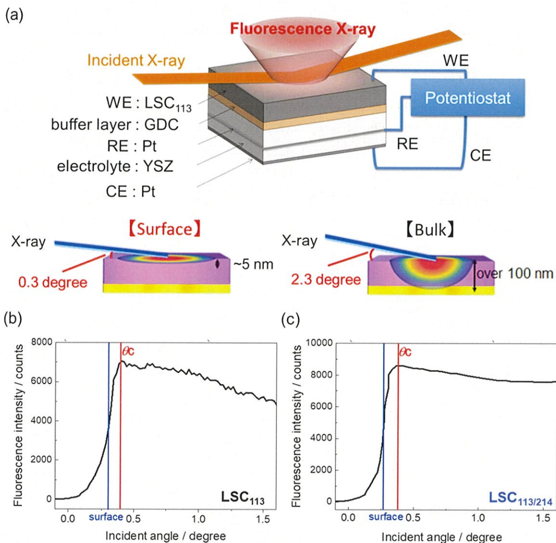
Figure 5.1. (a) Schematic of the setup for data collection in the operando total-reflection XAS cell. Fluorescence counts as a function of incident angle of (b) \text{LSC}_{113} and (c) \text{LSC}_{113/214} . The penetration depth was denoted as “surface” (blue font).
