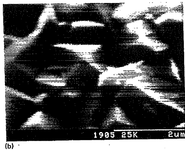
Figure. 2.7. SEM micrograph of (a) fracture cross section and (b) surface of YSZ thin film on CSZ.
