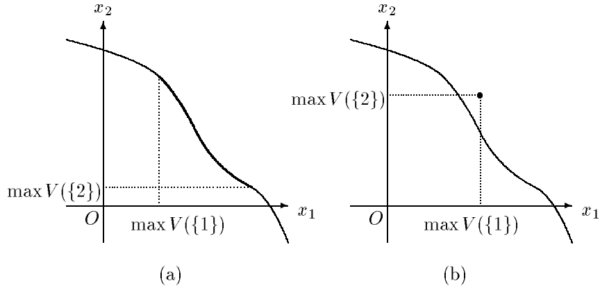
Figure 1: Aspirations for two-agent NTU games: In panel (a), the set of aspirations is indicated by the thick curve. In panel (b), it consists of a single point (\max V(\{1\}), \max V(\{2\})) .
