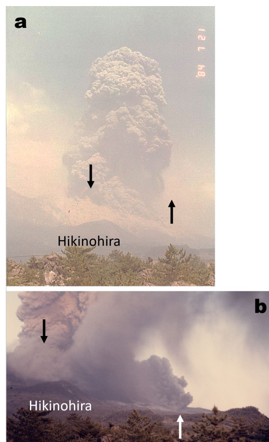
Photo 1 Pyroclastic flow from Minamidake crater. a: 15:02, July 21, 1984. B: 18:27, April 9, 1985. Photographs taken from SVO. Upward and downward arrows indicate front of pyroclastic flows and location of vent-A, respectively.
