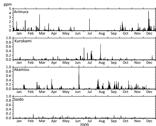
Fig.13 Hourly average of concentration of \text{SO}_2 gas. See Fig. 1 for the locations of monitoring sites.
