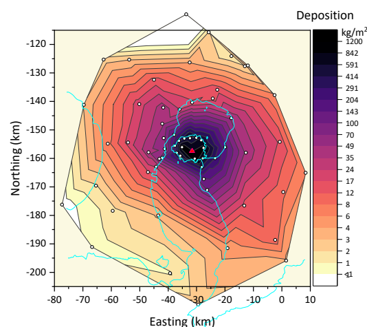
Fig.6 Deposition weight of volcanic ash during the period from August 1978 to December 2020. Circles show sampling sites, managed by Kagoshima Prefecture. The red triangle is the Minamidake crater.
