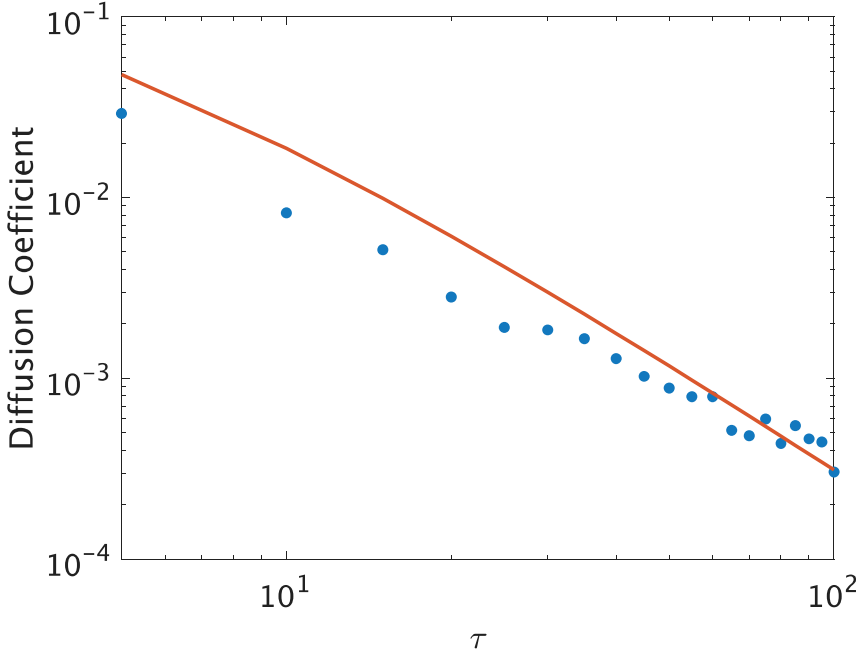
図 2: Diffusion Coefficients for n = 1,000,000 time steps with respect to \tau . K = 0.3 , D = 1.0 , \sigma = 1 . The results are the average of 100 trials.
