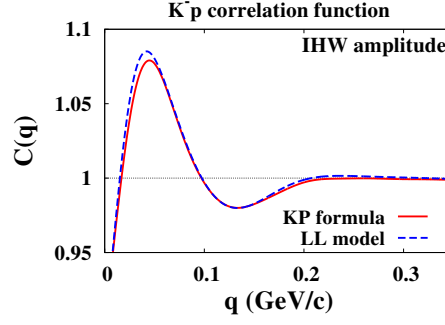
Figure 4: K^-p correlation function obtained with the potential [27], which is fitted to the amplitudes [25]. Solid and dashed lines show the results in KP and LL formulae. The source size is set to be R = 3 fm.
