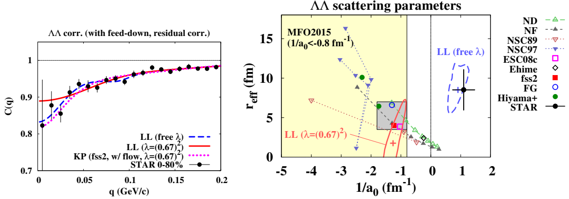
Figure 2: Left: \Lambda \Lambda correlation function obtained by using the LL and KP formulae in comparison with data [14]. Right: Low-energy scattering parameters (a_0, r_{\text{eff}}) of \Lambda \Lambda . Contours show \chi^2/\text{DOF} = 0.65 ( \lambda = (0.67)^2 , solid contour) and \chi^2/\text{DOF} = 0.56 (free \lambda , dashed contour) in the LL model analysis of the correlation data. Symbols show (1/a_0, r_{\text{eff}}) from \Lambda \Lambda potentials [15, 16, 17, 18], and shaded areas show the region favored by the \Lambda \Lambda correlation data in Ref. [2](MFO2015). Filled black circle with xy error bar shows the analysis result by the STAR collaboration, where \lambda is regarded as a free parameter [14].
