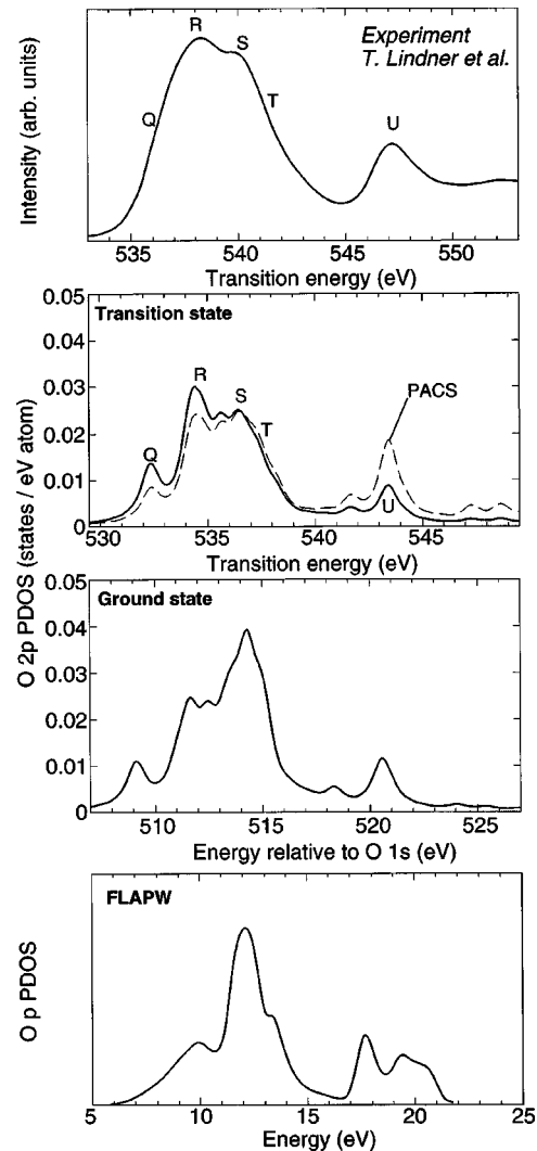
FIG. 3. (From top to bottom) Experimental O K-edge ELNES of MgO by Lindner et al. (Ref. 13). Theoretical O 2p PDOS by a cluster (\text{O}_{63}\text{Mg}_{62})^{2-} calculated for Slater's transition state and for the ground state. O p PDOS by the FLAPW band-structure calculation.
