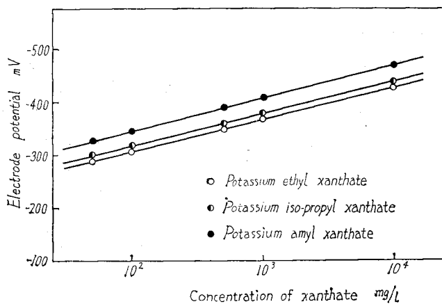
Fig. 8. Electrode potential of mercury in aqueous solution of various xanthates at the concentrations more than 100 mg/l.
