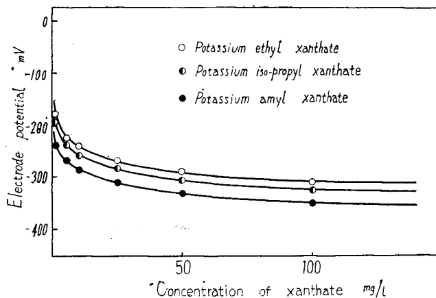
Fig. 6. Electrode potential of mercury in aqueous solutions of various xanthates.
