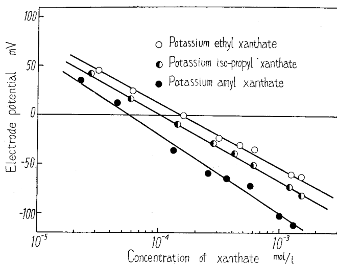
Fig. 9. Electrode potential of pyrite in aqueous solutions of various xanthates.
