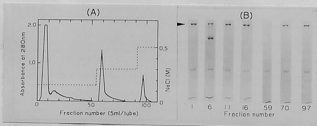
Fig. 10. (A) Elution profile of the Sp-60-MIP from a column (2x10 cm) of DEAE-cellulose. (B) MHC-degrading activity of each fraction determined on SDS-PAGE. Activity was measured at 60°C in the presence of 3 % NaCl. Arrow indicates MHC.
