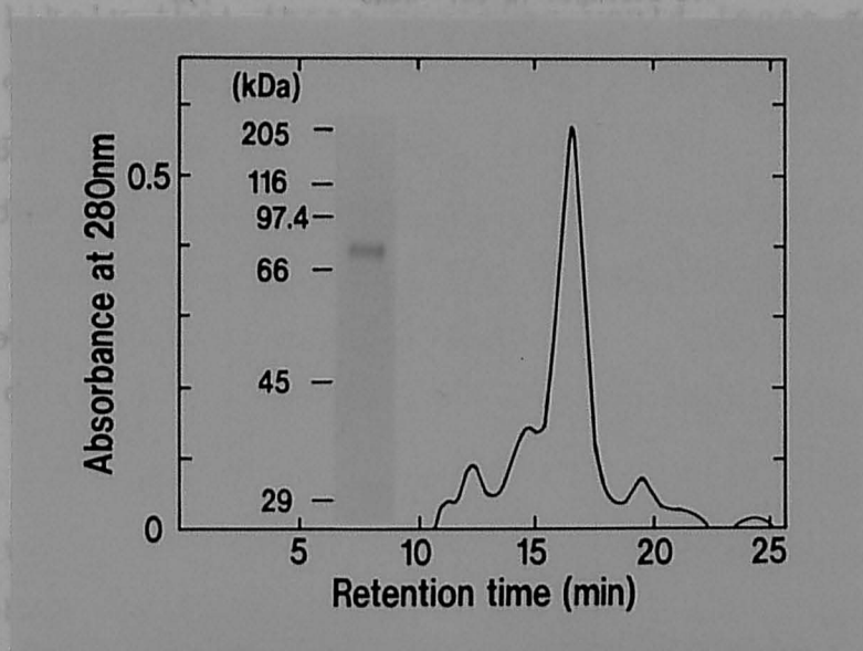
Fig. 19. Elution profile of the Sp-60-MIP from TSK gel G3000SWXL. Inset: 7.5% SDS-PAGE analysis of purified proteinase (retention time 16.5 min)
