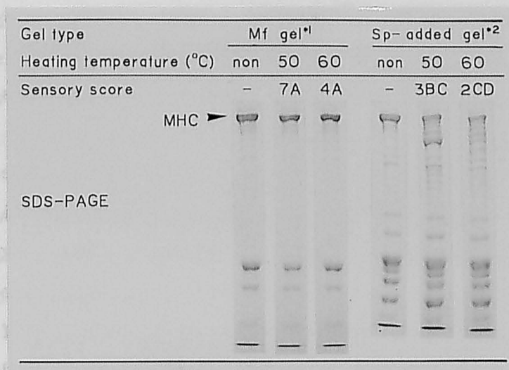
Fig. 24. Classification of modori -inducing proteinases of threadfin bream. Myofibrillar gels and sarcoplasmic fraction added gels were prepared and evaluated as described in "Materials and Methods". Degradation of myosin heavy chain (MHC) was determined by SDS-PAGE. * 1 myofibrillar gel; * 2 sarcoplasmic fraction added gel.
