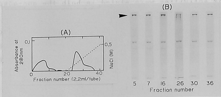
Fig. 12. (A) Elution profile of the Sp-60-MIP from a column (1x3 cm) of Arg-Sephadex. (B) MHC-degrading activity of each fraction determined on SDS-PAGE. Activity was measured at 60°C in the presence of 3 % NaCl. Arrow indicates MHC.
