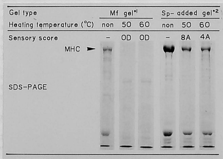
Fig. 26. Classification of modori -inducing proteinases of crucian carp.
