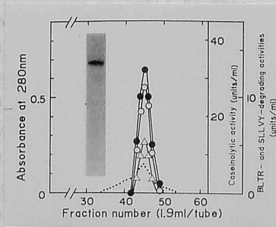
Fig. 1. Elution profile of carp muscle HAP from a column (1.5x100 cm) of Ultrogel AcA 34. Elution was monitored by the absorbance at 280nm(•••). Caseinolytic ( \Delta ), BLTR ( \circ ) and SLLVY ( \bullet )-degrading activities were measured at 65°C. Inset; 5% polyacrylamide gel electrophoresis of the purified proteinase (fraction number 45, 30 \mu g protein) under non-denaturing condition.
