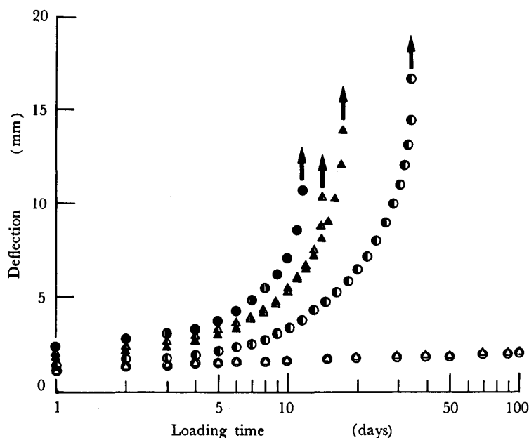
Fig. 2. Deflection-time curves of particleboards in bending-creep tests under progressive fungal attack by Tyromyces palustris .
