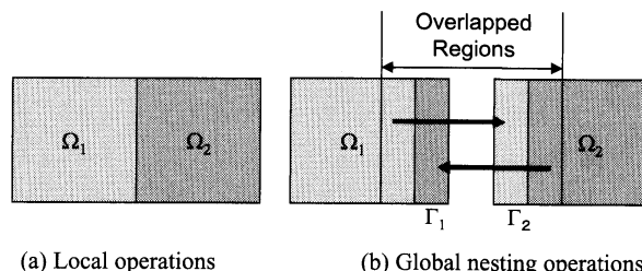
(a) Local operations (b) Global nesting operations 図 6 加法シュワルツ法 (Additive Schwarz Domain Decomposition, ASDD)
