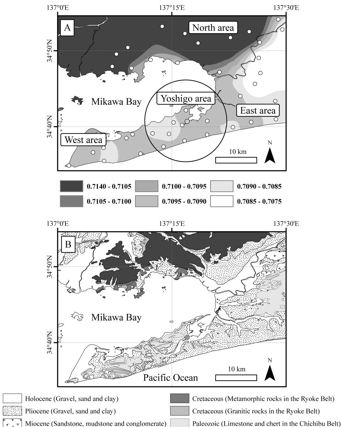
Figure 3: (A) Map of geographic distribution of Sr isotope ratios in plants in study area surrounding Mikawa Bay. Graphic representation is based on ArcGIS (ESRI, Inc.) software through the calculation method of kriging. Open circles are the locations where plant samples were collected. The gray circle is the location of the Yoshigo shell mound. (B) The geological map of the study area was modified from the 1:200,000 geological map “Toyohashi and Irigo Misaki” (Makimoto et al., 2004).
